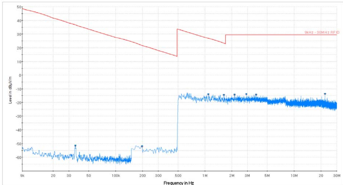
Plot 7-2. Radiated Spurious Plot 9kHz – 30MHz (Pol. Y)
