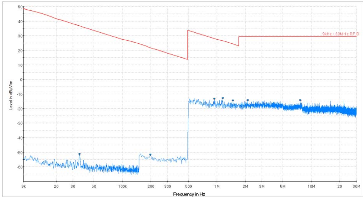
Plot 7-3. Radiated Spurious Plot 9kHz – 30MHz (Pol. Z)
