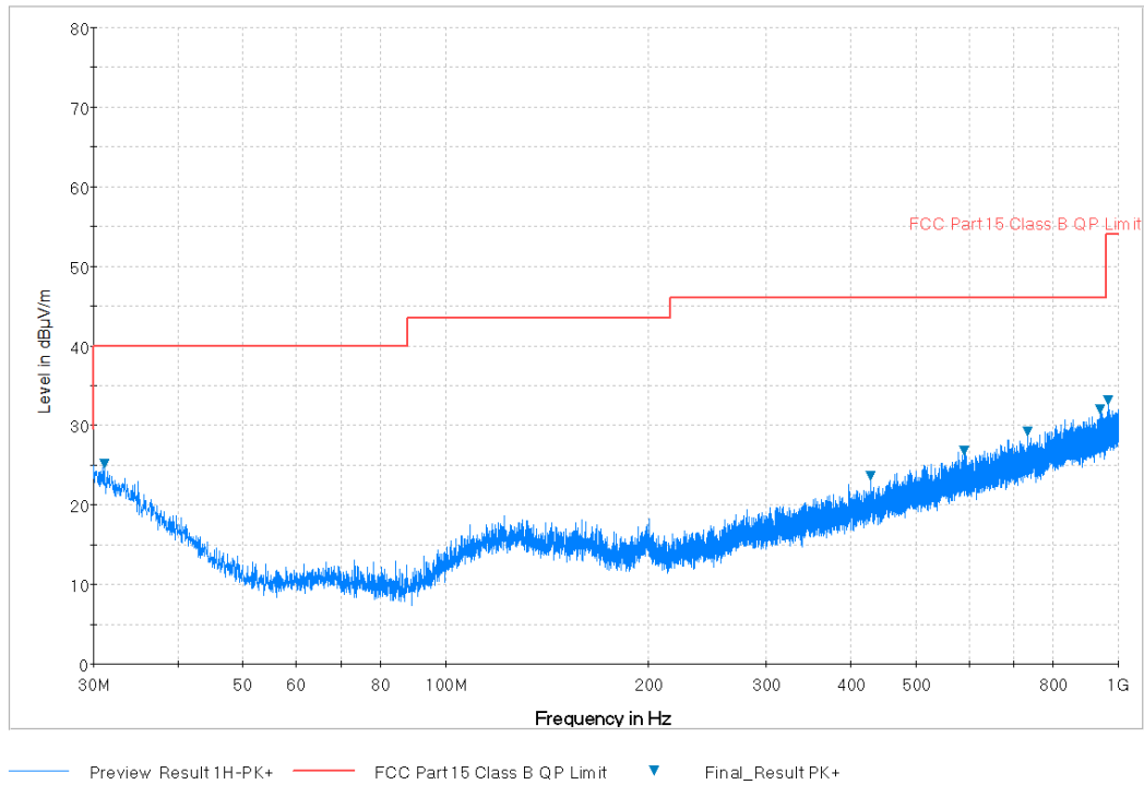
Plot 7-4. Radiated Spurious Plot 30MHz – 1GHz (Pol. H)
