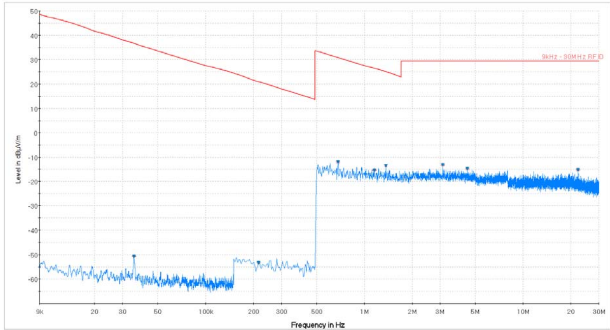
Plot 7-1. Radiated Spurious Plot 9kHz – 30MHz (Pol. X)
