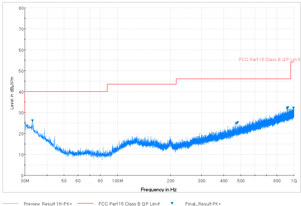
Plot 7-5. Radiated Spurious Plot 30MHz – 1GHz (Pol. V)
