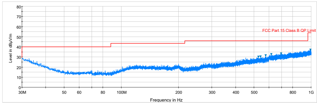
Plot 7-1. Radiated Spurious Plot 30MHz – 1GHz (Pol. H)
