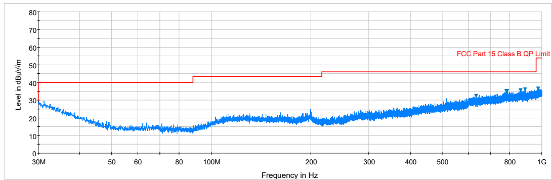
Plot 7-2. Radiated Spurious Plot 30MHz – 1GHz (Pol. V)
