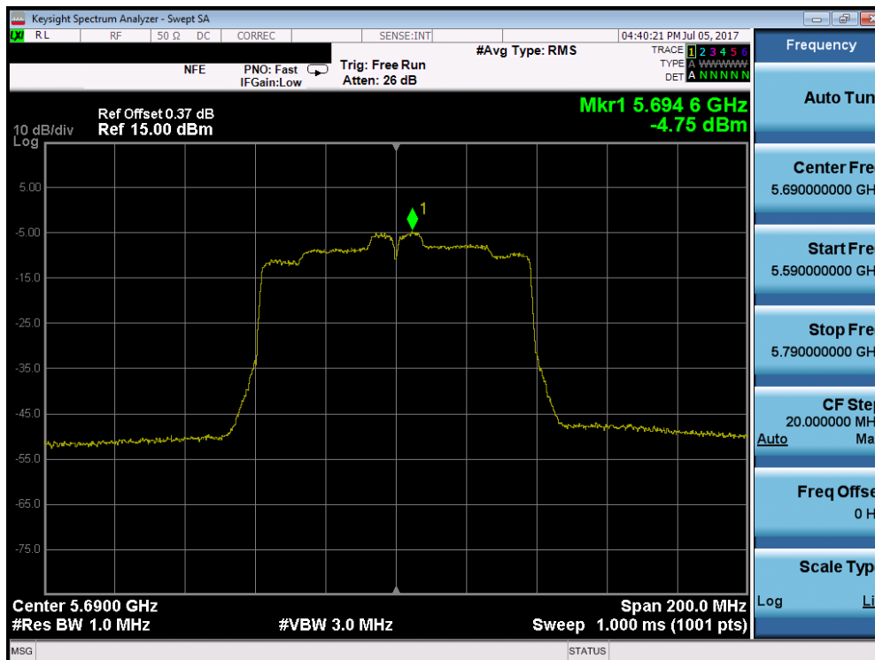
Plot 7-90. Power Spectral Density Plot (80MHz BW 802.11ac (UNII Band 2C) – Ch. 138)
