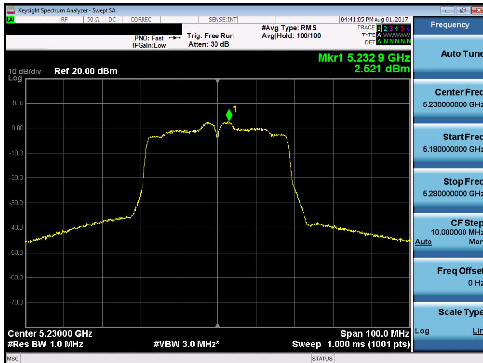
Plot 7-68. Power Spectral Density Plot (40MHz BW 802.11n (UNII Band 1) – Ch. 46)
