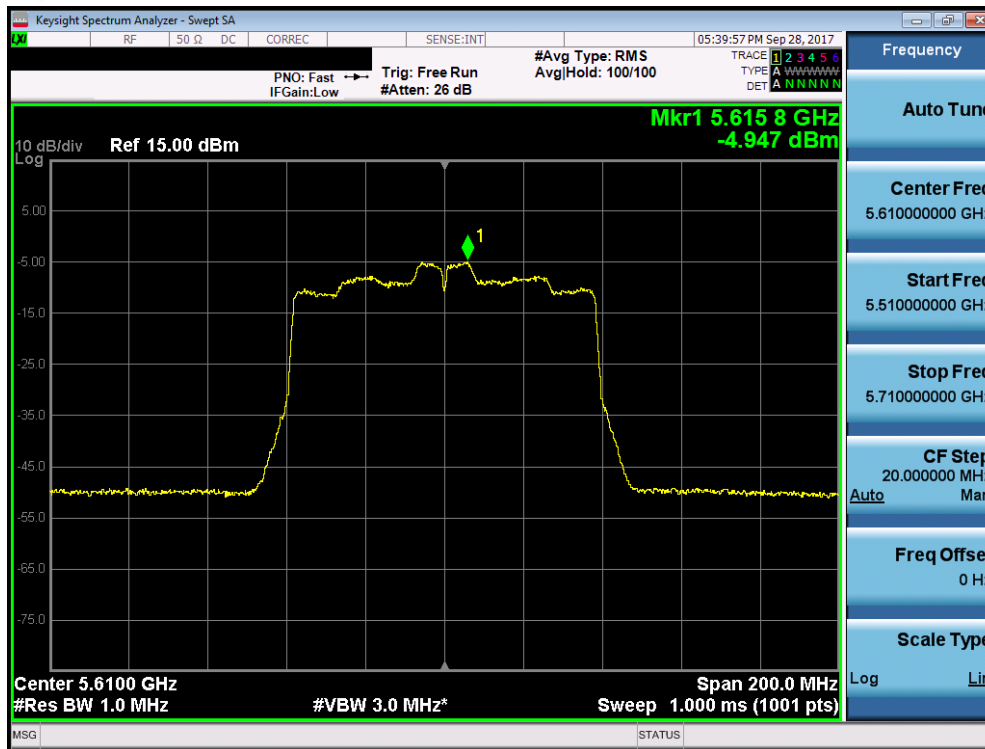
Plot 7-89. Power Spectral Density Plot (80MHz BW 802.11ac (UNII Band 2C) – Ch. 122)
