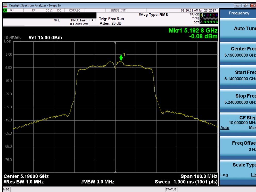
Plot 7-67. Power Spectral Density Plot (40MHz BW 802.11n (UNII Band 1) – Ch. 38)
