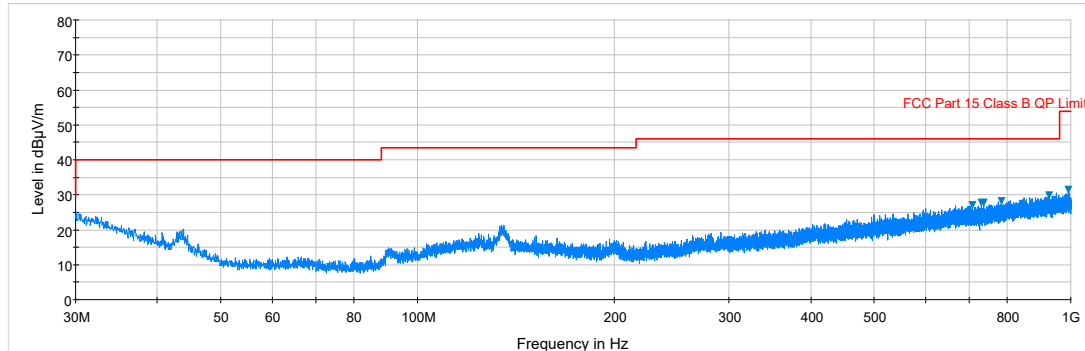
Plot 7-207. Radiated Spurious Plot below 1GHz (2.4GHz – 5GHz, Ant. Pol. H)
