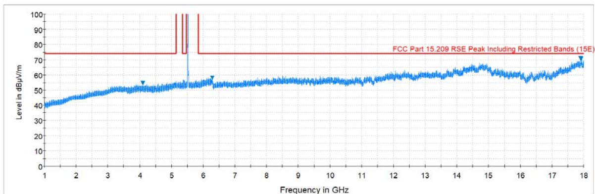
Plot 7-124. Radiated Spurious Plot above 1GHz (802.11a – U2C Ch. 116, Ant. Pol. V)
