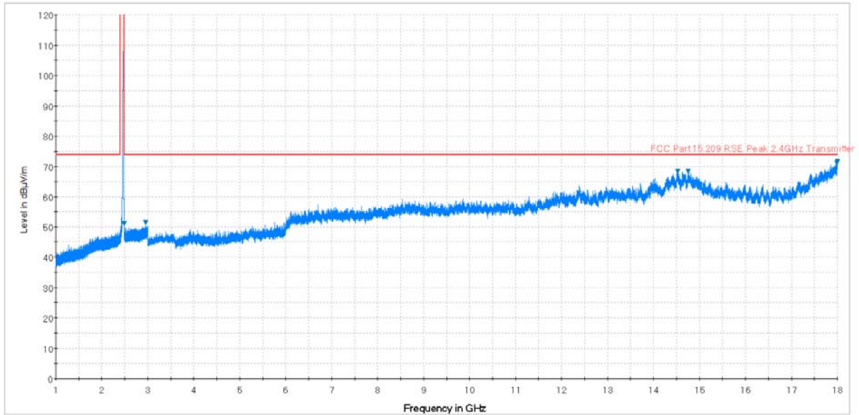
Plot 7-74. Radiated Spurious Plot above 1GHz (802.11b – Ch. 11, Ant. Pol. V)
