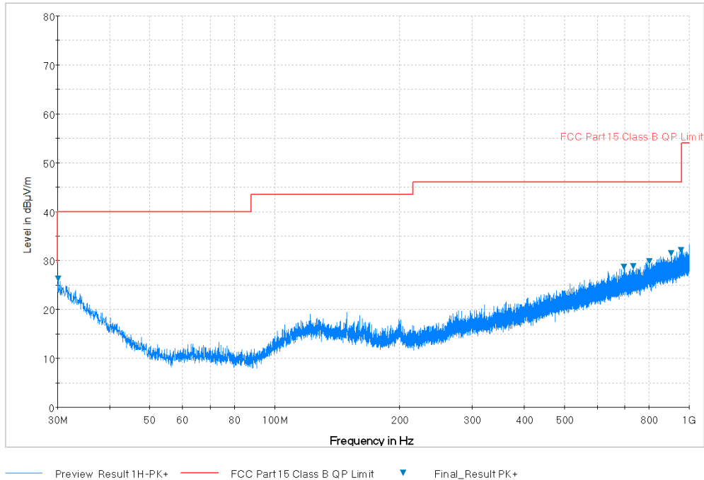
Plot 7-105. Radiated Spurious Plot below 1GHz (Pol. H)
