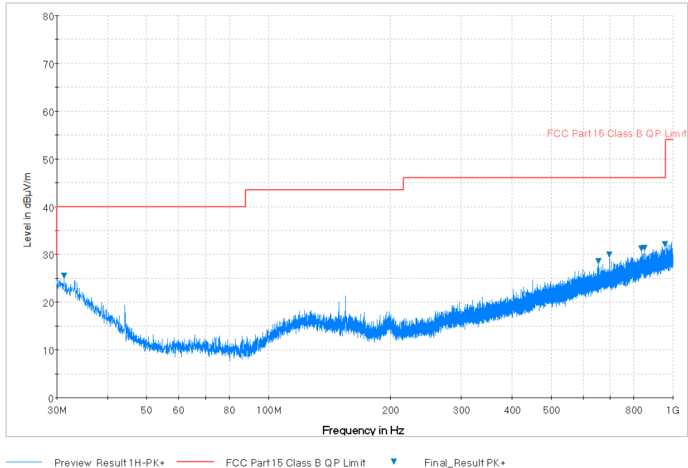
Plot 7-106. Radiated Spurious Plot below 1GHz (Pol. V)
