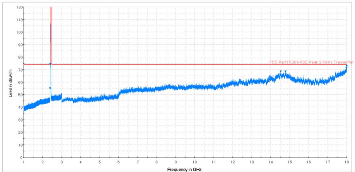
Plot 7-69. Radiated Spurious Plot above 1GHz (802.11b – Ch. 1, Ant. Pol. H)
