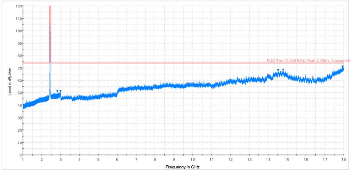
Plot 7-71. Radiated Spurious Plot above 1GHz (802.11b – Ch. 6, Ant. Pol. H)
