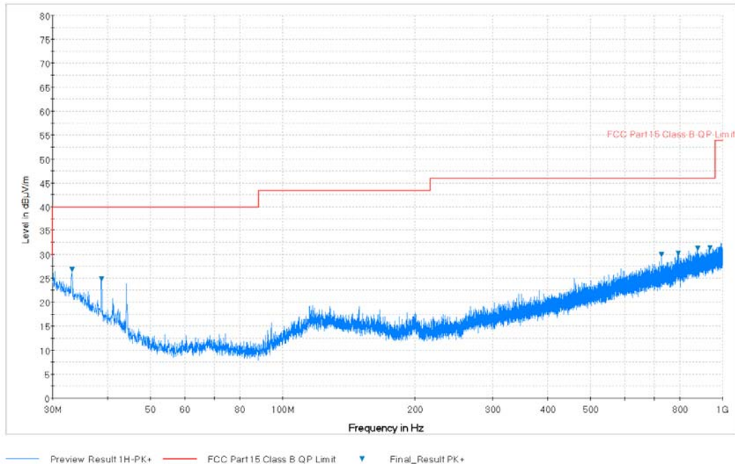
Plot 7-108. Radiated Spurious Plot below 1GHz (Pol. V)
