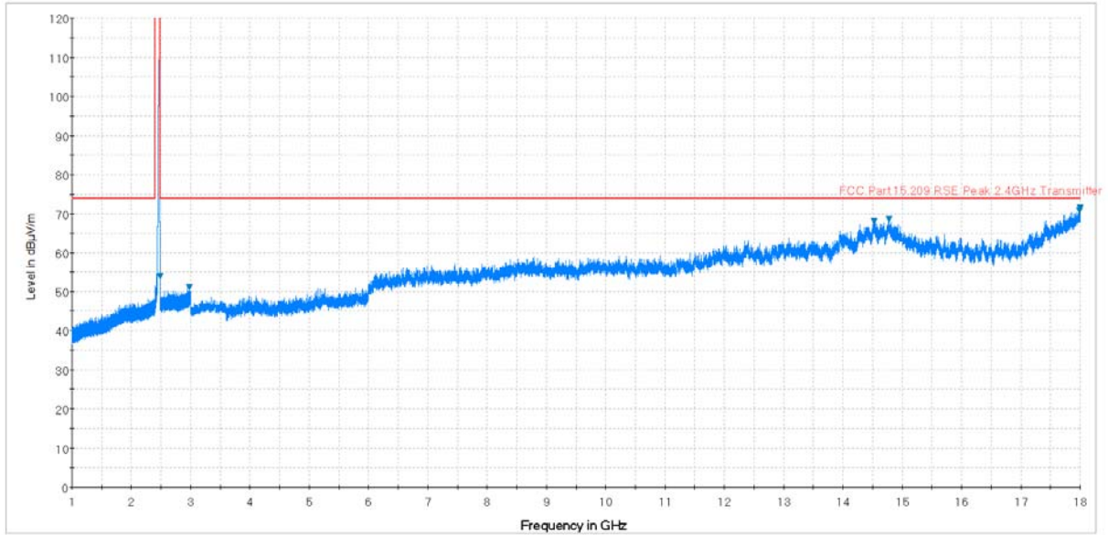
Plot 7-73. Radiated Spurious Plot above 1GHz (802.11b – Ch. 11, Ant. Pol. H)
