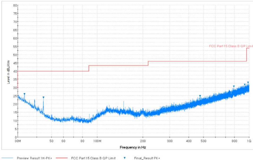
Plot 7-107. Radiated Spurious Plot below 1GHz (Pol. H)
