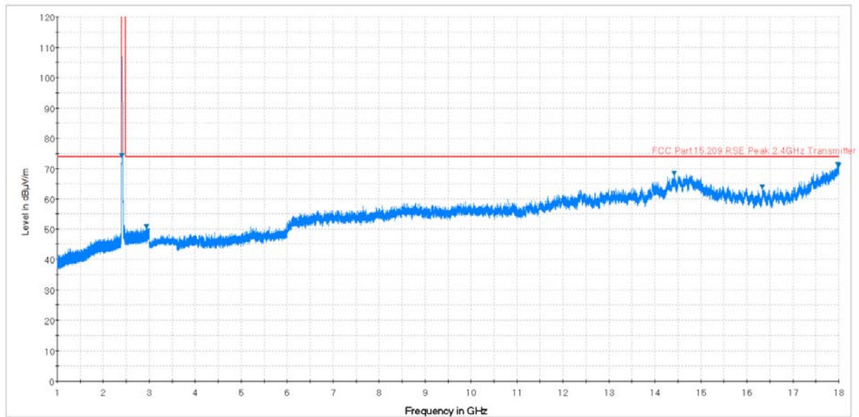
Plot 7-61. Radiated Spurious Plot above 1GHz (802.11b – Ch. 1, Ant. Pol. H)
