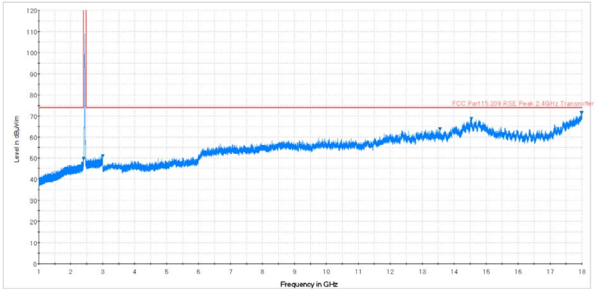
Plot 7-72. Radiated Spurious Plot above 1GHz (802.11b – Ch. 6, Ant. Pol. V)
