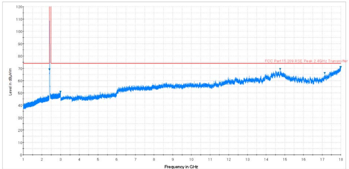
Plot 7-70. Radiated Spurious Plot above 1GHz (802.11b – Ch. 1, Ant. Pol. V)
