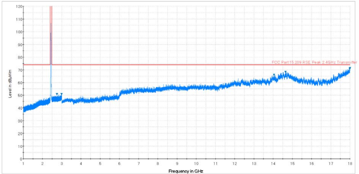
Plot 7-64. Radiated Spurious Plot above 1GHz (802.11b – Ch. 6, Ant. Pol. V)
