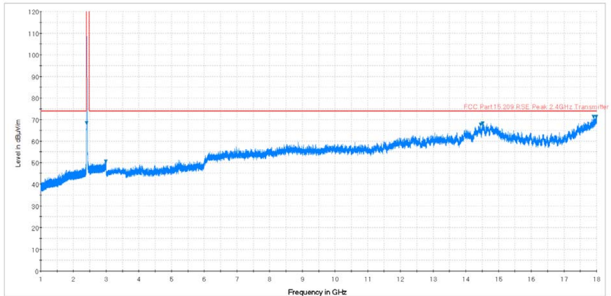
Plot 7-62. Radiated Spurious Plot above 1GHz (802.11b – Ch. 1, Ant. Pol. V)
