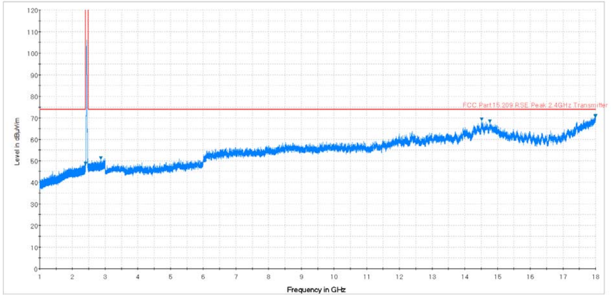
Plot 7-63. Radiated Spurious Plot above 1GHz (802.11b – Ch. 6, Ant. Pol. H)
