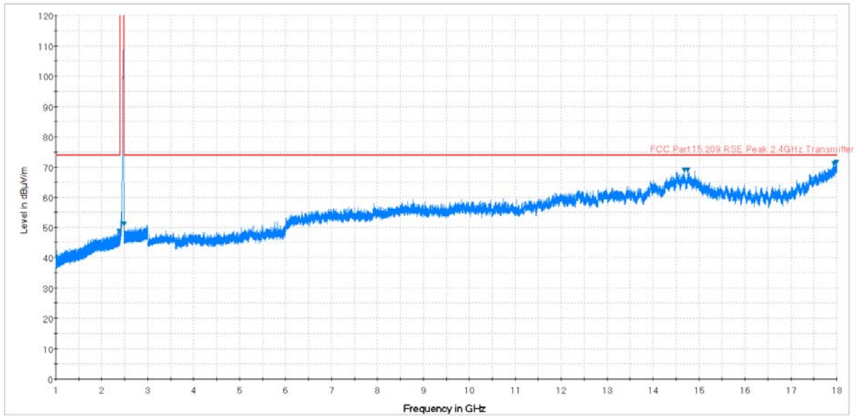
Plot 7-65. Radiated Spurious Plot above 1GHz (802.11b – Ch. 11, Ant. Pol. H)
