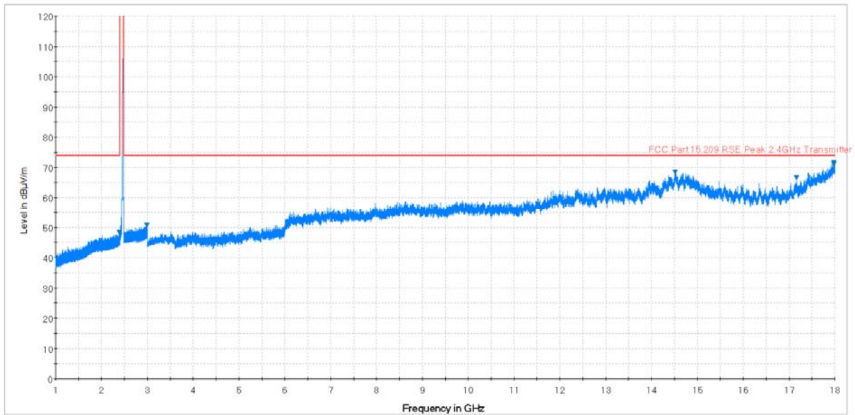
Plot 7-66. Radiated Spurious Plot above 1GHz (802.11b – Ch. 11, Ant. Pol. V)
