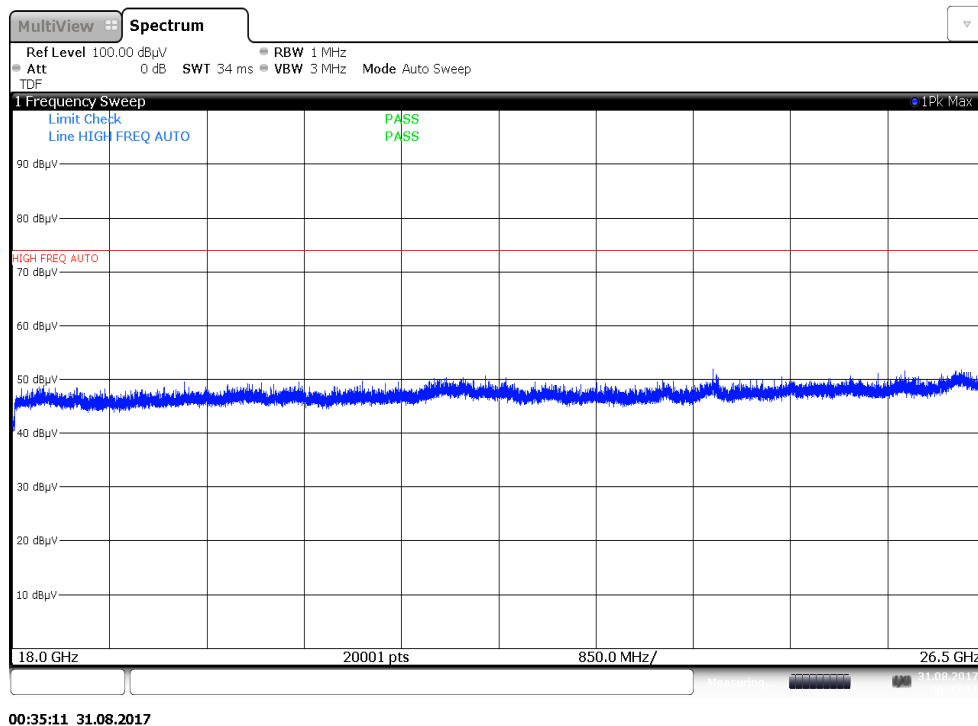
Plot 7-28. Radiated Spurious Plot above 18GHz (Pol. V)
