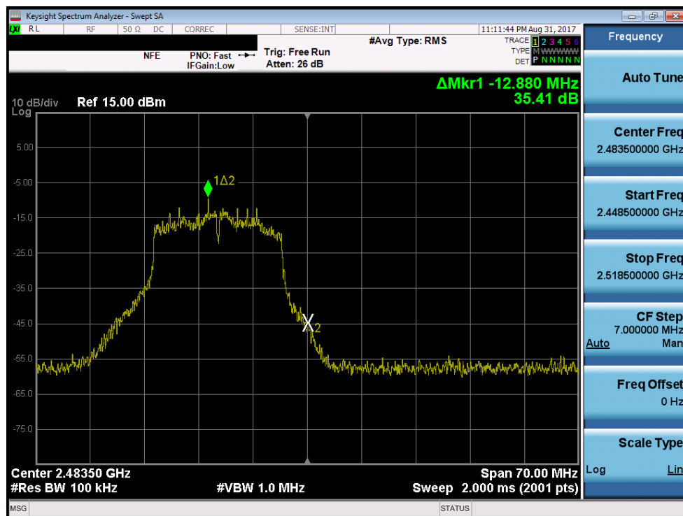
Plot 7-10. Band Edge Plot (802.11g – Ch. 13)
