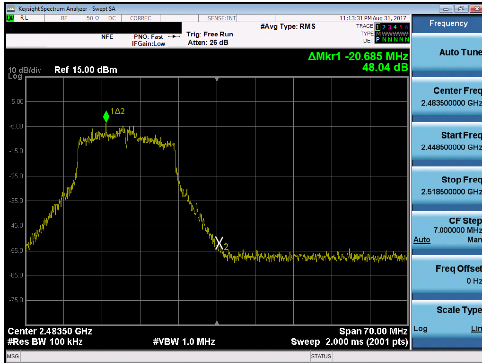
Plot 7-11. Band Edge Plot (802.11n – Ch. 12)
