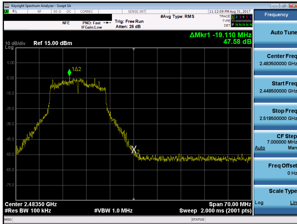
Plot 7-9. Band Edge Plot (802.11g – Ch. 12)
