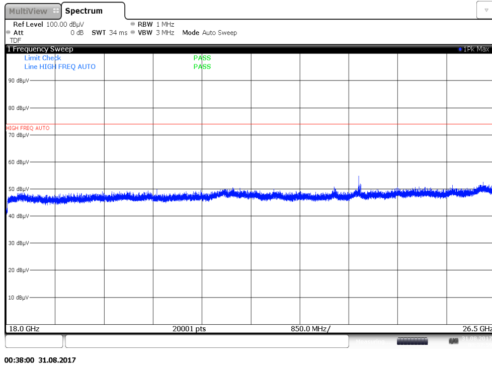
Plot 7-27. Radiated Spurious Plot above 18GHz (Pol. H)
