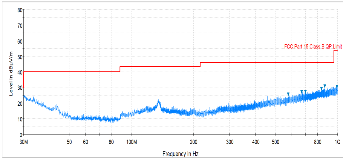
Plot 7-46. Radiated Spurious Plot below 1GHz (Pol. H)
