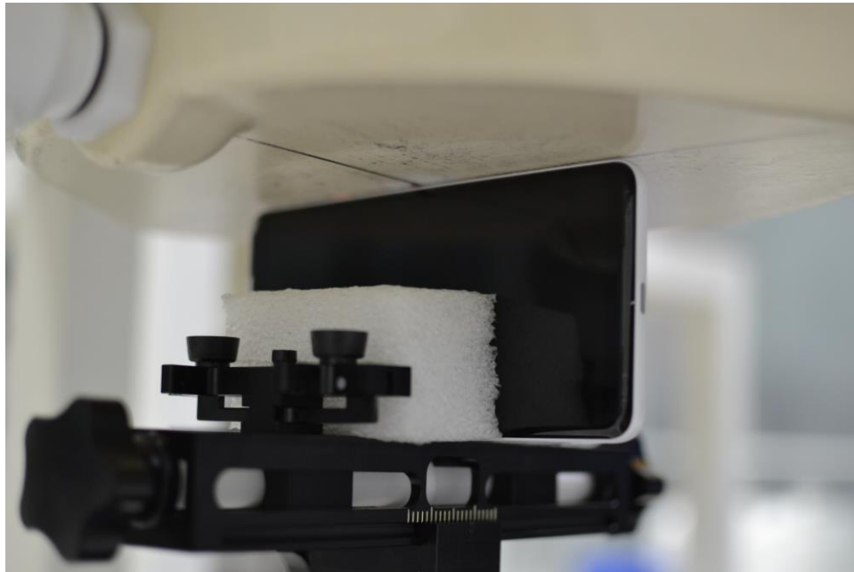
SAR Test Setup Photo 13: Right at 0.0 cm
