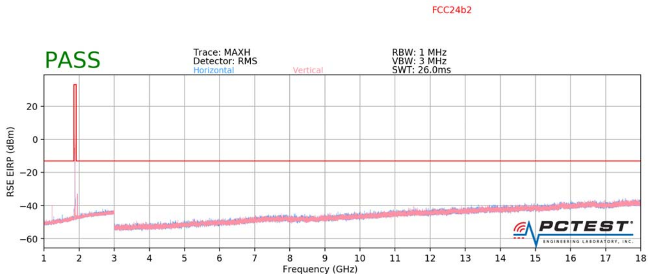
Plot 7-4. Radiated Spurious Plot (PCS GSM Mode)
