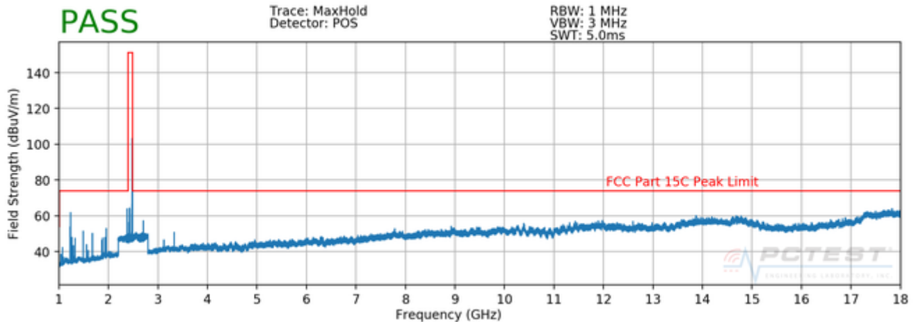
Plot 7-44. Radiated Spurious Plot above 1GHz (BT – Ch. 78, Pol. H)
