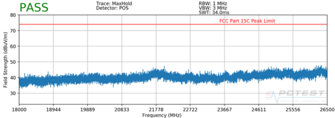
Plot 7-45. Radiated Spurious Plot above 18GHz (BT – Ch. 39, Pol. H)
