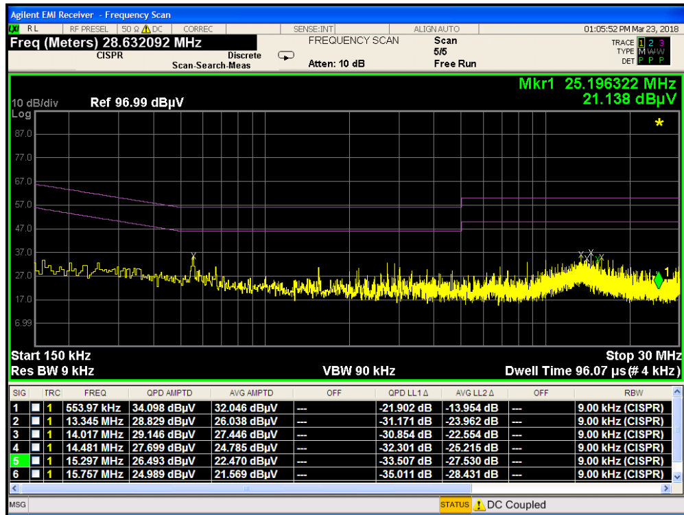
Plot 7-54. Line-Conducted Test Plot (L1) with WCP
