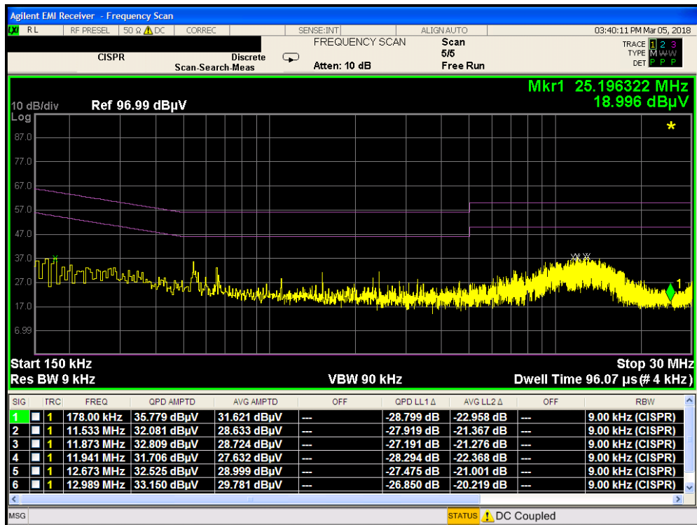
Plot 7-53. Line-Conducted Test Plot (N)
