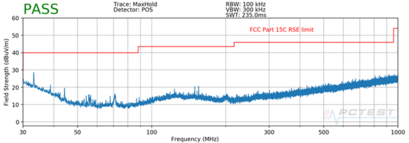
Plot 7-51. Radiated Spurious Plot below 1GHz (Pol. V)
