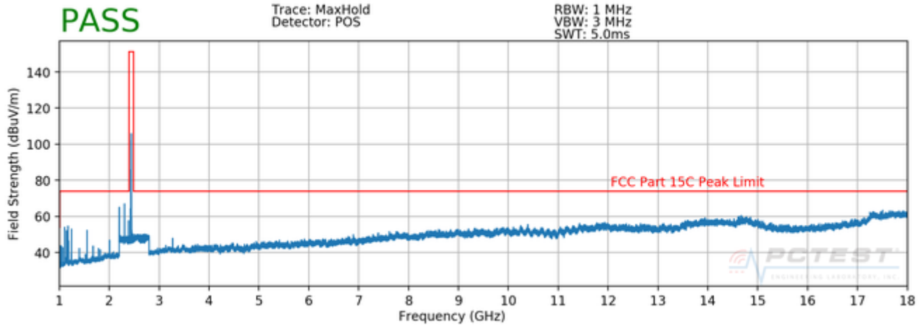
Plot 7-43. Radiated Spurious Plot above 1GHz (BT – Ch. 39, Pol. H)
