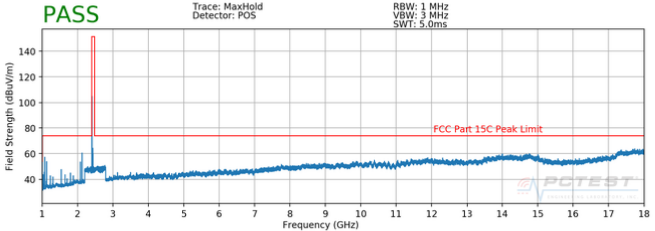
Plot 7-42. Radiated Spurious Plot above 1GHz (BT – Ch. 0, Pol. H)
