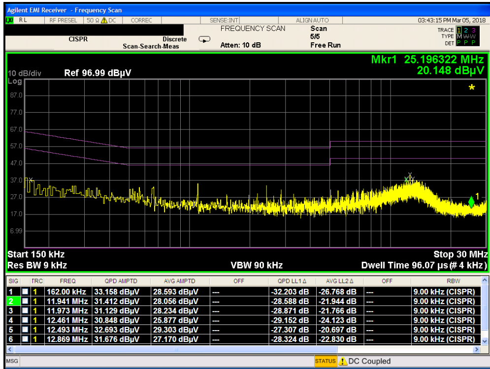
Plot 7-52. Line-Conducted Test Plot (L1)
