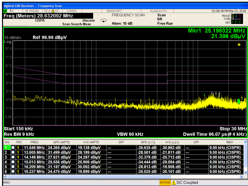
Plot 7-55. Line-Conducted Test Plot (N) with WCP
