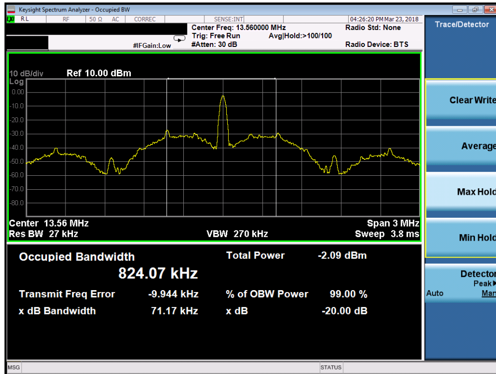
Figure 7-2. 20dB Bandwidth Plot
