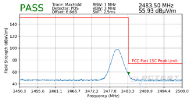
Plot 7-8. Radiated Restricted Upper Band Edge Measurement with WCP (Peak)
