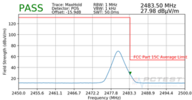
Plot 7-7. Radiated Restricted Upper Band Edge Measurement with WCP (Average)
