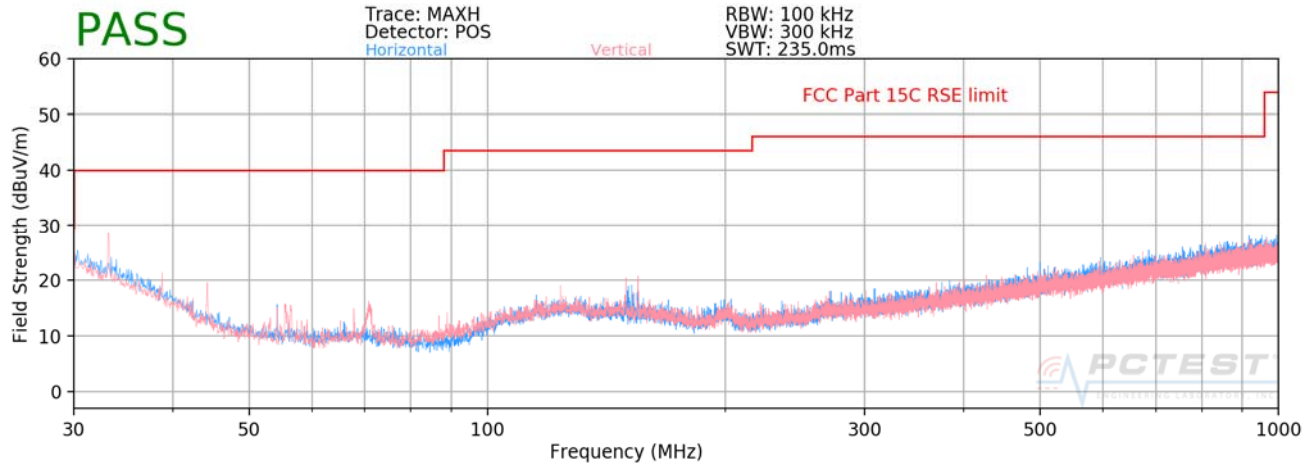
Plot 7-9. Radiated Spurious Plot below 1GHz GFSK ePA
