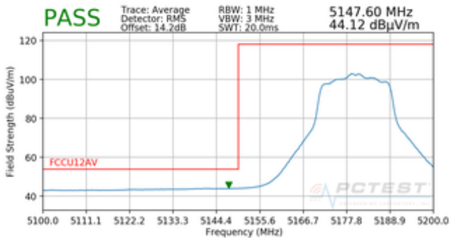
Plot 7-79. Radiated Lower Band Edge Plot (Average – UNII Band 1)
