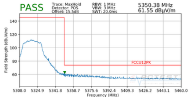
Plot 7-46. Radiated Upper Band Edge Plot (Peak – UNII Band 2A)
