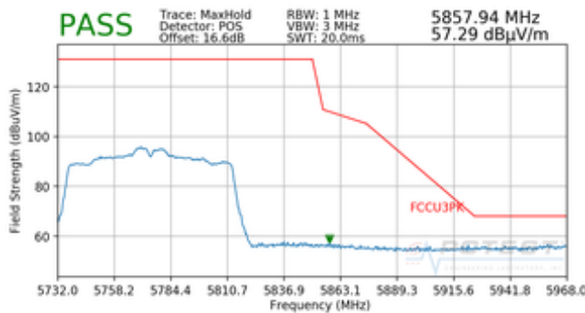
Plot 7-40. Radiated Upper Band Edge Plot (Peak – UNII Band 3)
