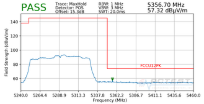
Plot 7-42. Radiated Band Edge Plot (Peak – WCP)
