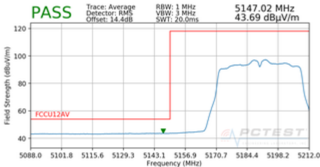
Plot 7-88. Radiated Lower Band Edge Plot (Average – UNII Band 1)
