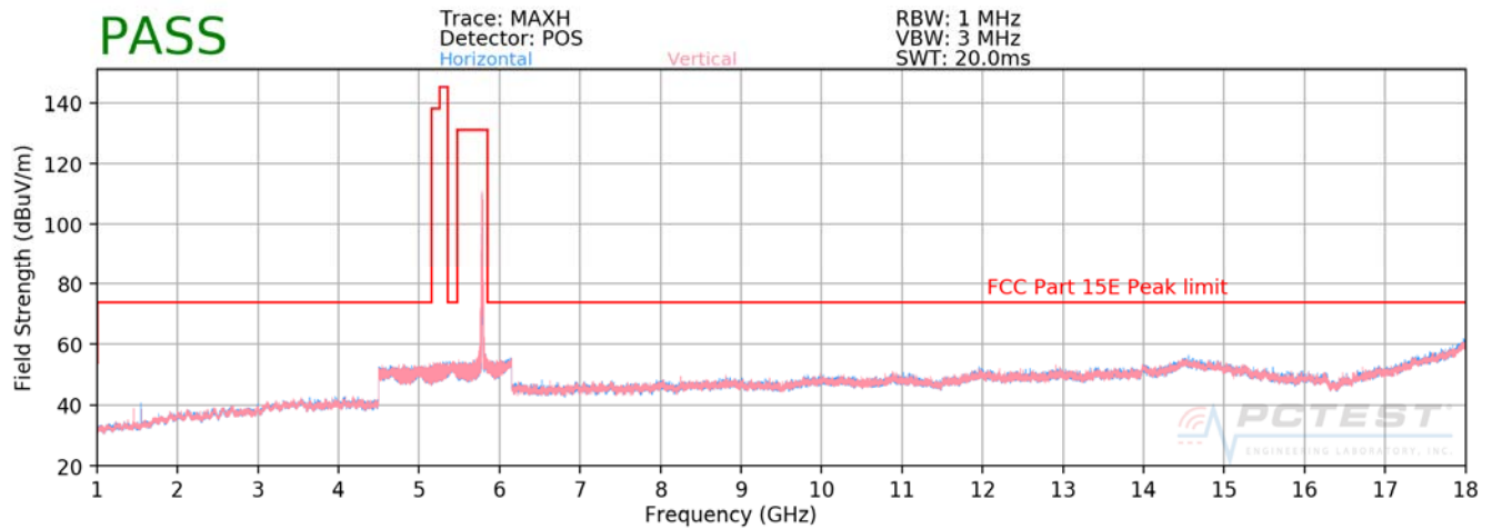
Plot 7-10. Radiated Spurious Plot above 1GHz (802.11a – U3 Ch. 157)
