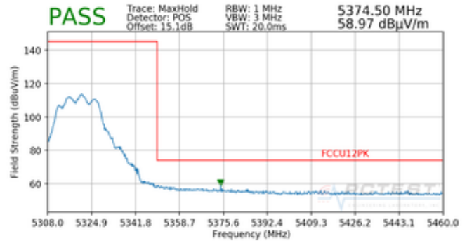
Plot 7-78. Radiated Band Edge Plot (Peak – WCP)
