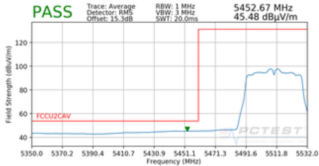
Plot 7-92. Radiated Lower Band Edge Plot (Average – UNII Band 2C)
