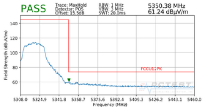
Plot 7-82. Radiated Upper Band Edge Plot (Peak – UNII Band 2A)
