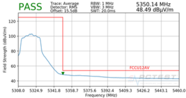
Plot 7-86. Radiated Band Edge Plot (Average – WCP)
