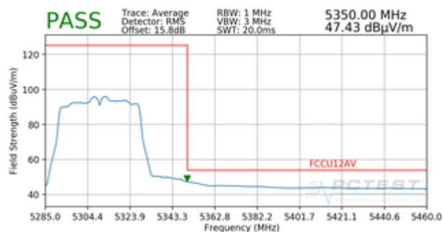
Plot 7-95. Radiated Band Edge Plot (Average – WCP)
