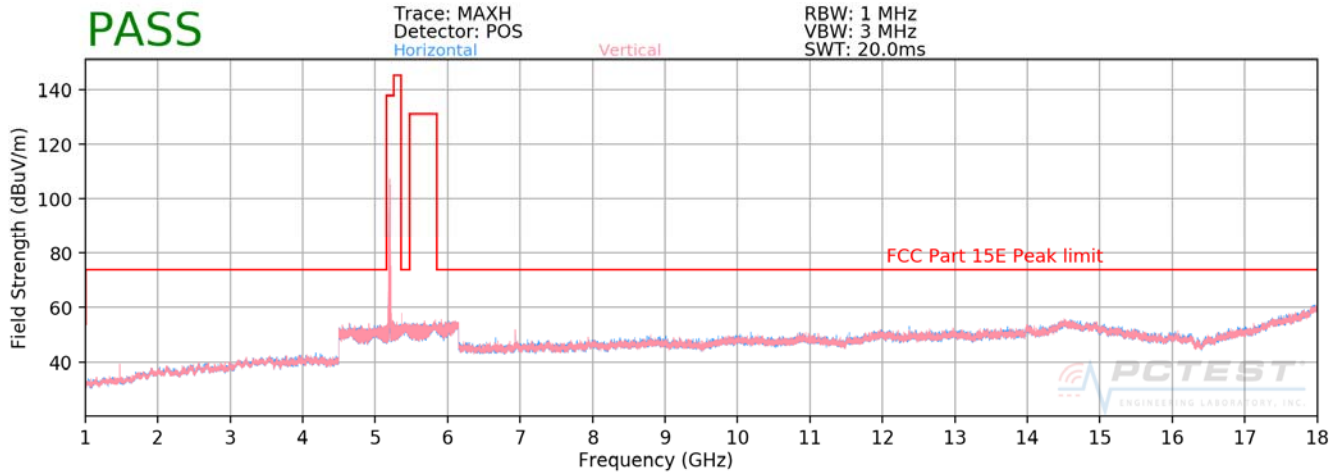
Plot 7-7. Radiated Spurious Plot above 1GHz (802.11a – U1 Ch. 40)
