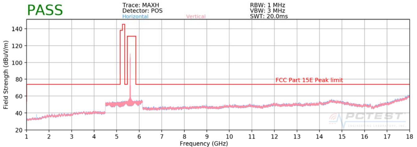
Plot 7-9. Radiated Spurious Plot above 1GHz (802.11a – U2C Ch. 116)
