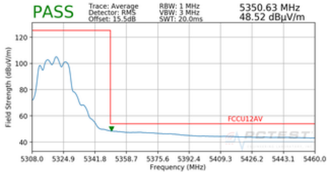
Plot 7-77. Radiated Band Edge Plot (Average – WCP)
