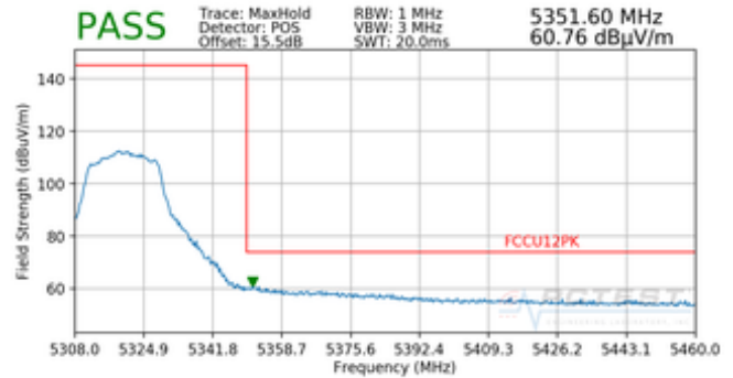
Plot 7-87. Radiated Band Edge Plot (Peak – WCP)
