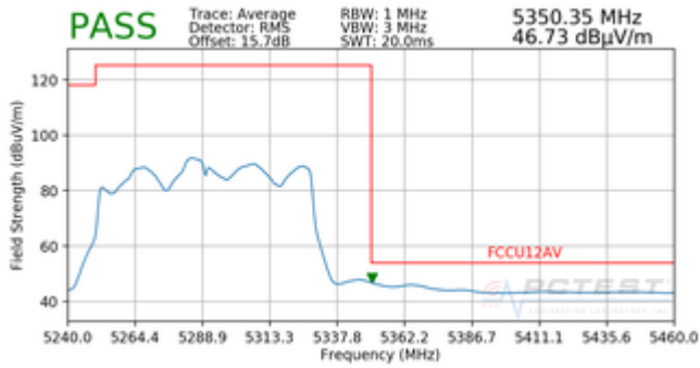
Plot 7-104. Radiated Band Edge Plot (Average – WCP)
