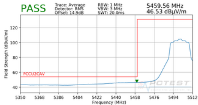
Plot 7-83. Radiated Lower Band Edge Plot (Average – UNII Band 2C)
