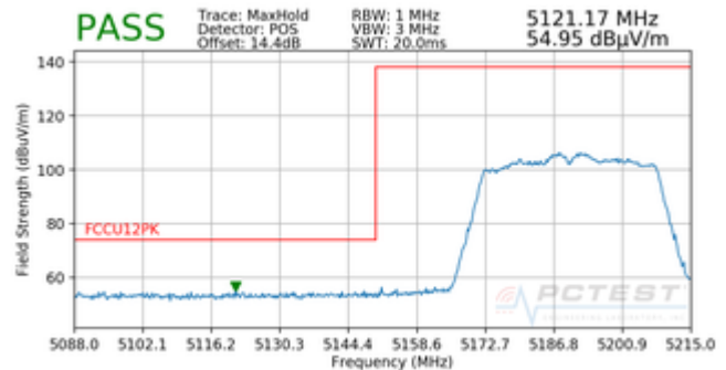
Plot 7-89. Radiated Lower Band Edge Plot (Peak – UNII Band 1)
