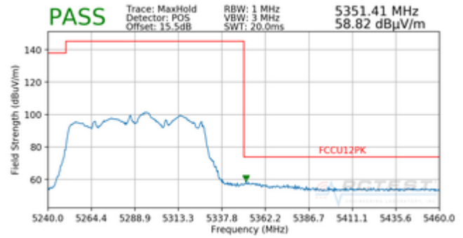
Plot 7-105. Radiated Band Edge Plot (Peak – WCP)
