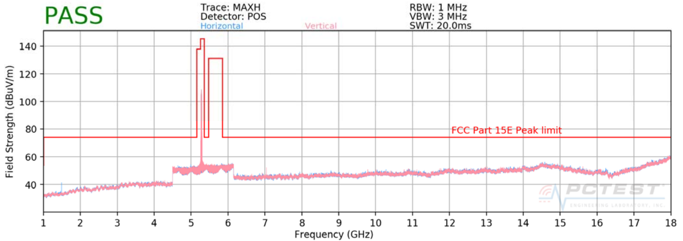
Plot 7-8. Radiated Spurious Plot above 1GHz (802.11a – U2A Ch. 56)
