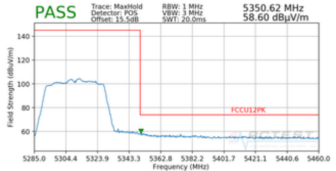
Plot 7-55. Radiated Upper Band Edge Plot (Peak – UNII Band 2A)
