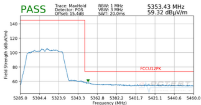
Plot 7-96. Radiated Band Edge Plot (Peak – WCP)
