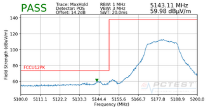
Plot 7-80. Radiated Lower Band Edge Plot (Peak – UNII Band 1)
