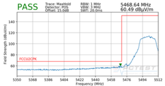
Plot 7-84. Radiated Lower Band Edge Plot (Peak – UNII Band 2C)
