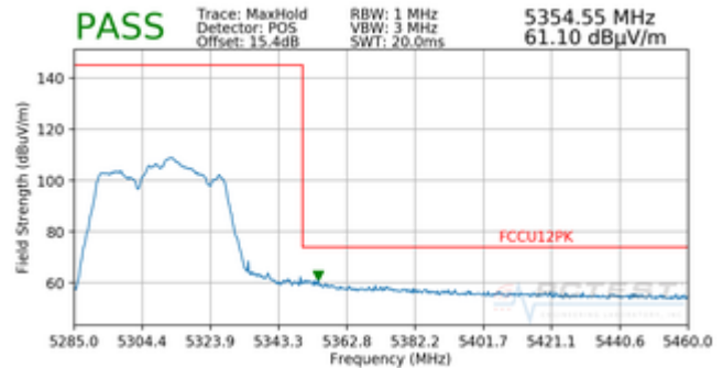
Plot 7-91. Radiated Upper Band Edge Plot (Peak – UNII Band 2A)
