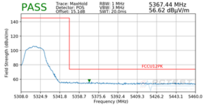
Plot 7-24. Radiated Band Edge Plot (Peak – WCP)
