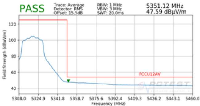
Plot 7-81. Radiated Upper Band Edge Plot (Average – UNII Band 2A)
