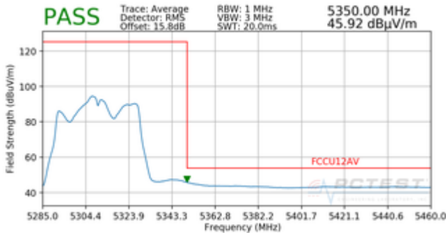
Plot 7-90. Radiated Upper Band Edge Plot (Average – UNII Band 2A)
