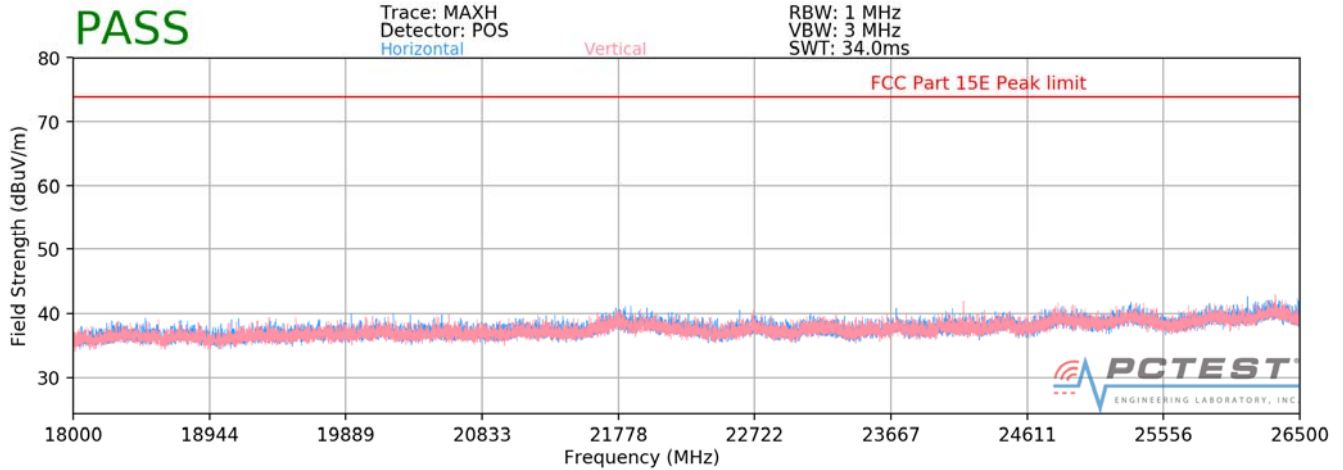
Plot 7-11. Radiated Spurious Plot above 18GHz - 26.5GHz (802.11a)
