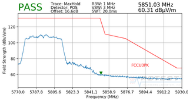
Plot 7-94. Radiated Upper Band Edge Plot (Peak – UNII Band 3)
