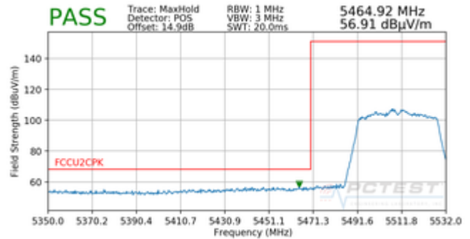
Plot 7-93. Radiated Lower Band Edge Plot (Peak – UNII Band 2C)
