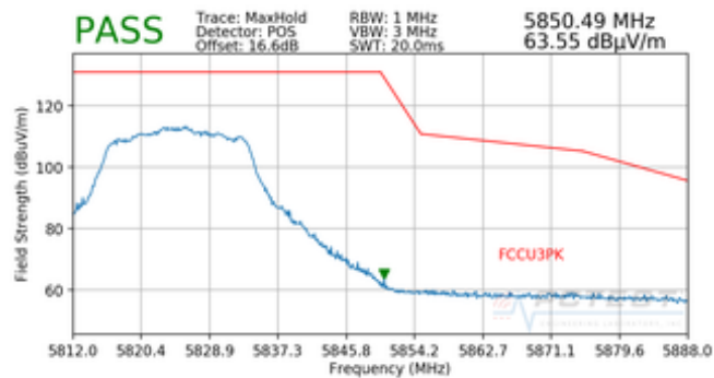
Plot 7-85. Radiated Upper Band Edge Plot (Peak – UNII Band 3)
