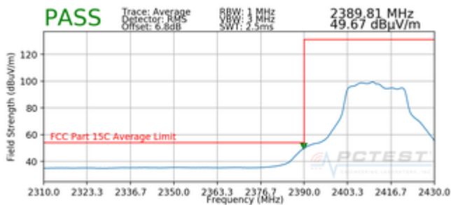
Plot 7-81. Radiated Restricted Lower Band Edge Measurement (Average)
