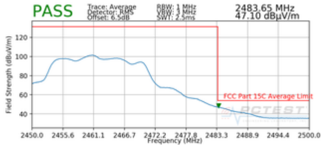
Plot 7-91. Radiated Restricted Band Edge Measurement with WCP (Average)
