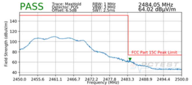
Plot 7-92. Radiated Restricted Band Edge Measurement with WCP (Peak)
