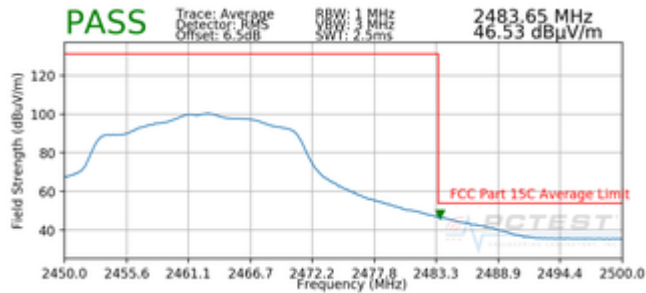
Plot 7-85. Radiated Restricted Band Edge Measurement with WCP (Average)
