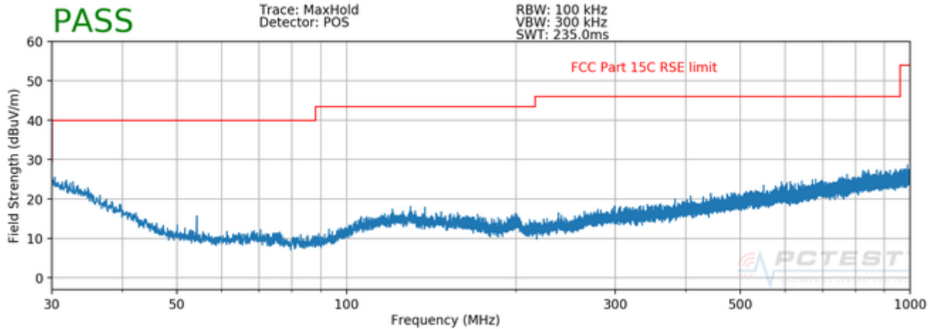
Plot 7-93. Radiated Spurious Plot below 1GHz (Pol. H)
