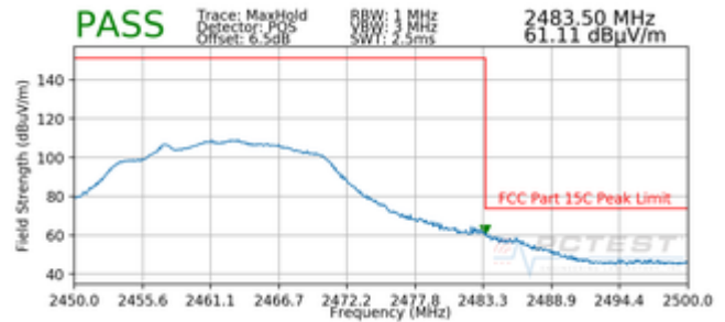
Plot 7-86. Radiated Restricted Band Edge Measurement with WCP (Peak)
