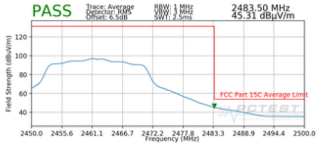
Plot 7-79. Radiated Restricted Band Edge Measurement with WCP (Average)
