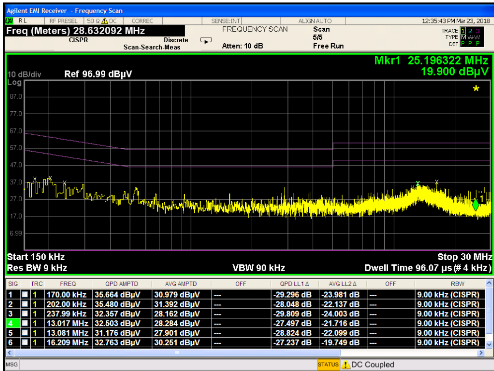
Plot 7-97. Line Conducted Plot with 802.11b (L1) with WCP
