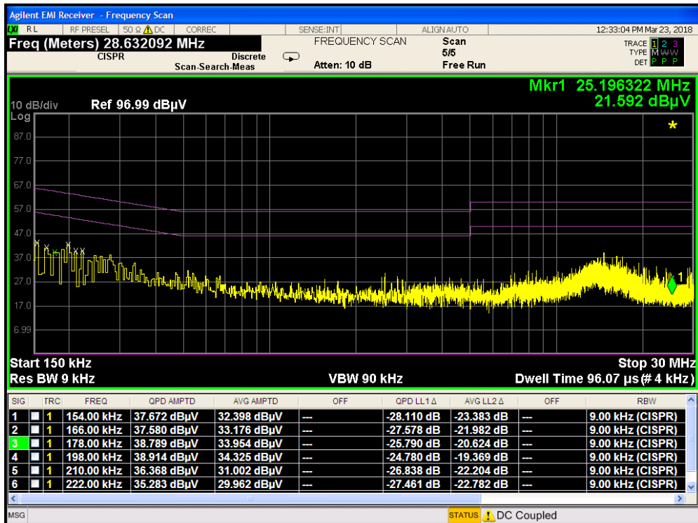
Plot 7-98. Line Conducted Plot with 802.11b (N) with WCP
