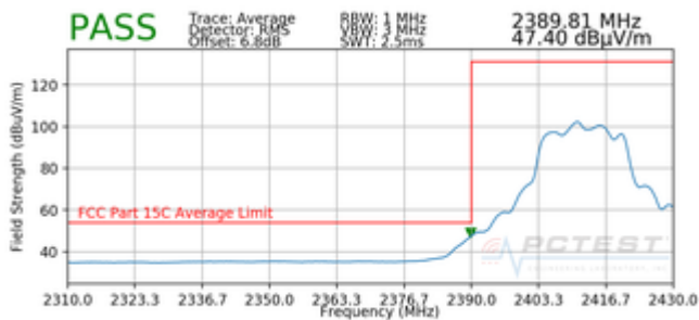
Plot 7-87. Radiated Restricted Lower Band Edge Measurement (Average)
