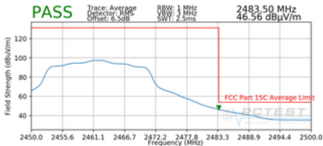
Plot 7-77. Radiated Restricted Upper Band Edge Measurement (Average)
