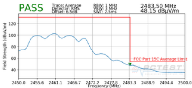
Plot 7-89. Radiated Restricted Upper Band Edge Measurement (Average)
