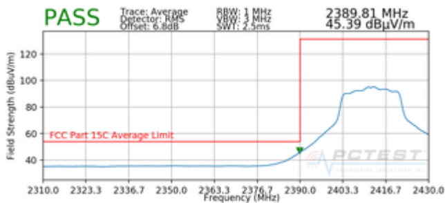
Plot 7-75. Radiated Restricted Lower Band Edge Measurement (Average)
