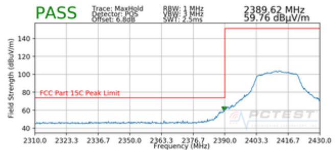
Plot 7-76. Radiated Restricted Lower Band Edge Measurement (Peak)
