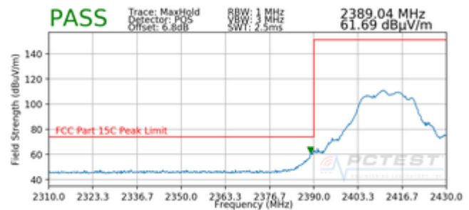
Plot 7-88. Radiated Restricted Lower Band Edge Measurement (Peak)
