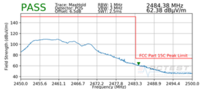
Plot 7-84. Radiated Restricted Upper Band Edge Measurement (Peak)
