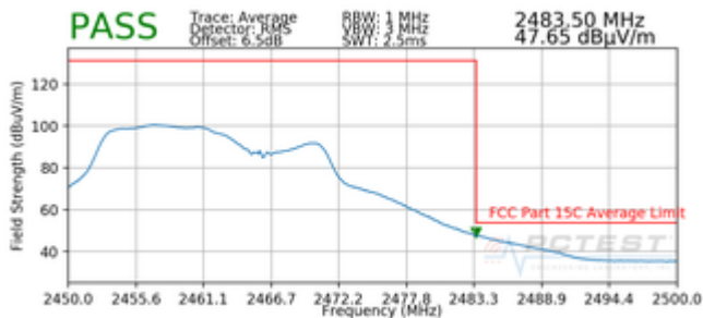
Plot 7-83. Radiated Restricted Upper Band Edge Measurement (Average)
