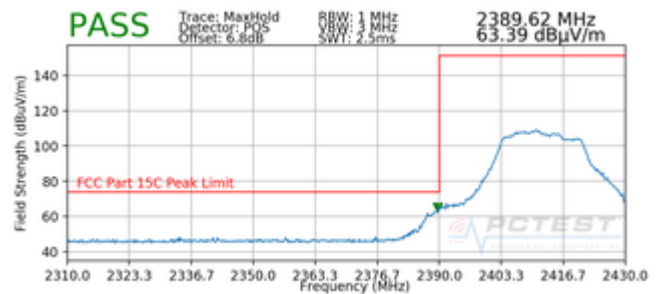
Plot 7-82. Radiated Restricted Lower Band Edge Measurement (Peak)
