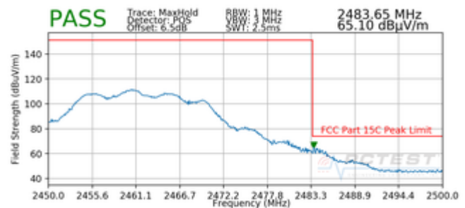
Plot 7-90. Radiated Restricted Upper Band Edge Measurement (Peak)
