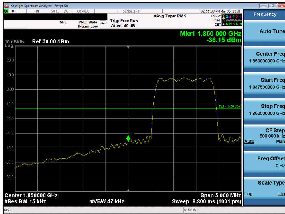
Plot 7-82. Band Edge Plot (PCS CDMA Mode - Low Channel)
