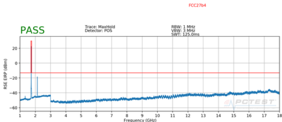
Plot 7-104. Radiated Spurious Plot above 1GHz (AWS WCDMA)
