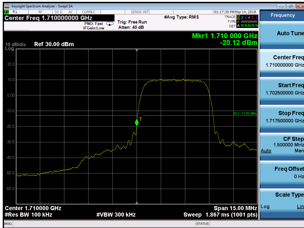
Plot 7-88. Band Edge Plot (AWS WCDMA Mode - Low Channel)
