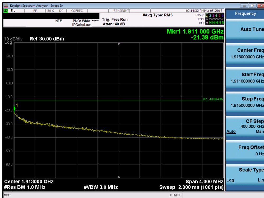
Plot 7-85. 4MHz Span Plot (PCS CDMA Mode - High Channel)
