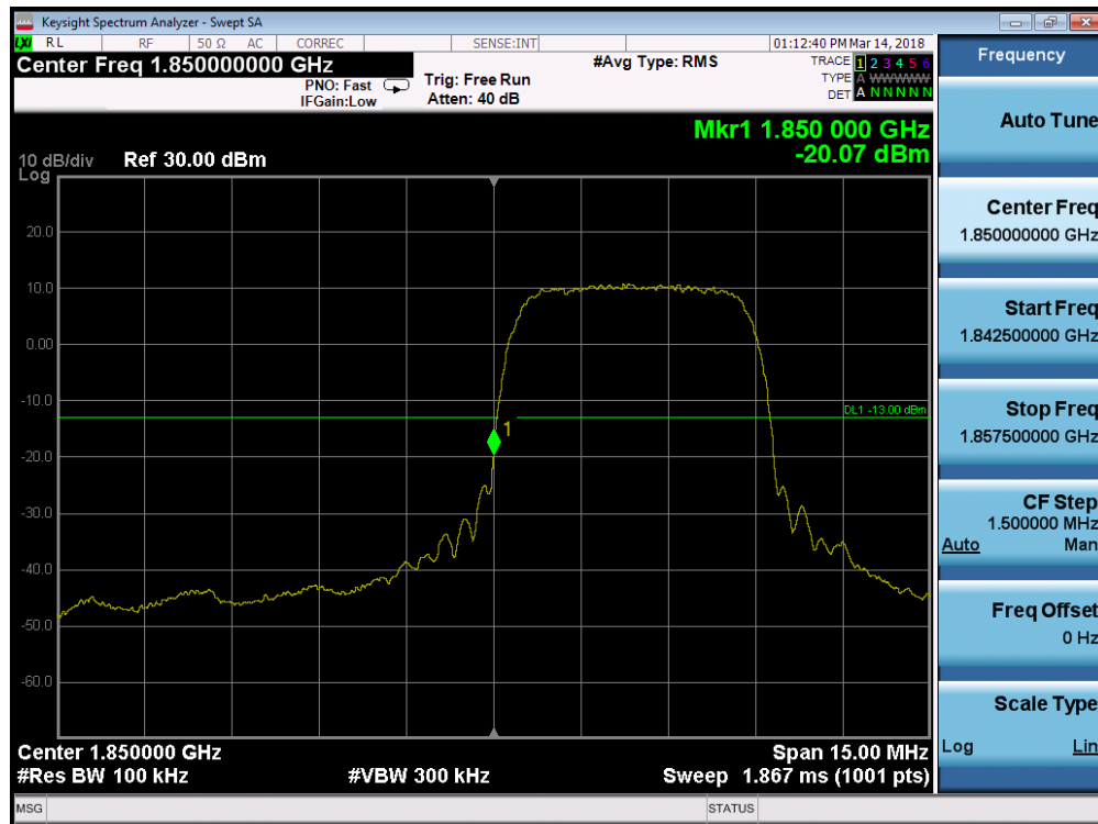
Plot 7-92. Band Edge Plot (PCS WCDMA Mode - Low Channel)
