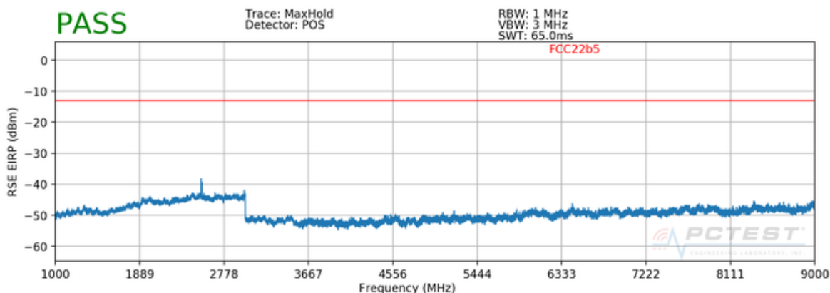
Plot 7-103. Radiated Spurious Plot above 1GHz (Cellular WCDMA)
