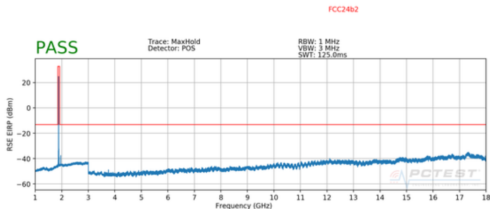
Plot 7-105. Radiated Spurious Plot above 1GHz (PCS GPRS)
