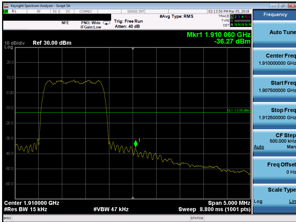
Plot 7-84. Band Edge Plot (PCS CDMA Mode - High Channel)
