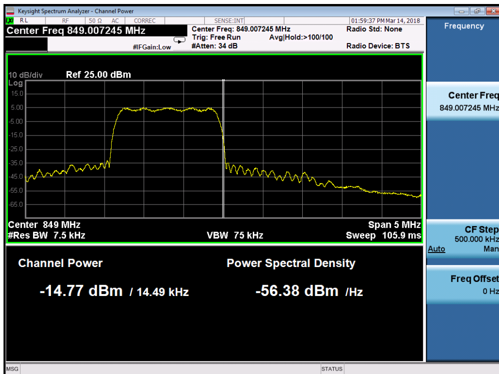
Plot 7-80. Band Edge Plot (Cellular CDMA Mode - High Channel)
