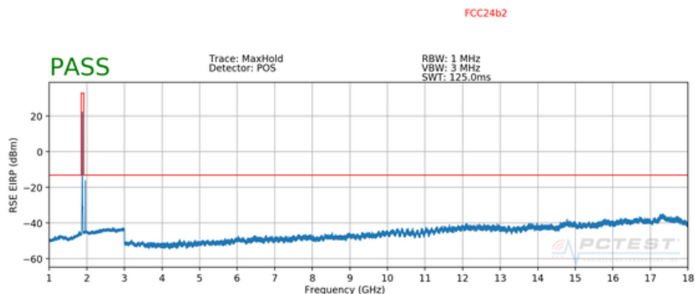
Plot 7-107. Radiated Spurious Plot above 1GHz (PCS WCDMA)
