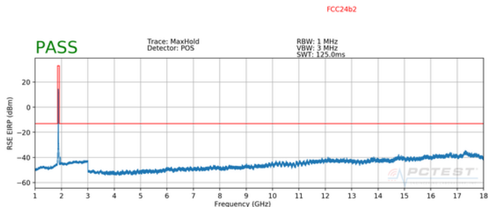
Plot 7-106. Radiated Spurious Plot above 1GHz (PCS CDMA)
