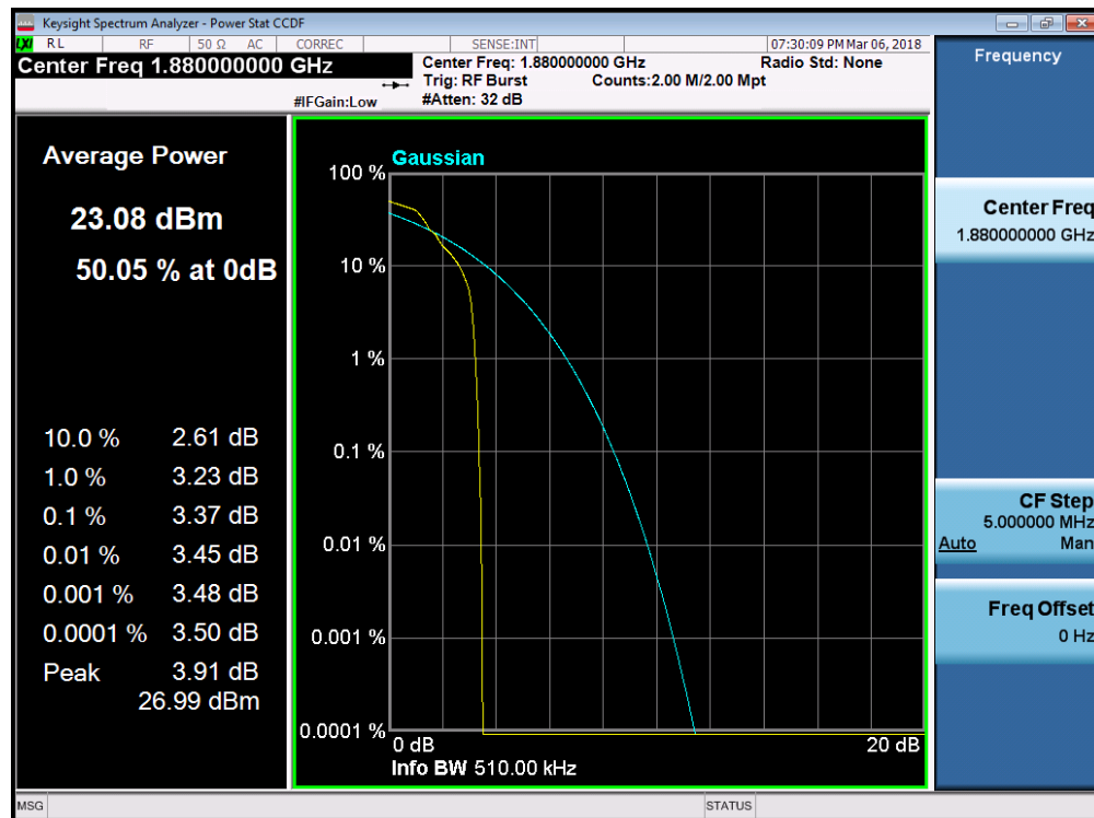
Plot 7-97. Peak-Average Ratio Plot (EDGE1900 Mode)
