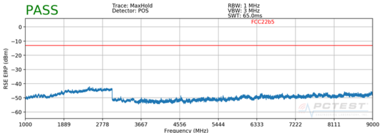
Plot 7-102. Radiated Spurious Plot above 1GHz (Cellular CDMA)
