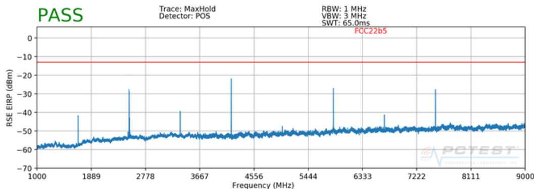
Plot 7-101. Radiated Spurious Plot above 1GHz (Cellular GPRS)
