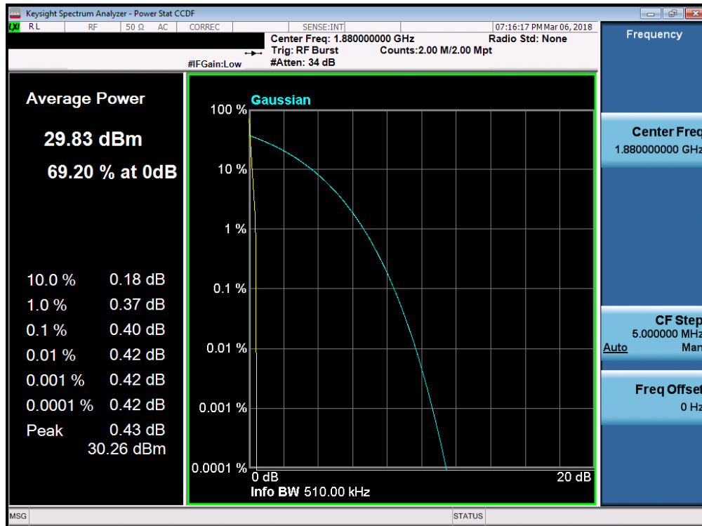
Plot 7-96. Peak-Average Ratio Plot (GPRS1900 Mode)
