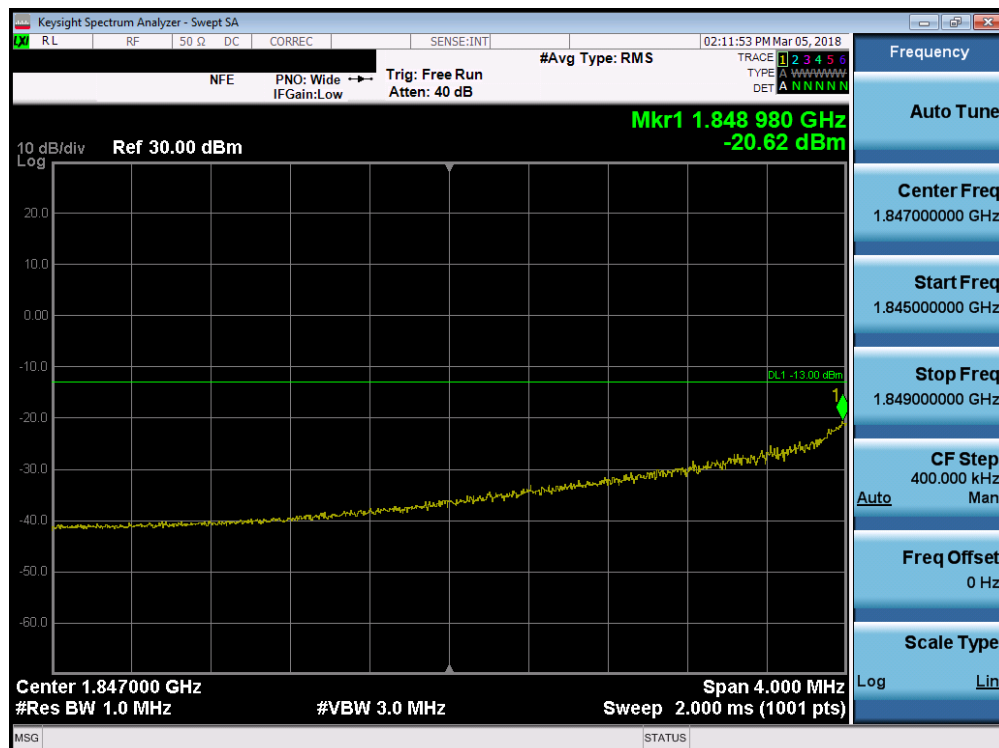
Plot 7-83. 4MHz Span Plot (PCS CDMA Mode - Low Channel)
