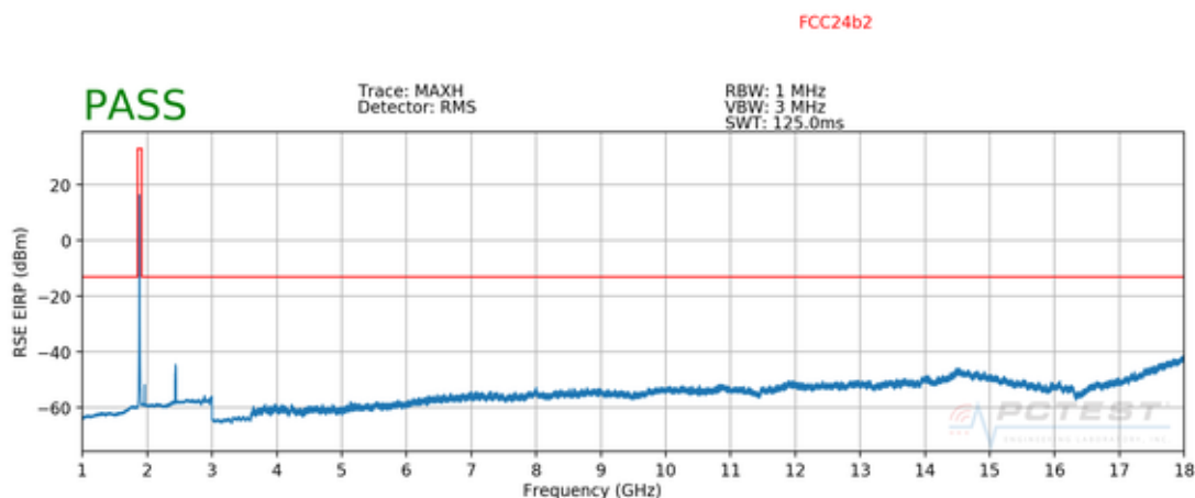
Plot 7-7. Radiated Spurious Plot above 1GHz (PCS WCDMA Mode)
