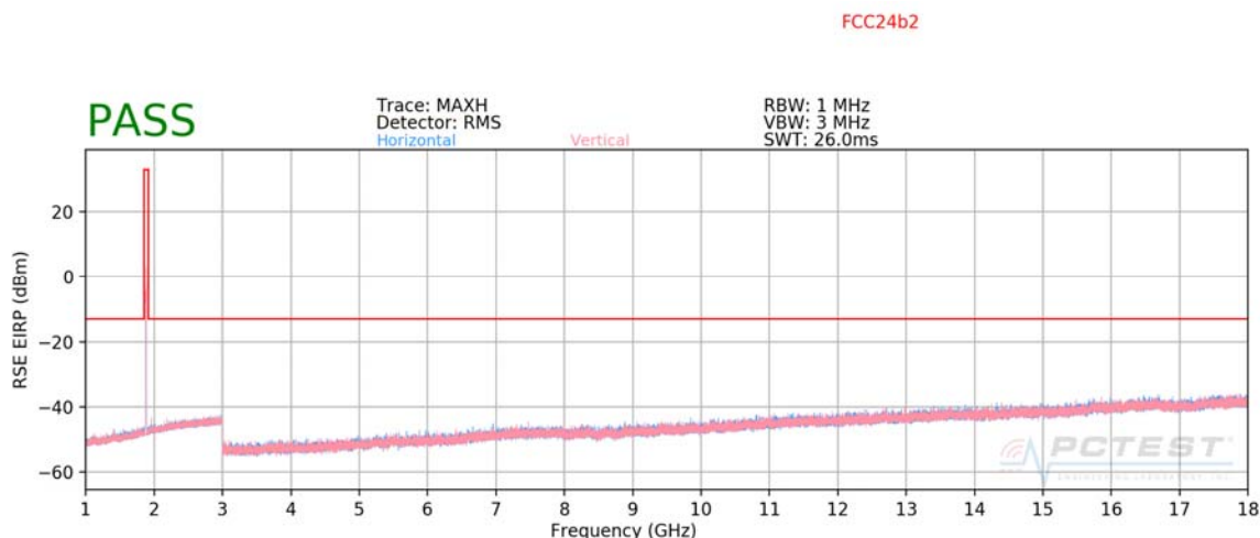
Plot 7-6. Radiated Spurious Plot above 1GHz (PCS CDMA Mode)
