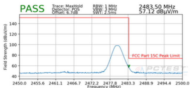
Plot 7-34. Radiated Restricted Upper Band Edge Measurement (Peak)
