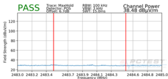
Plot 7-33. Radiated Restricted Upper Band Edge Measurement (Average)
