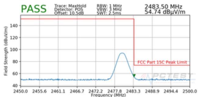
Plot 7-36. Radiated Restricted Upper Band Edge Measurement with WCP (Peak)
