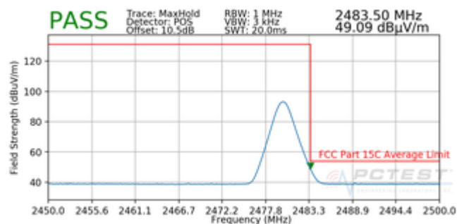
Plot 7-35. Radiated Restricted Upper Band Edge Measurement with WCP (Average)
