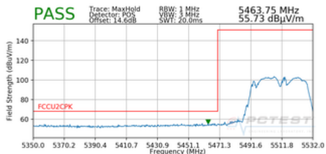
Plot 7-249. Radiated Lower Band Edge Plot (Peak – UNII Band 2C)
