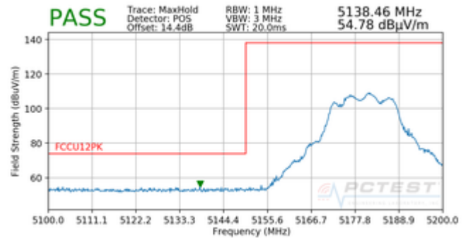
Plot 7-236. Radiated Lower Band Edge Plot (Peak – UNII Band 1)
