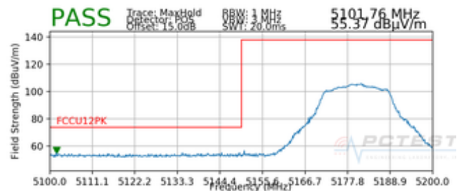
Plot 7-17. Radiated Lower Band Edge Plot SISO ANT1 (Peak – UNII Band 1)
