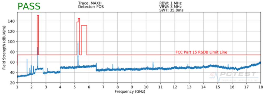
Plot 7-13. Radiated Spurious Plot above 1GHz (Simultaneous Transmission Config-1)
