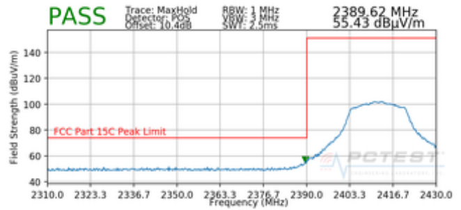
Plot 7-80. Radiated Restricted Band Edge Measurement with WCP (Peak)
