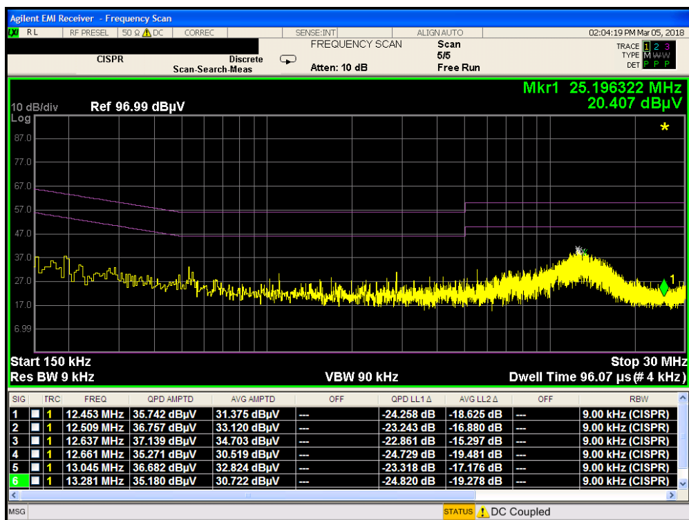
Plot 7-94. Line Conducted Plot with 802.11b (N)
