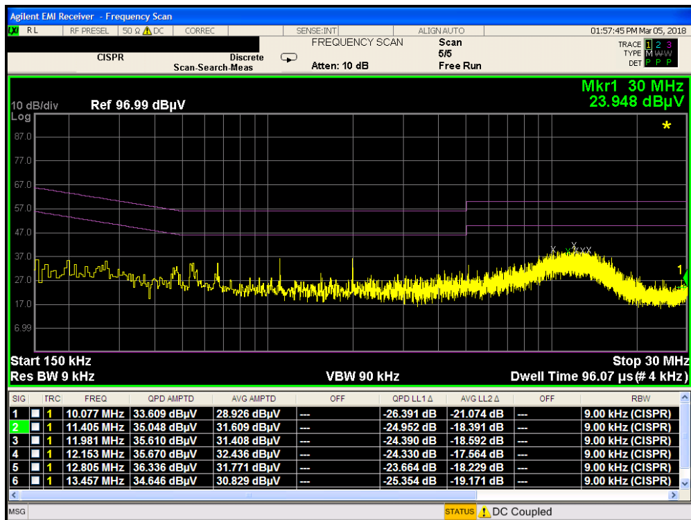
Plot 7-93. Line Conducted Plot with 802.11b (L1)
