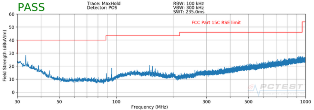
Plot 7-91. Radiated Spurious Plot below 1GHz
