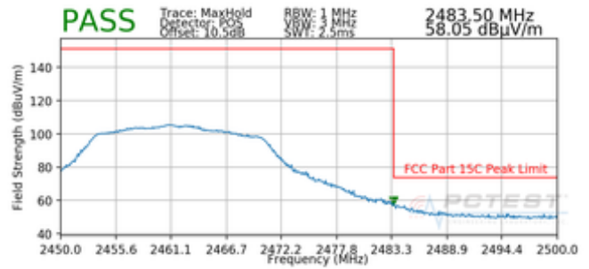
Plot 7-74. Radiated Restricted Band Edge Measurement with WCP (Peak)
