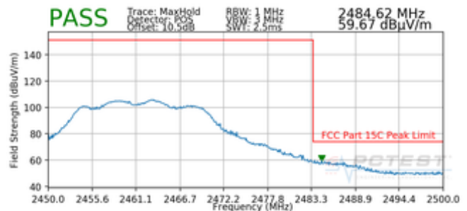
Plot 7-88. Radiated Restricted Upper Band Edge Measurement (Peak)
