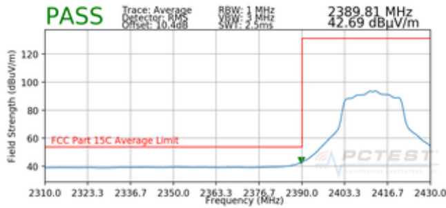
Plot 7-79. Radiated Restricted Band Edge Measurement with WCP (Average)
