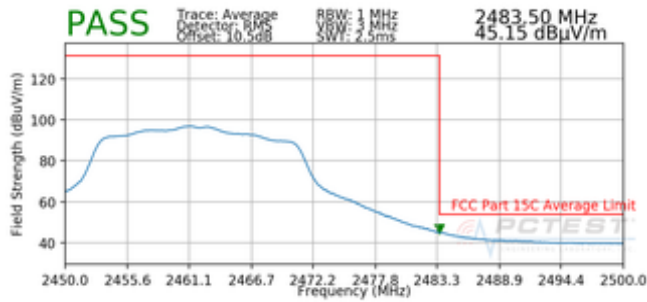
Plot 7-73. Radiated Restricted Band Edge Measurement with WCP (Average)
