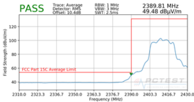
Plot 7-85. Radiated Restricted Lower Band Edge Measurement (Average)
