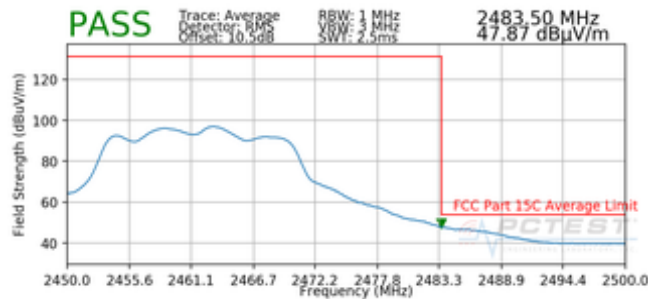
Plot 7-89. Radiated Restricted Band Edge Measurement with WCP (Average)
