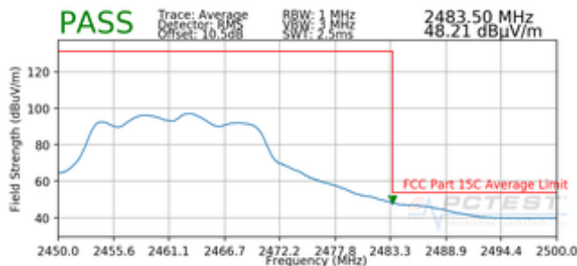
Plot 7-87. Radiated Restricted Upper Band Edge Measurement (Average)
