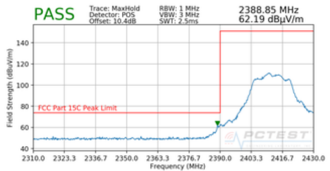
Plot 7-86. Radiated Restricted Lower Band Edge Measurement (Peak)
