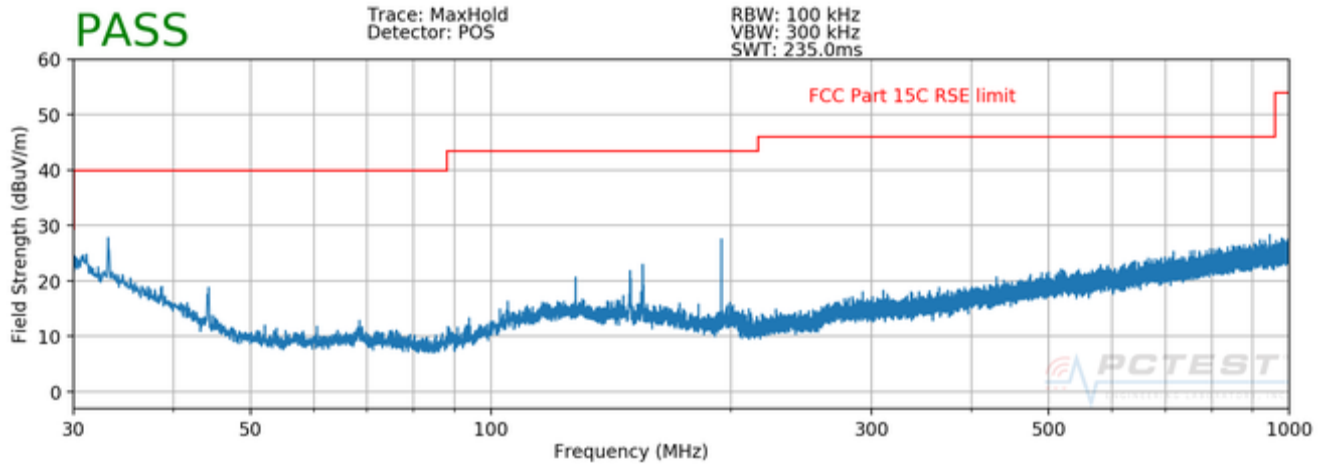
Plot 7-92. Radiated Spurious Plot below 1GHz
