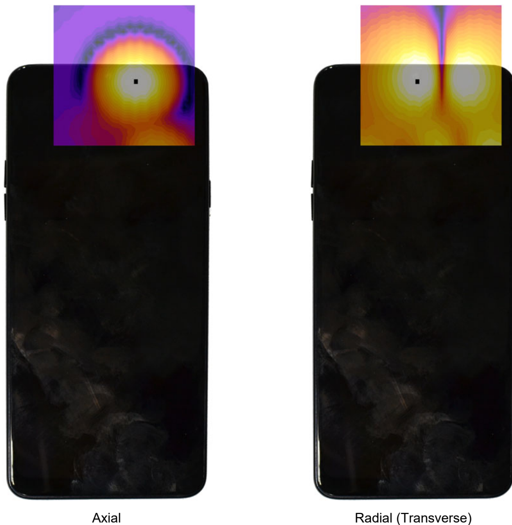
Axial Radial (Transverse) Figure 16-3 T-Coil Scan Overlay Magnetic Field Distributions
