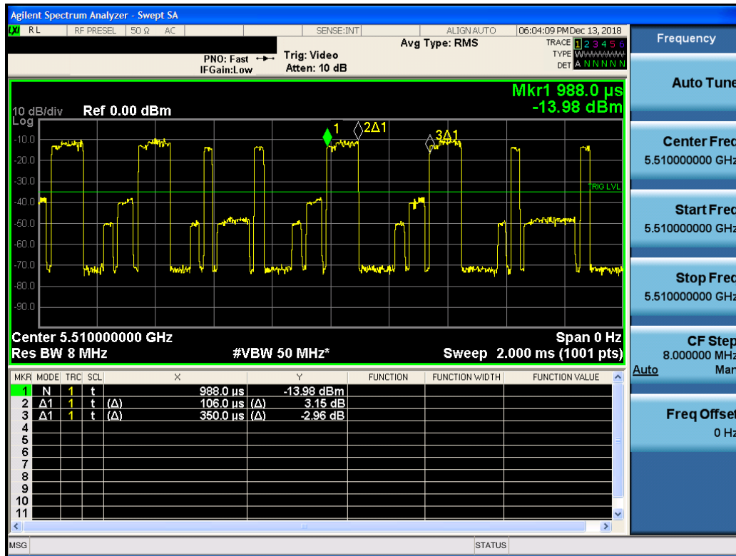
Figure 5-2. Band 2C Pulse Width + Period
