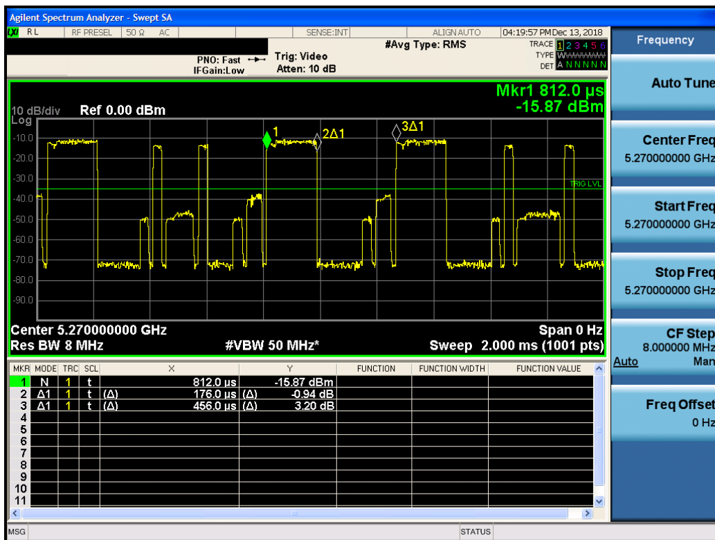
Figure 5-1. Band 2A Pulse Width + Period
