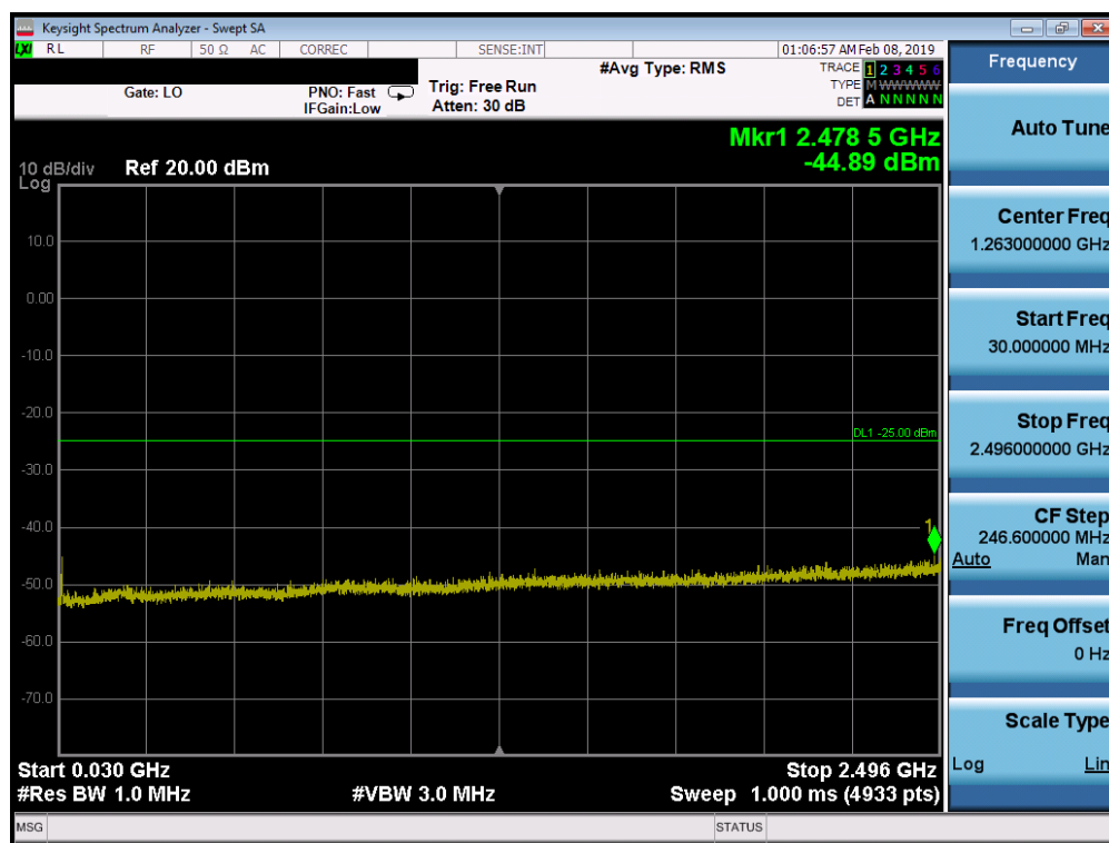
Plot 7-1. Conducted Spurious Plot (Band 41 – 20.0MHz QPSK – PCC 1/99 SCC 1/0 – Mid Channel)
