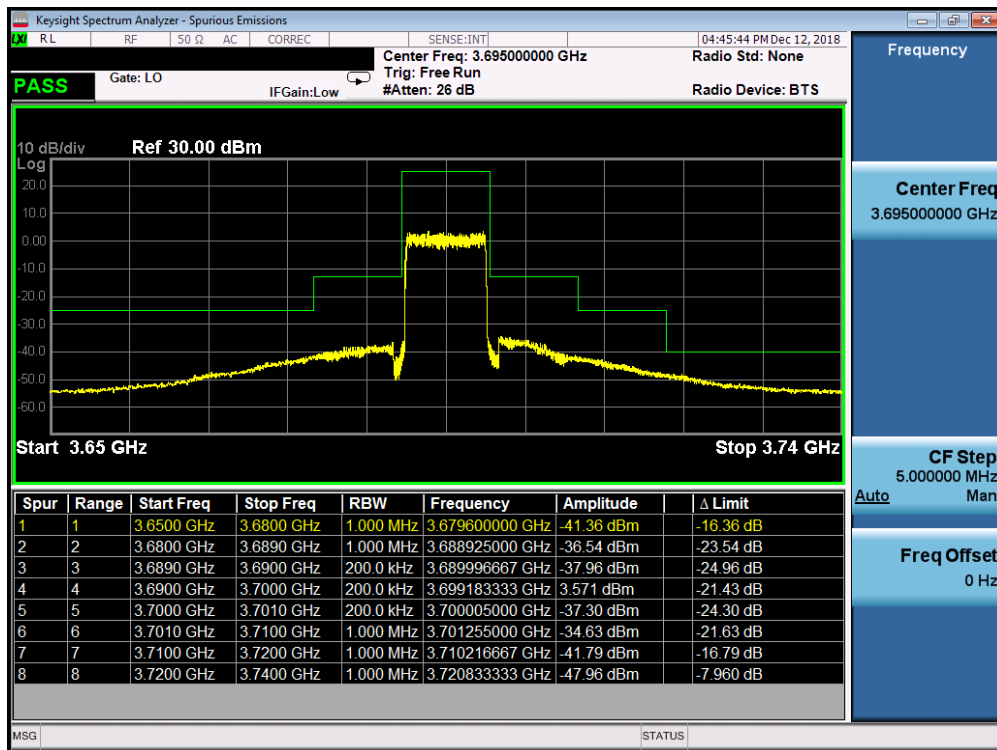
Plot 7-25. Upper ACP Plot (Band 48 - 10.0MHz QPSK - Full RB Configuration)
