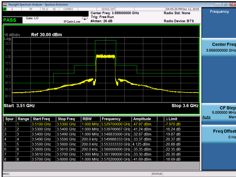
Plot 7-24. Lower ACP Plot (Band 48 - 10.0MHz QPSK - Full RB Configuration)
