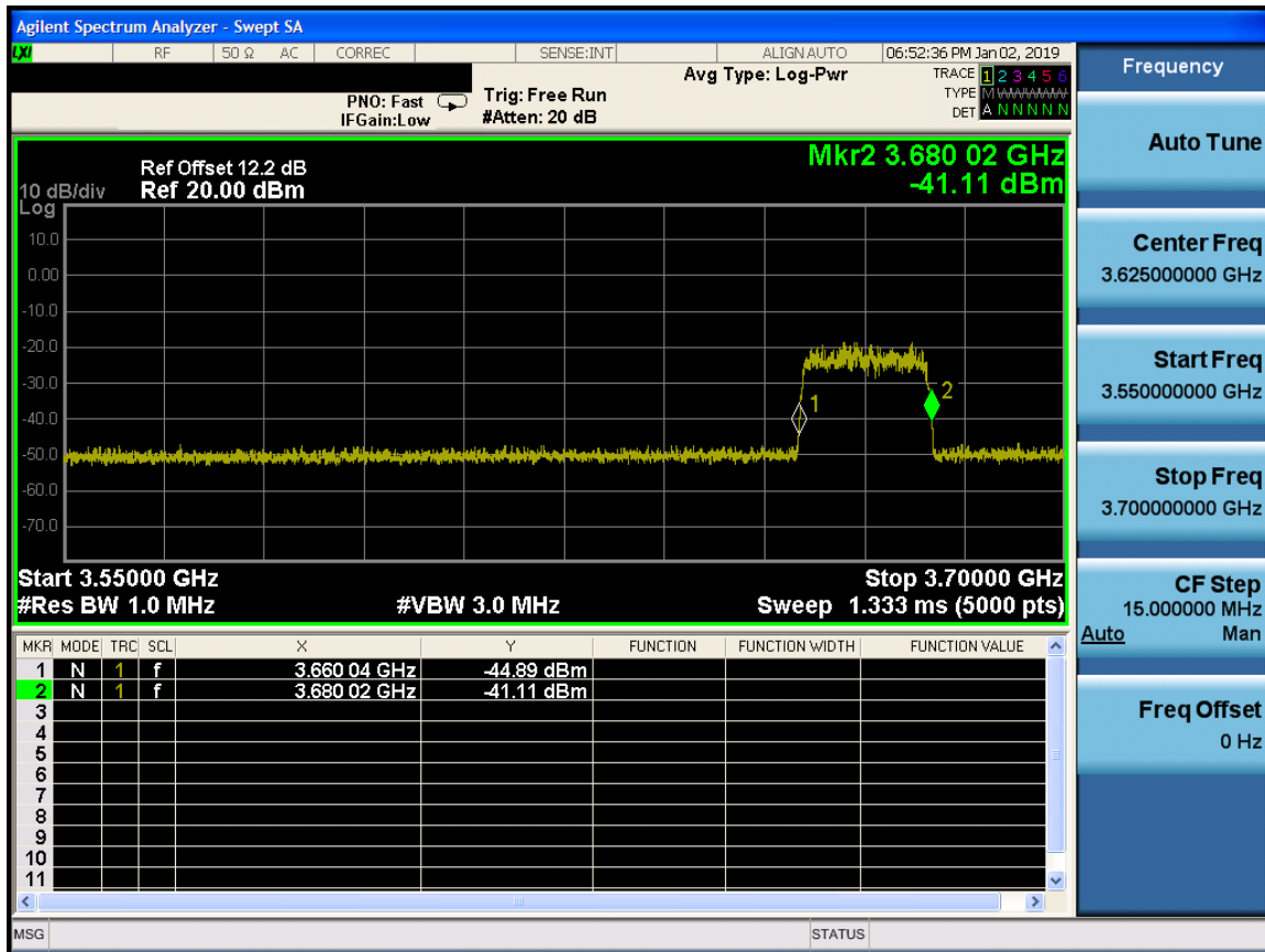
Plot 7-37. Run#2 End User Device Frequency of Operations
