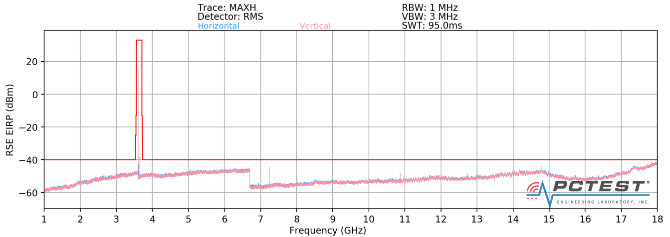
Plot 7-30. Radiated Spurious Plot 1GHz - 18GHz (Band 48)
