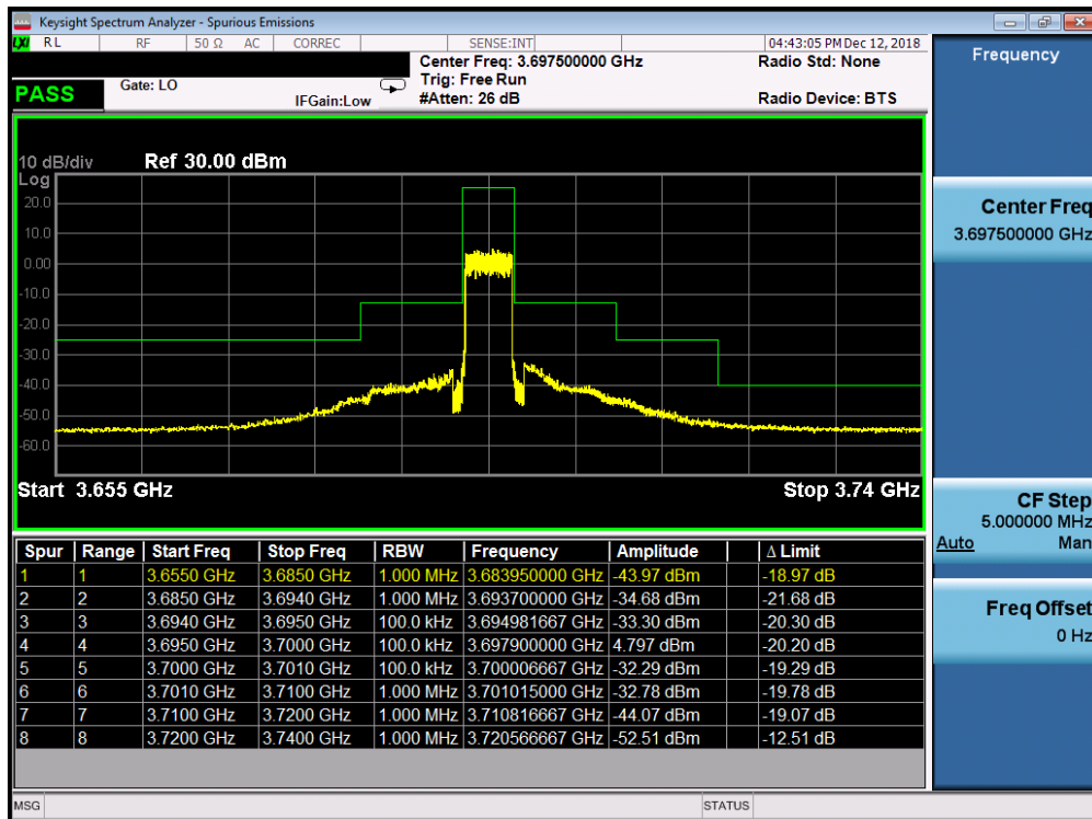
Plot 7-23. Upper ACP Plot (Band 48 - 5.0MHz QPSK - Full RB Configuration)
