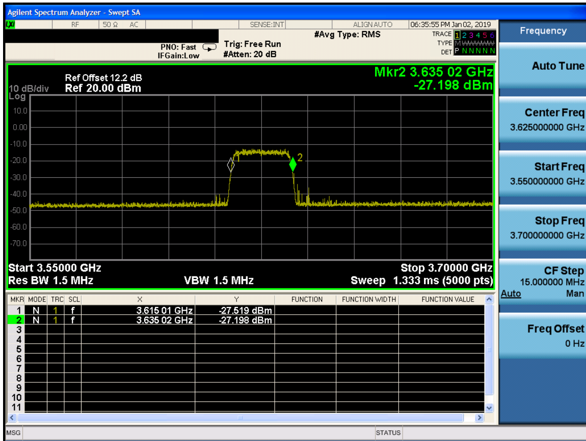
Plot 7-35. Run#1 End User Device Frequency of Operations
