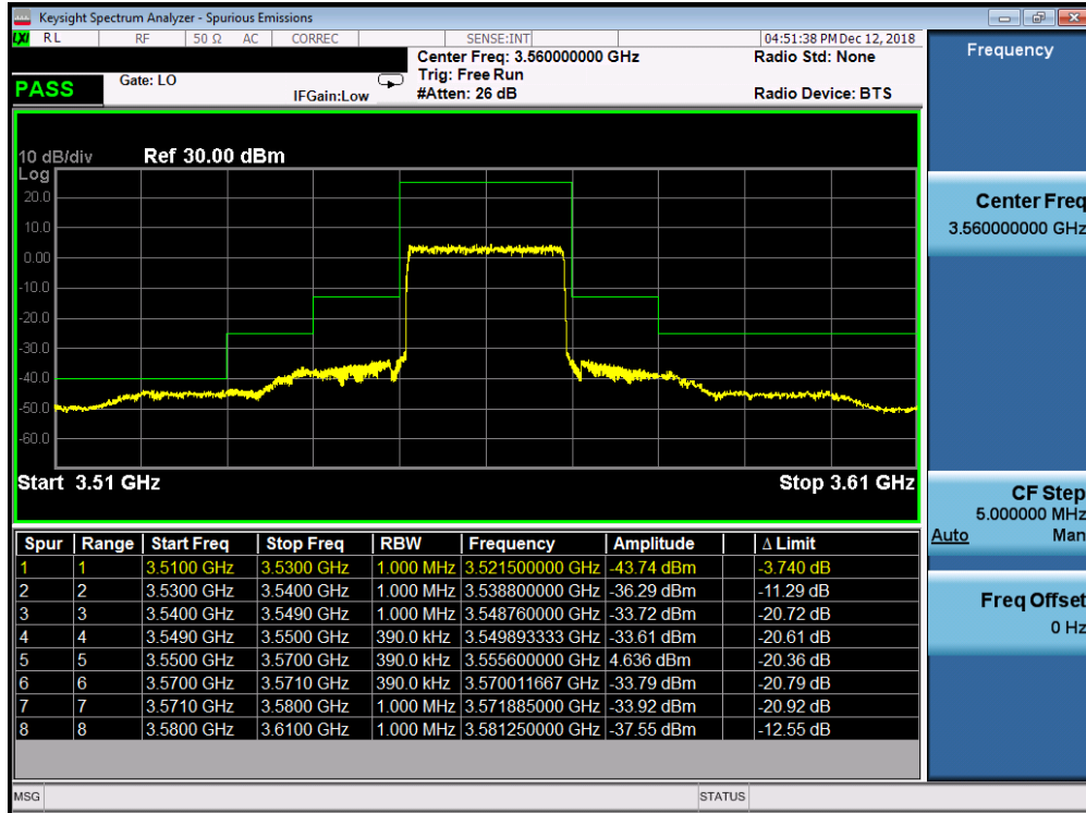
Plot 7-28. Lower ACP Plot (Band 48 - 20.0MHz QPSK - Full RB Configuration)
