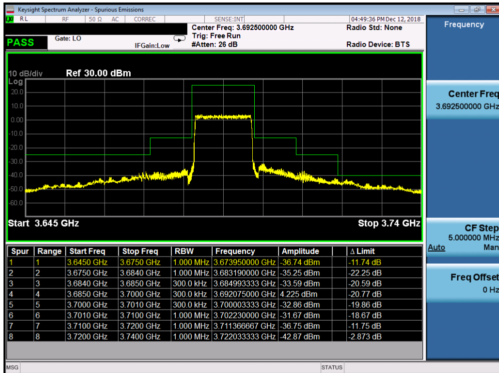
Plot 7-27. Upper ACP Plot (Band 48 - 15.0MHz QPSK - Full RB Configuration)
