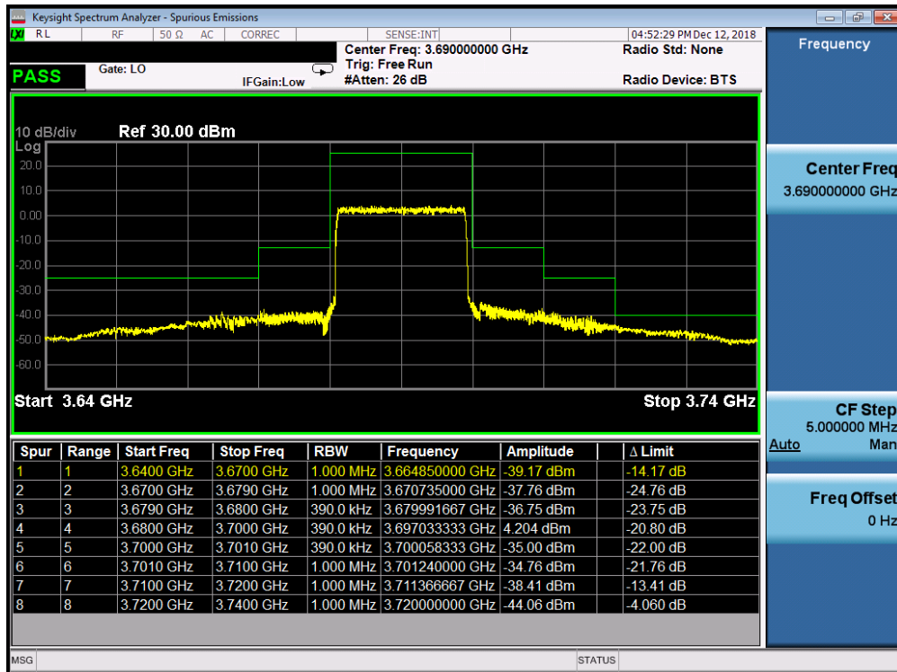
Plot 7-29. Upper ACP Plot (Band 48 - 20.0MHz QPSK - Full RB Configuration)
