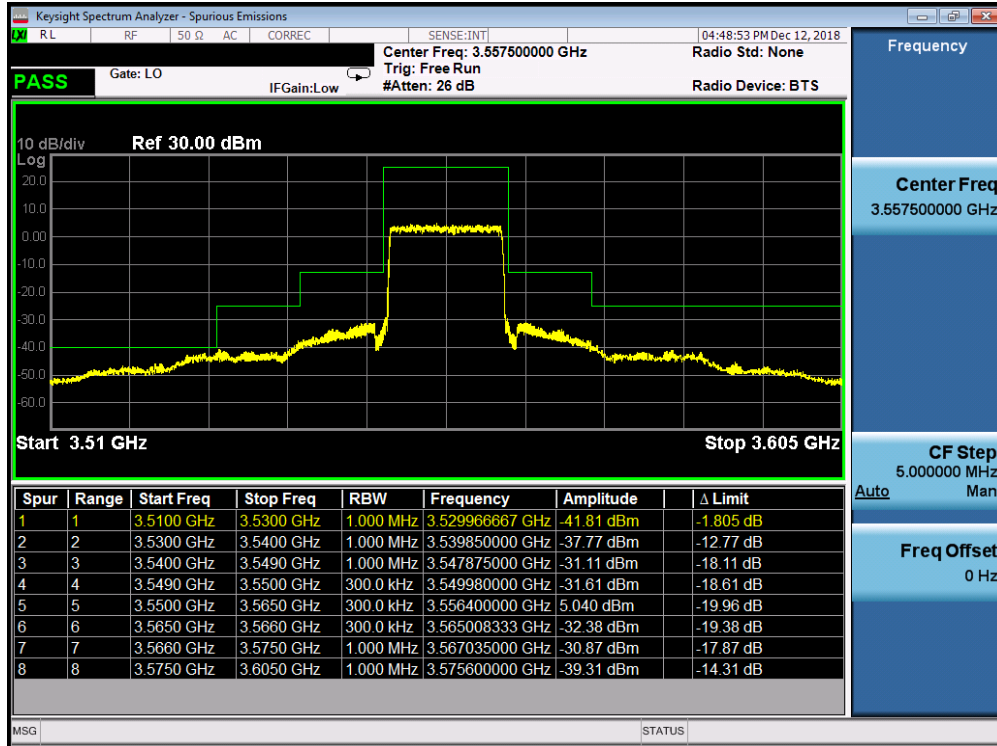
Plot 7-26. Lower ACP Plot (Band 48 - 15.0MHz QPSK - Full RB Configuration)
