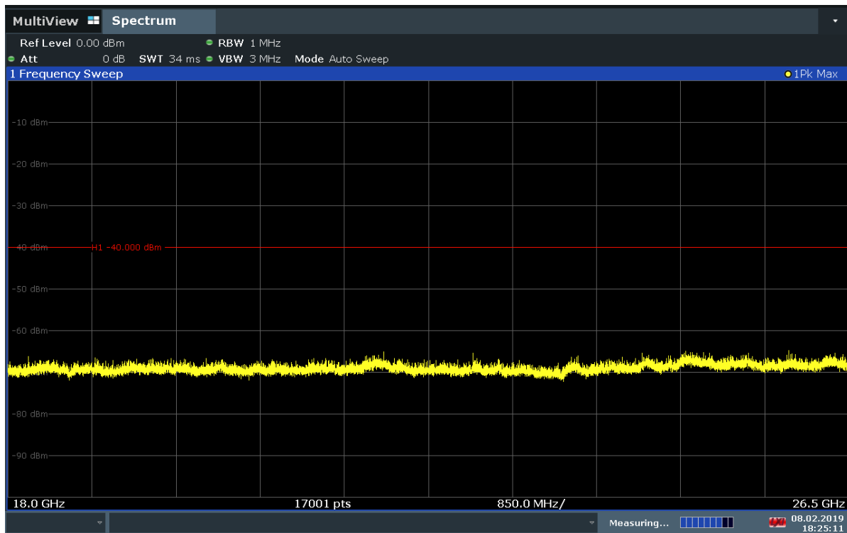
Plot 7-2. Radiated Spurious Plot 18GHz – 26.5GHz (Band 48) - H
