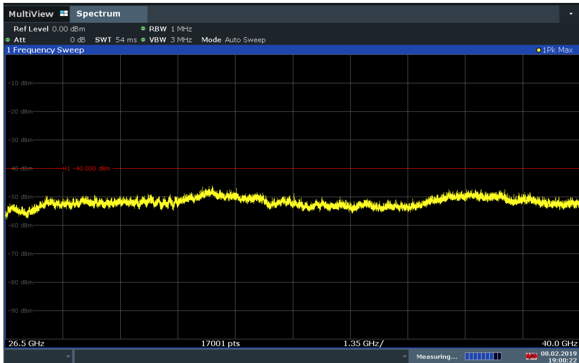
Plot 7-3. Radiated Spurious Plot 26.5GHz – 40GHz (Band 48) - V
