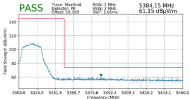
Plot 7-80. Radiated Upper Band Edge Plot (Peak – UNII Band 2A)
