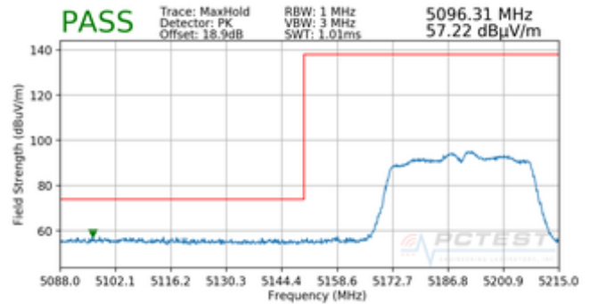
Plot 7-33. Radiated Band Edge Plot (Peak – WCP)
