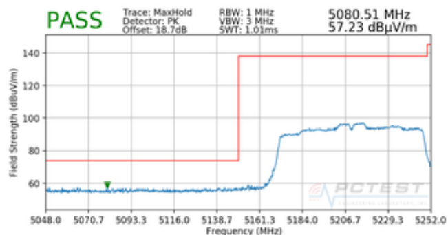
Plot 7-62. Radiated Lower Band Edge Plot (Peak – UNII Band 1)
