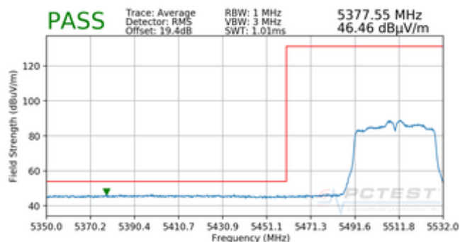
Plot 7-93. Radiated Band Edge Plot (Average – WCP)
