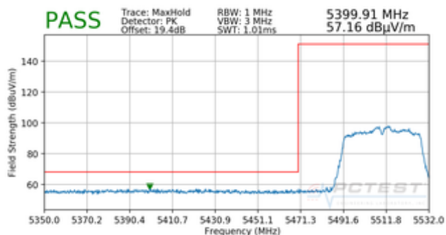
Plot 7-94. Radiated Band Edge Plot (Peak – WCP)
