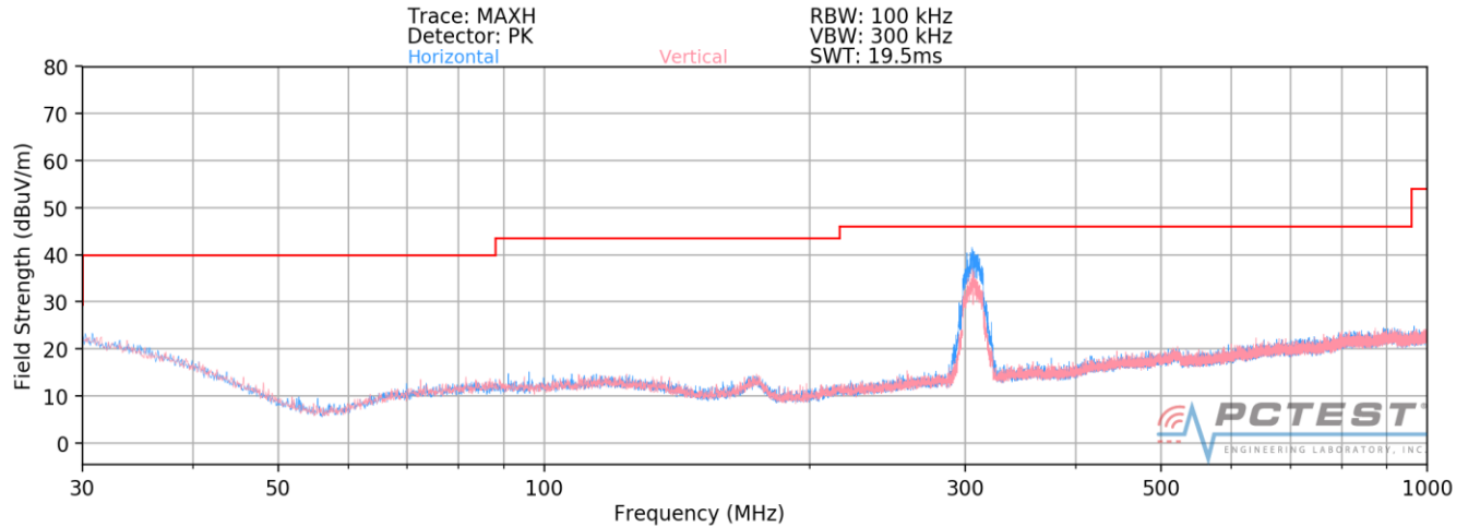
Plot 7-106. Radiated Spurious Plot below 1GHz (2.4GHz – 5GHz)
