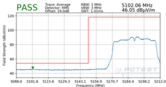
Plot 7-52. Radiated Lower Band Edge Plot (Average – UNII Band 1)
