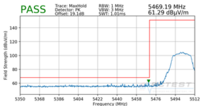
Plot 7-21. Radiated Lower Band Edge Plot (Peak – UNII Band 2C)
