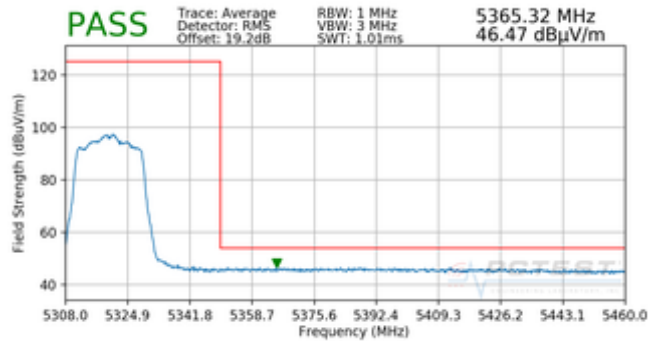
Plot 7-84. Radiated Band Edge Plot (Average – WCP)
