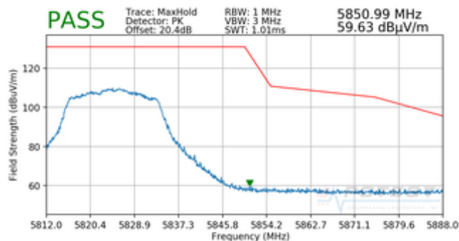
Plot 7-83. Radiated Upper Band Edge Plot (Peak – UNII Band 3)
