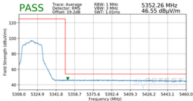
Plot 7-18. Radiated Upper Band Edge Plot (Average – UNII Band 2A)
