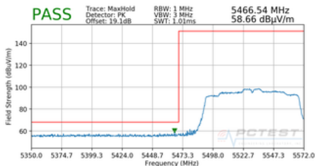
Plot 7-66. Radiated Lower Band Edge Plot (Peak – UNII Band 2C)
