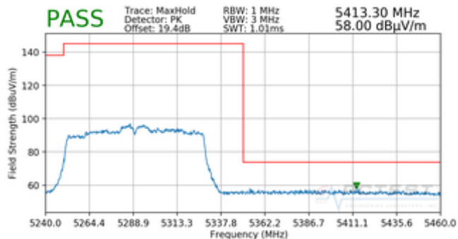
Plot 7-98. Radiated Upper Band Edge Plot (Peak – UNII Band 2A)
