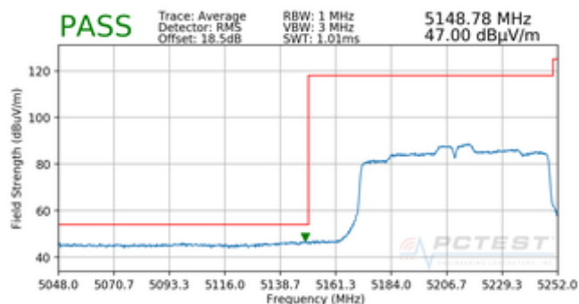
Plot 7-61. Radiated Lower Band Edge Plot (Average – UNII Band 1)
