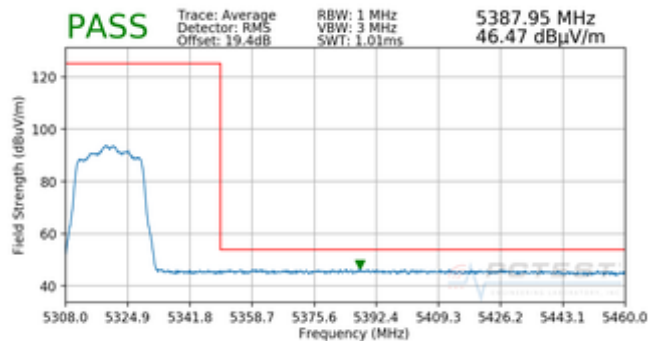
Plot 7-23. Radiated Band Edge Plot (Average – WCP)
