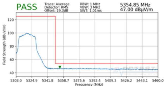
Plot 7-79. Radiated Upper Band Edge Plot (Average – UNII Band 2A)
