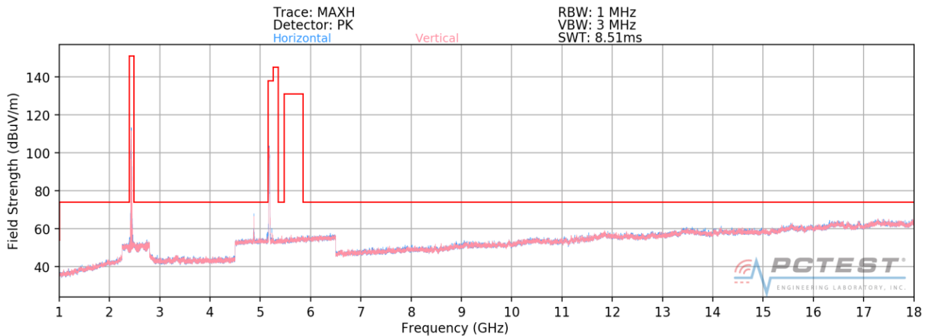
Plot 7-13. Radiated Spurious Plot above 1GHz (2.4GHz – 5GHz)
