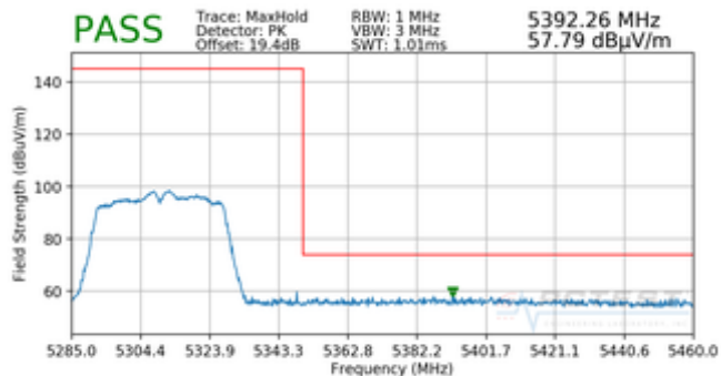
Plot 7-55. Radiated Upper Band Edge Plot (Peak – UNII Band 2A)
