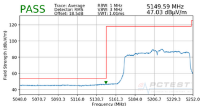
Plot 7-95. Radiated Lower Band Edge Plot (Average – UNII Band 1)
