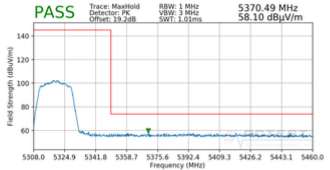
Plot 7-51. Radiated Band Edge Plot (Peak – WCP)
