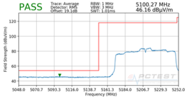
Plot 7-68. Radiated Band Edge Plot (Average – WCP)
