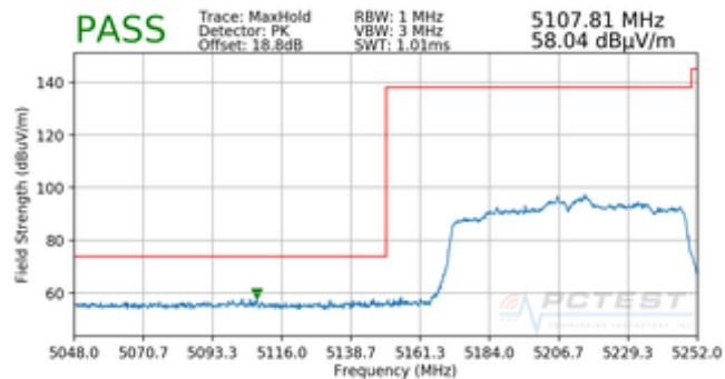
Plot 7-103. Radiated Band Edge Plot (Peak – WCP)
