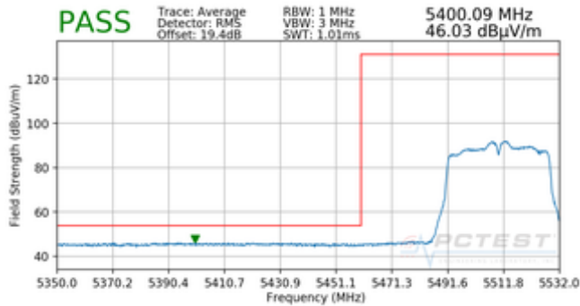
Plot 7-56. Radiated Lower Band Edge Plot (Average – UNII Band 2C)
