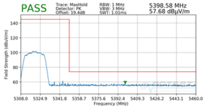
Plot 7-24. Radiated Band Edge Plot (Peak – WCP)
