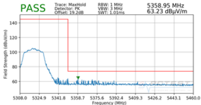
Plot 7-19. Radiated Upper Band Edge Plot (Peak – UNII Band 2A)
