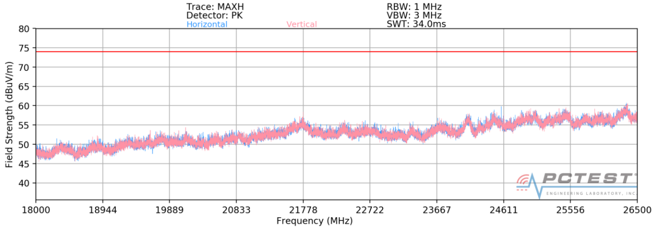
Plot 7-11. Radiated Spurious Plot 18GHz - 26.5GHz (802.11a)
