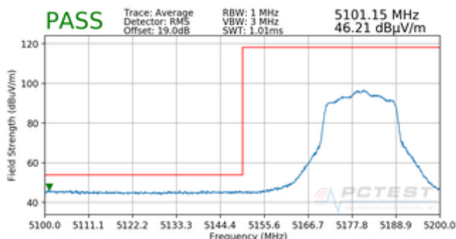
Plot 7-16. Radiated Lower Band Edge Plot (Average – UNII Band 1)
