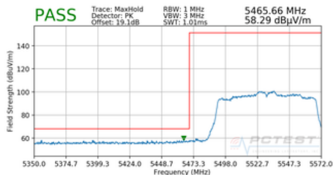
Plot 7-100. Radiated Lower Band Edge Plot (Peak – UNII Band 2C)
