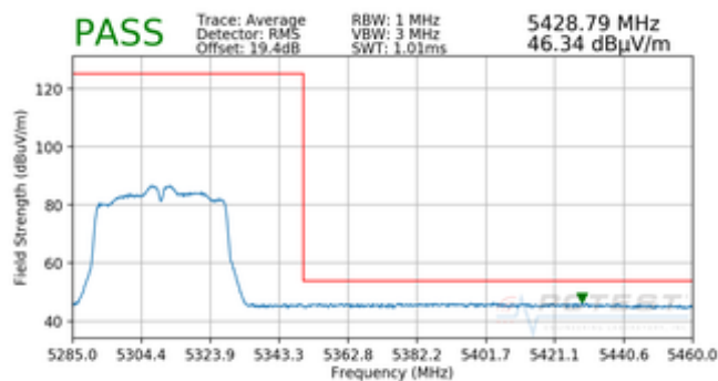
Plot 7-59. Radiated Band Edge Plot (Average – WCP)
