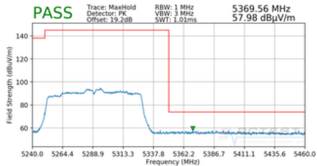
Plot 7-64. Radiated Upper Band Edge Plot (Peak – UNII Band 2A)
