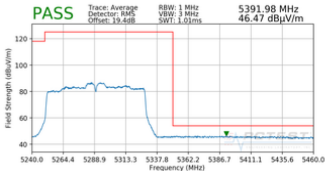
Plot 7-97. Radiated Upper Band Edge Plot (Average – UNII Band 2A)
