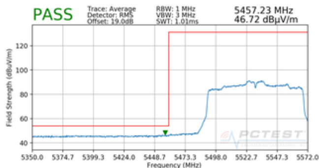
Plot 7-99. Radiated Lower Band Edge Plot (Average – UNII Band 2C)
