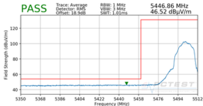
Plot 7-81. Radiated Lower Band Edge Plot (Average – UNII Band 2C)
