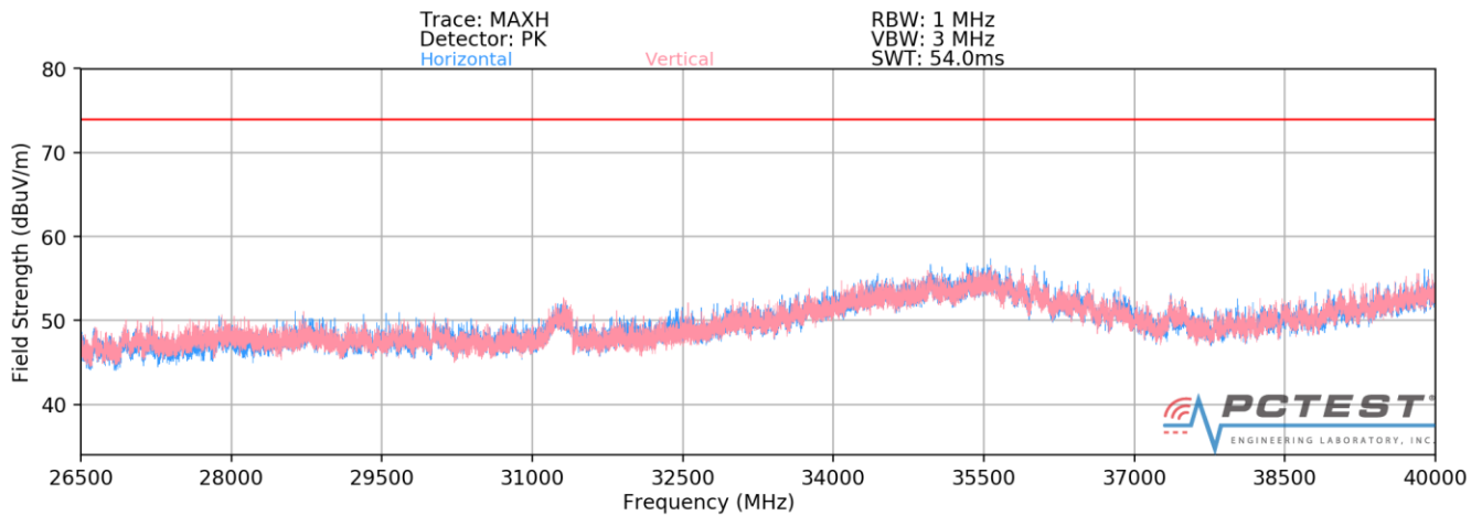
Plot 7-12. Radiated Spurious Plot 26.5GHz - 40GHz (802.11a)
