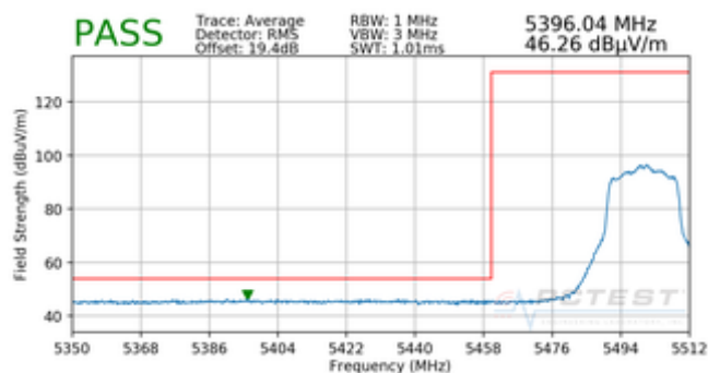
Plot 7-20. Radiated Lower Band Edge Plot (Average – UNII Band 2C)
