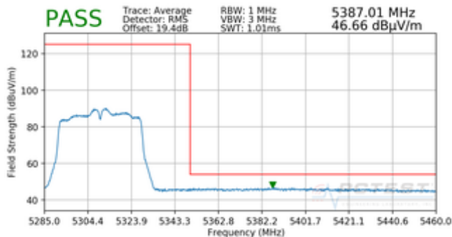
Plot 7-54. Radiated Upper Band Edge Plot (Average – UNII Band 2A)
