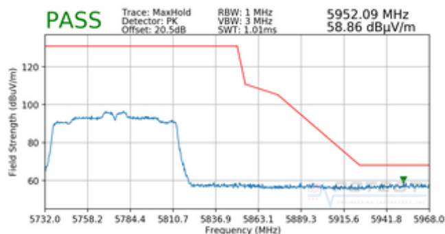
Plot 7-67. Radiated Upper Band Edge Plot (Peak – UNII Band 3)
