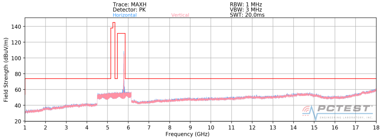
Plot 7-10. Radiated Spurious Plot above 1GHz (802.11a – U3 Ch. 157)
