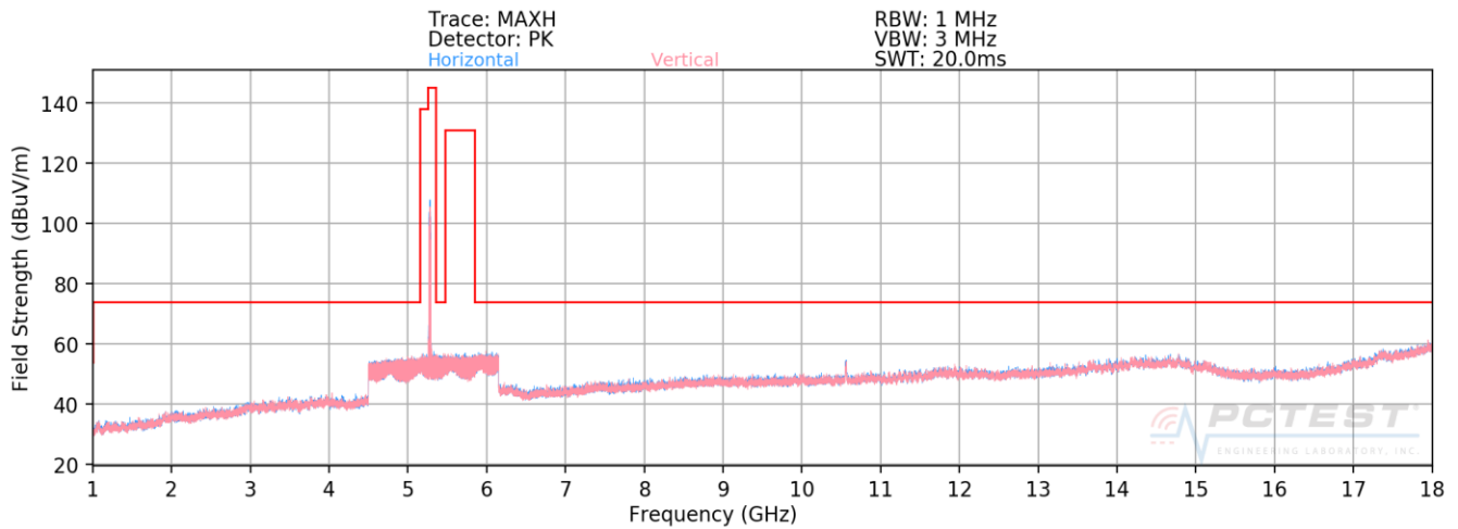
Plot 7-8. Radiated Spurious Plot above 1GHz (802.11a – U2A Ch. 56)
