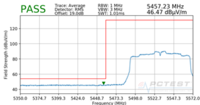
Plot 7-65. Radiated Lower Band Edge Plot (Average – UNII Band 2C)
