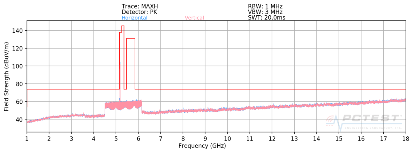
Plot 7-1. Radiated Spurious Plot above 1GHz (802.11a – U1 Ch. 40)
