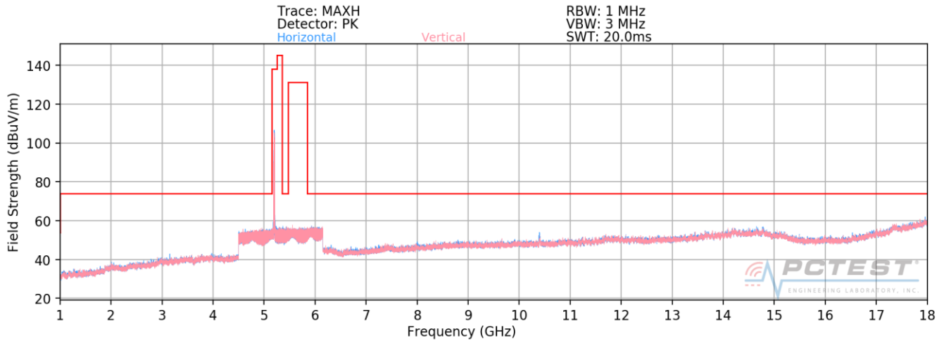
Plot 7-7. Radiated Spurious Plot above 1GHz (802.11a – U1 Ch. 40)
