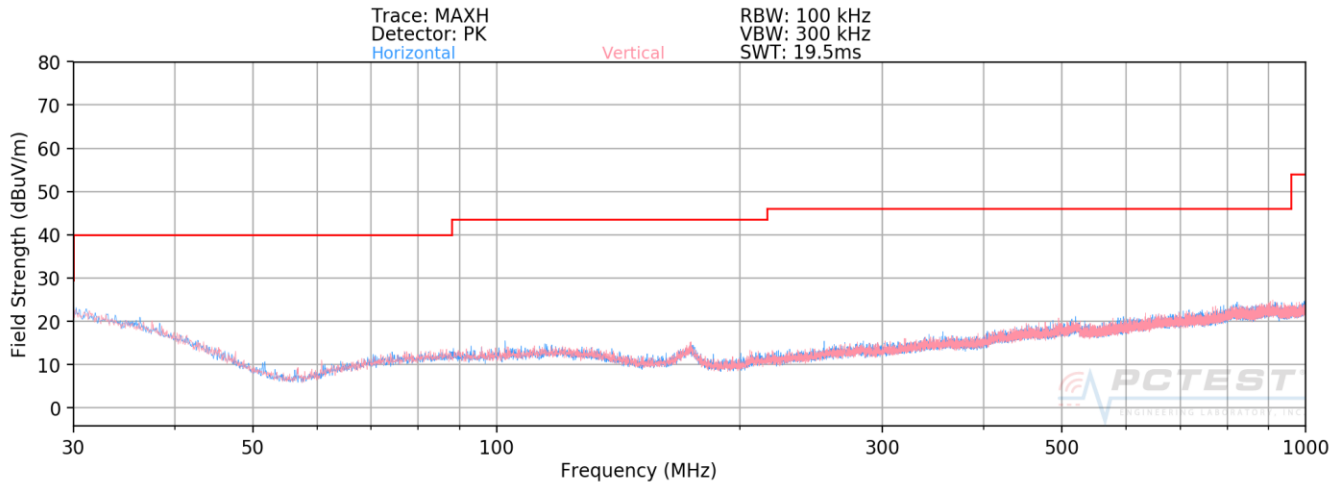
Plot 7-104. Radiated Spurious Plot below 1GHz
