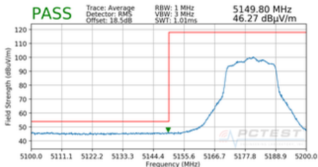
Plot 7-77. Radiated Lower Band Edge Plot (Average – UNII Band 1)
