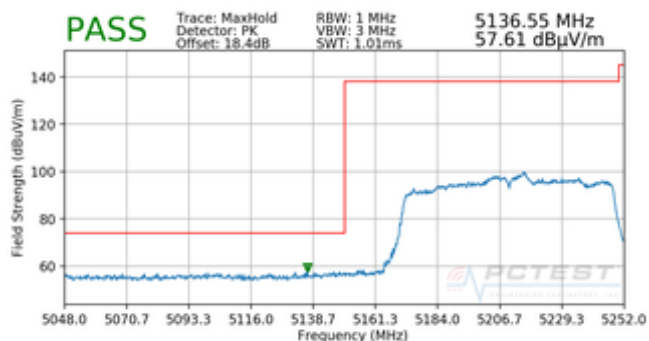
Plot 7-96. Radiated Lower Band Edge Plot (Peak – UNII Band 1)
