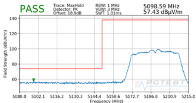
Plot 7-53. Radiated Lower Band Edge Plot (Peak – UNII Band 1)
