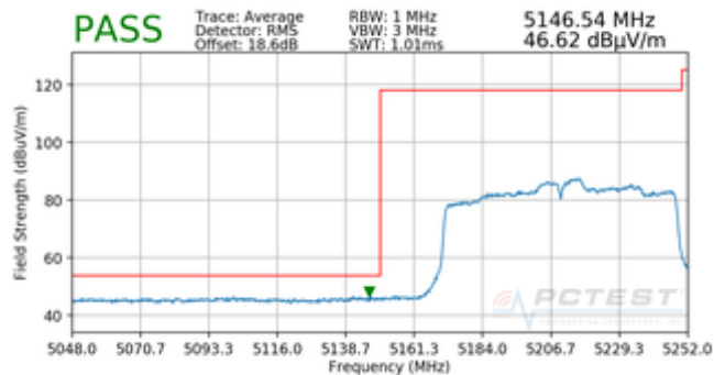
Plot 7-102. Radiated Band Edge Plot (Average – WCP)
