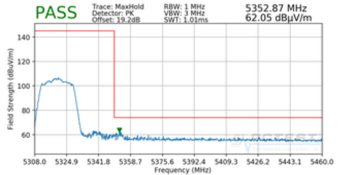
Plot 7-85. Radiated Band Edge Plot (Peak – WCP)
