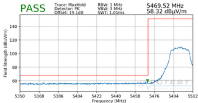
Plot 7-82. Radiated Lower Band Edge Plot (Peak – UNII Band 2C)
