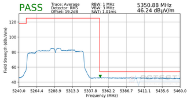
Plot 7-63. Radiated Upper Band Edge Plot (Average – UNII Band 2A)
