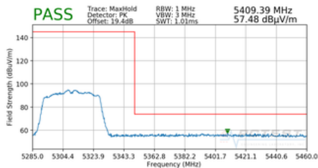
Plot 7-60. Radiated Band Edge Plot (Peak – WCP)
