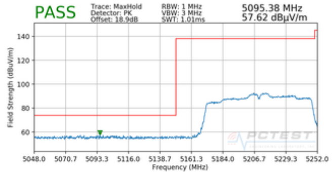
Plot 7-69. Radiated Band Edge Plot (Peak – WCP)
