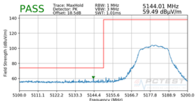
Plot 7-17. Radiated Lower Band Edge Plot (Peak – UNII Band 1)
