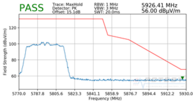
Plot 7-58. Radiated Upper Band Edge Plot (Peak – UNII Band 3)
