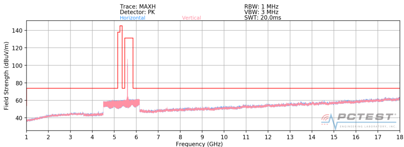
Plot 7-3. Radiated Spurious Plot above 1GHz (802.11a – U2C Ch. 120)
