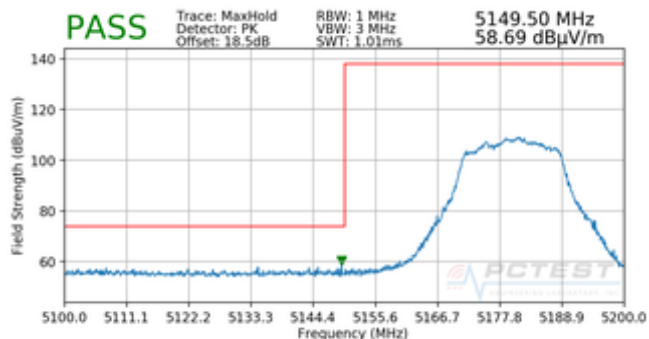
Plot 7-78. Radiated Lower Band Edge Plot (Peak – UNII Band 1)
