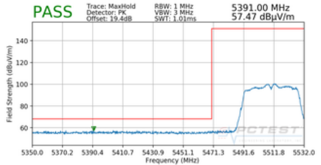
Plot 7-57. Radiated Lower Band Edge Plot (Peak – UNII Band 2C)
