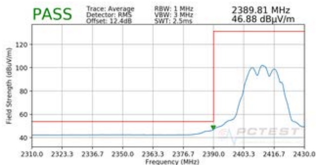
Plot 7-107. Radiated Restricted Band Edge Measurement CDD with WCP (Average)
