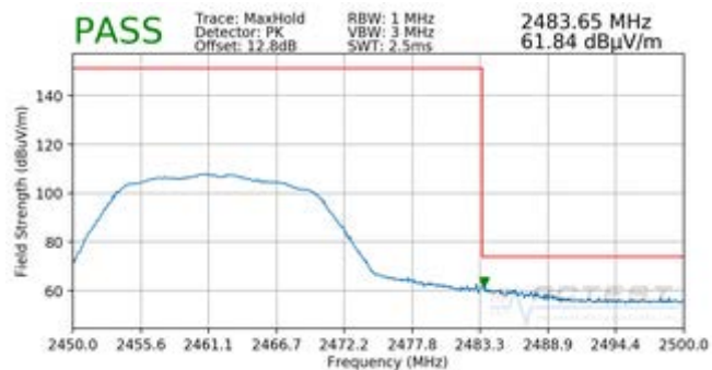
Plot 7-86. Radiated Restricted Upper Band Edge Measurement SISO ANT2 (Peak)
