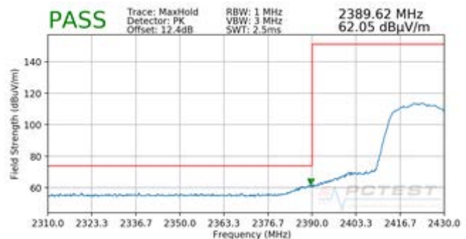
Plot 7-102. Radiated Restricted Lower Band Edge Measurement CDD (Peak)
