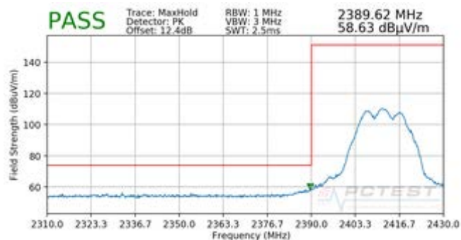
Plot 7-108. Radiated Restricted Band Edge Measurement CDD with WCP (Peak)
