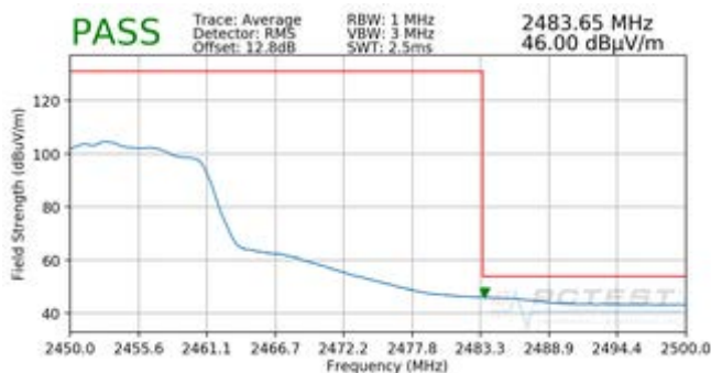
Plot 7-93. Radiated Restricted Upper Band Edge Measurement MIMO (Average)
