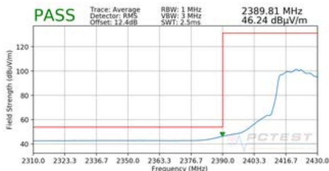
Plot 7-81. Radiated Restricted Lower Band Edge Measurement SISO ANT2 (Average)
