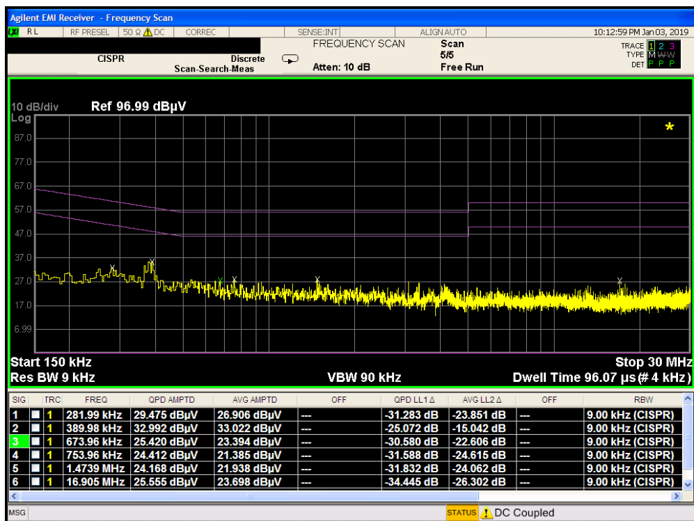
Plot 7-114. Line Conducted Plot with 802.11b (N) on WCP
