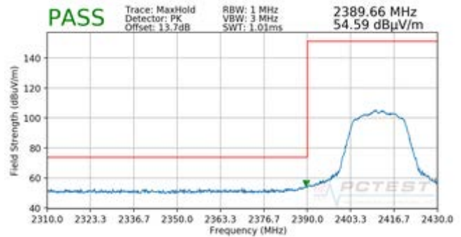
Plot 7-88. Radiated Restricted Band Edge Measurement SISO ANT2 with WCP (Peak)
