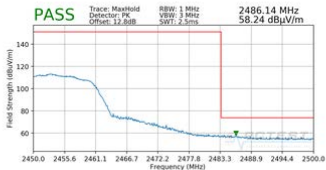
Plot 7-94. Radiated Restricted Upper Band Edge Measurement MIMO (Peak)
