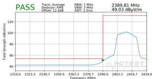
Plot 7-89. Radiated Restricted Lower Band Edge Measurement MIMO (Average)
