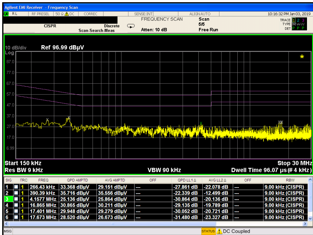
Plot 7-113. Line Conducted Plot with 802.11b (L1) on WCP
