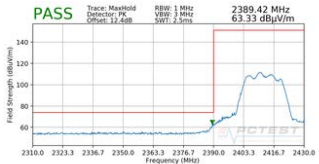
Plot 7-100. Radiated Restricted Lower Band Edge Measurement CDD (Peak)
