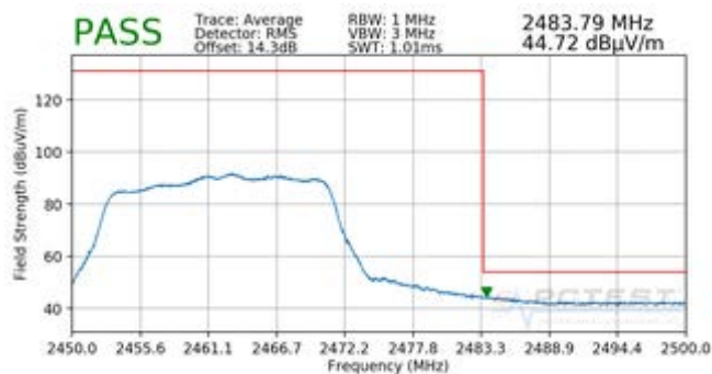
Plot 7-97. Radiated Restricted Band Edge Measurement MIMO with WCP (Average)
