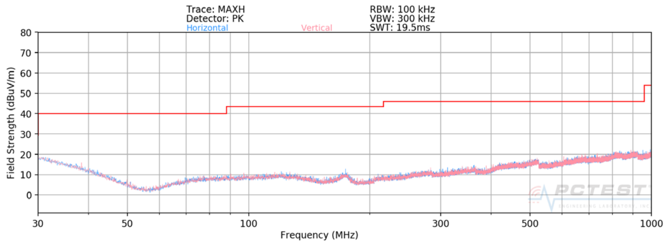
Plot 7-109. Radiated Spurious Plot below 1GHz SISO ANT1
