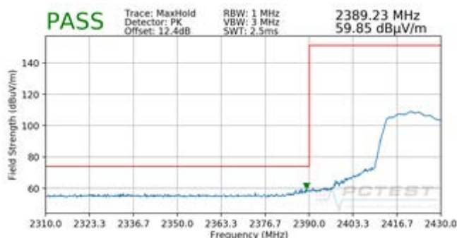
Plot 7-82. Radiated Restricted Lower Band Edge Measurement SISO ANT2 (Peak)
