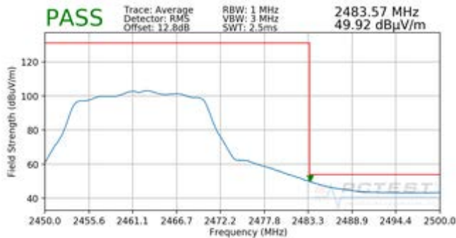
Plot 7-105. Radiated Restricted Upper Band Edge Measurement CDD (Average)
