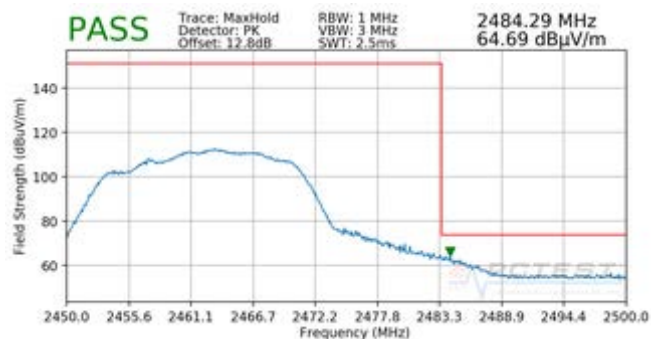
Plot 7-96. Radiated Restricted Upper Band Edge Measurement MIMO (Peak)
