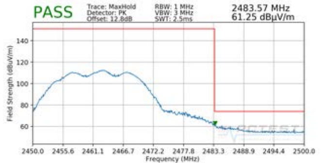
Plot 7-106. Radiated Restricted Upper Band Edge Measurement CDD (Peak)
