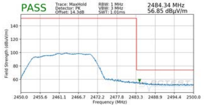
Plot 7-78. Radiated Restricted Band Edge Measurement SISO ANT1 with WCP (Peak)
