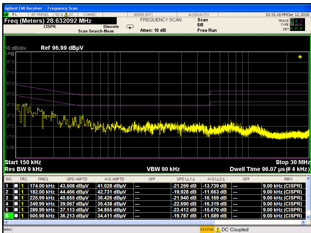
Plot 7-112. Line Conducted Plot with 802.11b (N)
