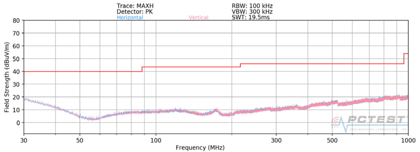
Plot 7-110. Radiated Spurious Plot below 1GHz SISO ANT2
