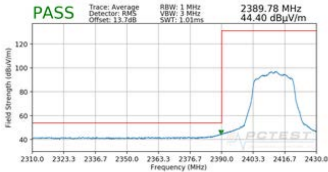
Plot 7-87. Radiated Restricted Band Edge Measurement SISO ANT2 with WCP (Average)
