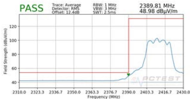
Plot 7-99. Radiated Restricted Lower Band Edge Measurement CDD (Average)
