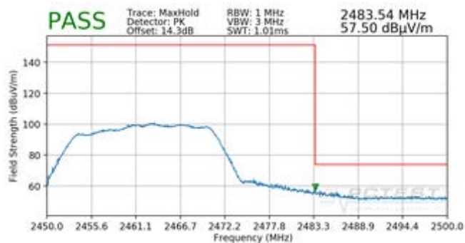
Plot 7-98. Radiated Restricted Band Edge Measurement MIMO with WCP (Peak)
