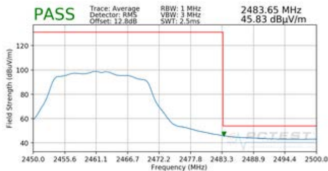
Plot 7-85. Radiated Restricted Upper Band Edge Measurement SISO ANT2 (Average)
