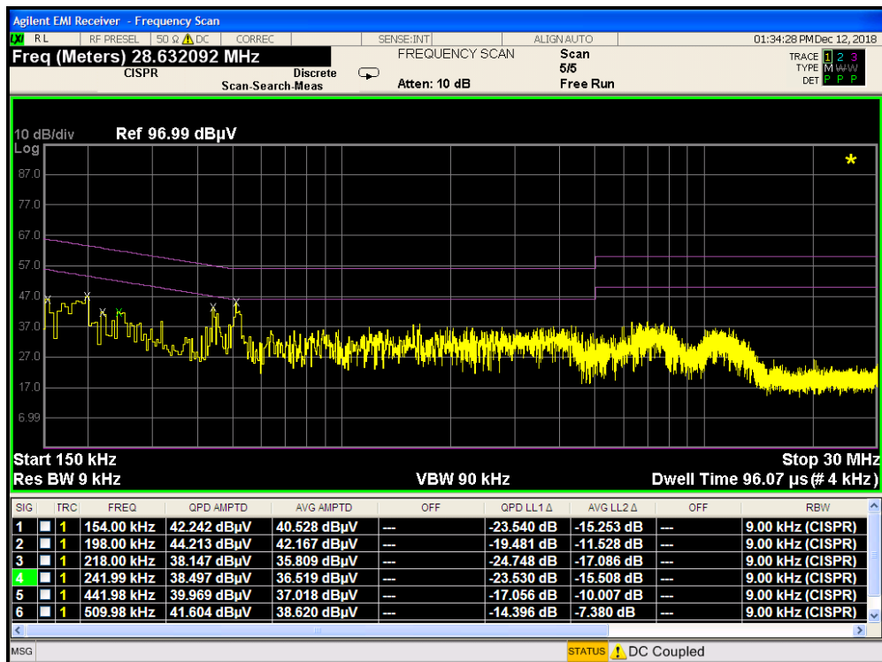
Plot 7-111. Line Conducted Plot with 802.11b (L1)
