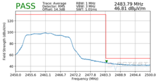
Plot 7-27. Radiated Restricted Band Edge Measurement SISO ANT2 with WCP (Average)
