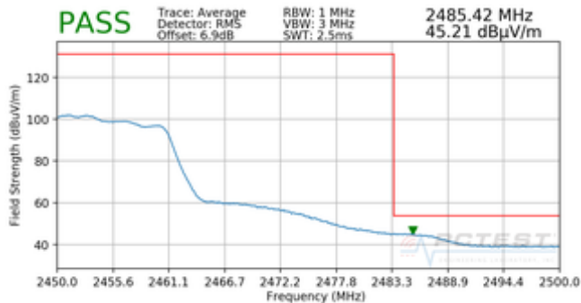
Plot 7-33. Radiated Restricted Upper Band Edge Measurement MIMO (Average)
