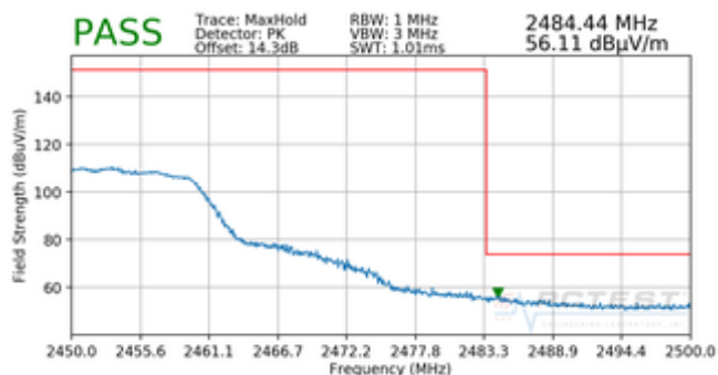
Plot 7-24. Radiated Restricted Upper Band Edge Measurement SISO ANT2 (Peak)
