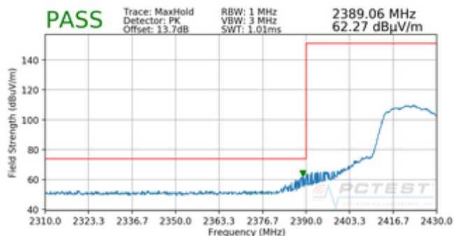
Plot 7-22. Radiated Restricted Lower Band Edge Measurement SISO ANT2 (Peak)
