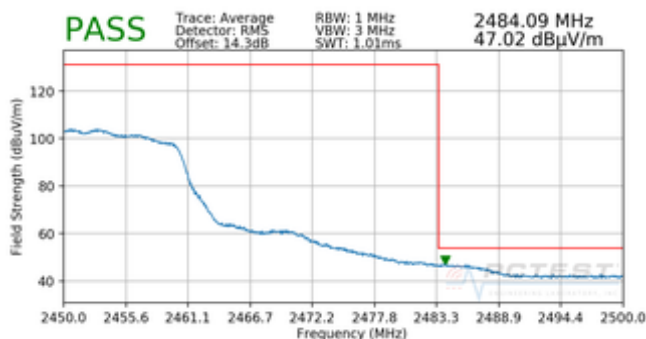
Plot 7-43. Radiated Restricted Upper Band Edge Measurement CDD (Average)
