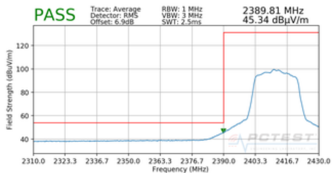
Plot 7-37. Radiated Restricted Band Edge Measurement MIMO with WCP (Average)
