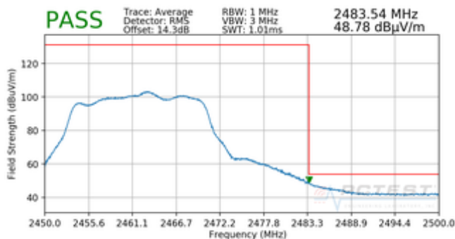
Plot 7-45. Radiated Restricted Upper Band Edge Measurement CDD (Average)
