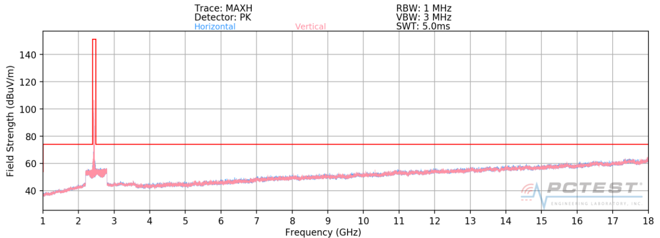
Plot 7-6. Radiated Spurious Plot above 1GHz SISO ANT2 (802.11b – Ch. 6)
