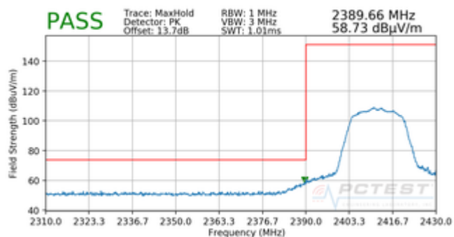
Plot 7-20. Radiated Restricted Lower Band Edge Measurement SISO ANT2 (Peak)
