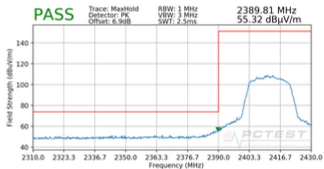
Plot 7-38. Radiated Restricted Band Edge Measurement MIMO with WCP (Peak)
