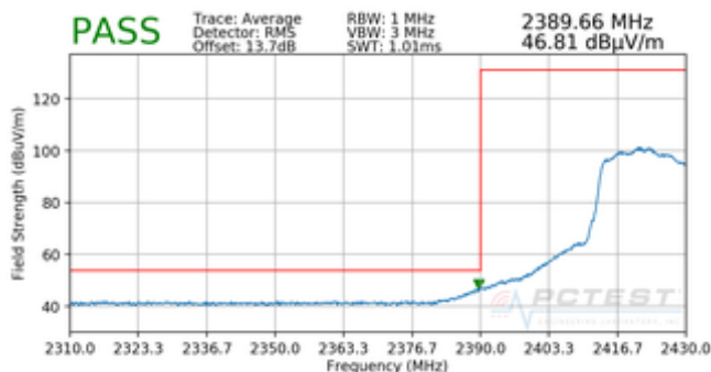
Plot 7-21. Radiated Restricted Lower Band Edge Measurement SISO ANT2 (Average)
