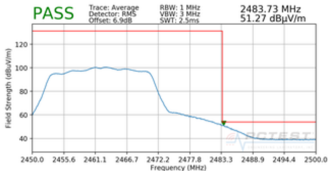
Plot 7-35. Radiated Restricted Upper Band Edge Measurement MIMO (Average)
