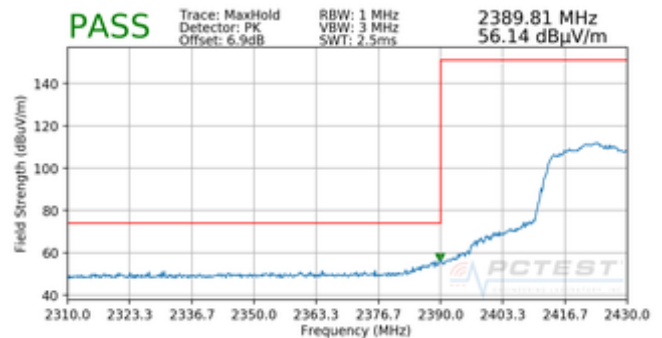
Plot 7-32. Radiated Restricted Lower Band Edge Measurement MIMO (Peak)
