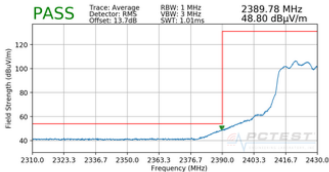
Plot 7-41. Radiated Restricted Lower Band Edge Measurement CDD (Average)
