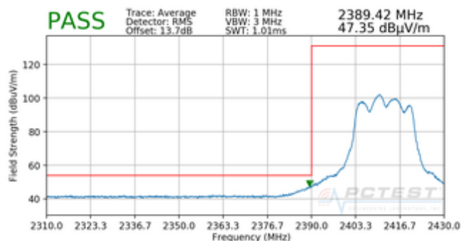
Plot 7-47. Radiated Restricted Band Edge Measurement CDD with WCP (Average)
