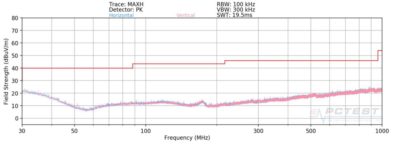
Plot 7-50. Radiated Spurious Plot below 1GHz SISO ANT2
