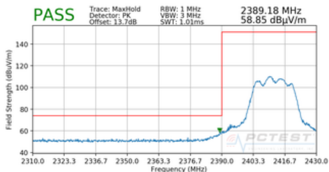
Plot 7-48. Radiated Restricted Band Edge Measurement CDD with WCP (Peak)
