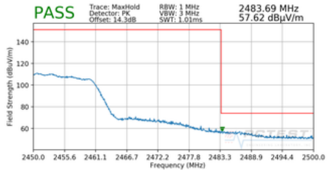
Plot 7-14. Radiated Restricted Upper Band Edge Measurement SISO ANT1 (Peak)
