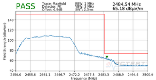
Plot 7-36. Radiated Restricted Upper Band Edge Measurement MIMO (Peak)
