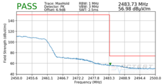
Plot 7-34. Radiated Restricted Upper Band Edge Measurement MIMO (Peak)
