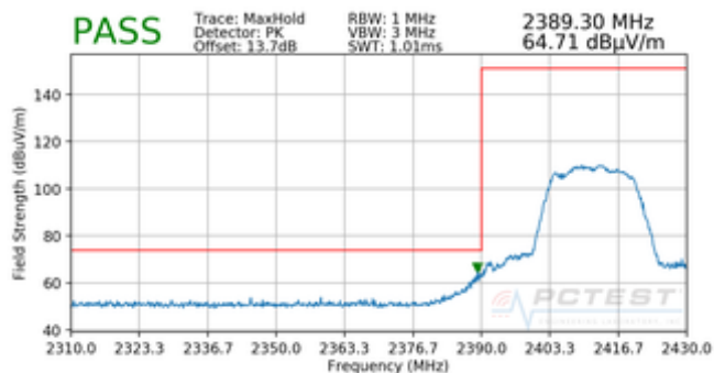
Plot 7-40. Radiated Restricted Lower Band Edge Measurement CDD (Peak)
