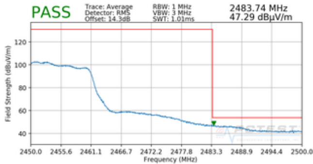
Plot 7-13. Radiated Restricted Upper Band Edge Measurement SISO ANT1 (Average)
