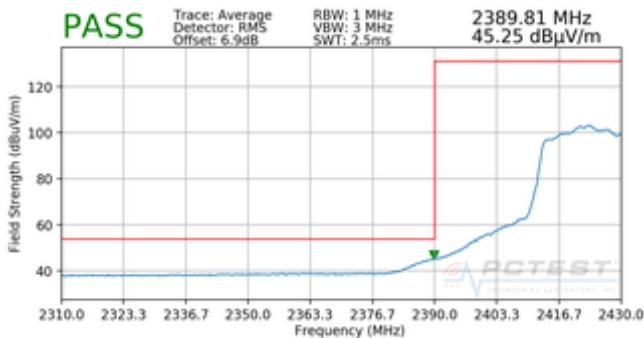
Plot 7-31. Radiated Restricted Lower Band Edge Measurement MIMO (Average)
