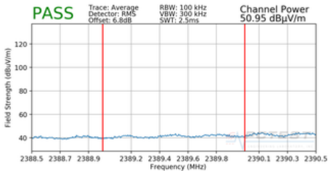
Plot 7-29. Radiated Restricted Lower Band Edge Measurement MIMO (Average)
