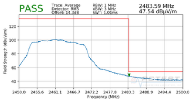
Plot 7-25. Radiated Restricted Upper Band Edge Measurement SISO ANT2 (Average)
