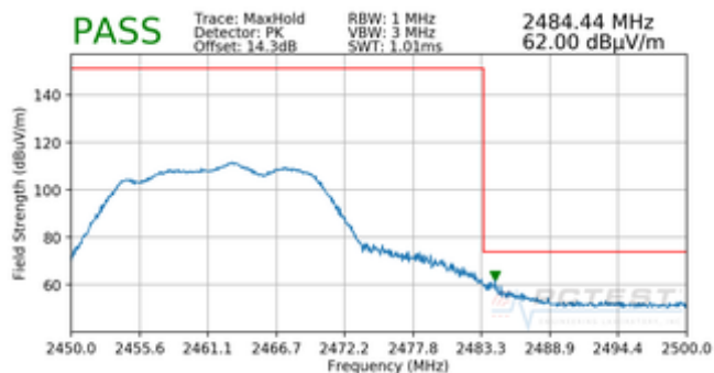
Plot 7-46. Radiated Restricted Upper Band Edge Measurement CDD (Peak)
