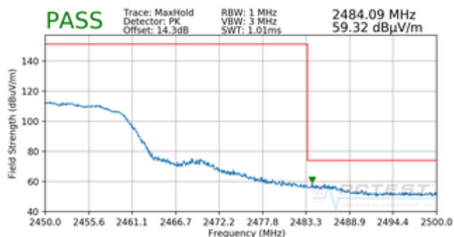
Plot 7-44. Radiated Restricted Upper Band Edge Measurement CDD (Peak)
