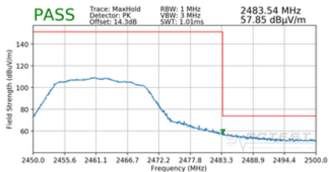
Plot 7-26. Radiated Restricted Upper Band Edge Measurement SISO ANT2 (Peak)
