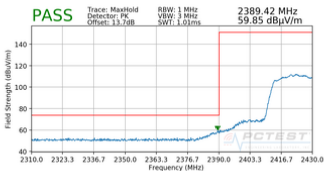
Plot 7-12. Radiated Restricted Lower Band Edge Measurement SISO ANT1 (Peak)
