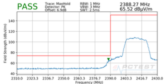
Plot 7-30. Radiated Restricted Lower Band Edge Measurement MIMO (Peak)
