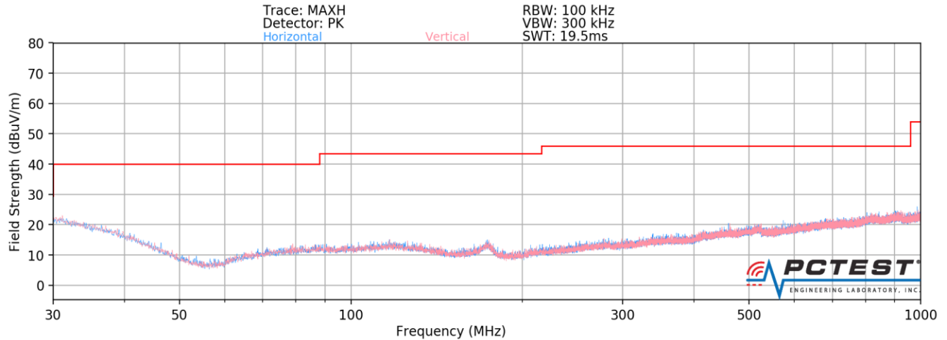
Plot 7-49. Radiated Spurious Plot below 1GHz SISO ANT1
