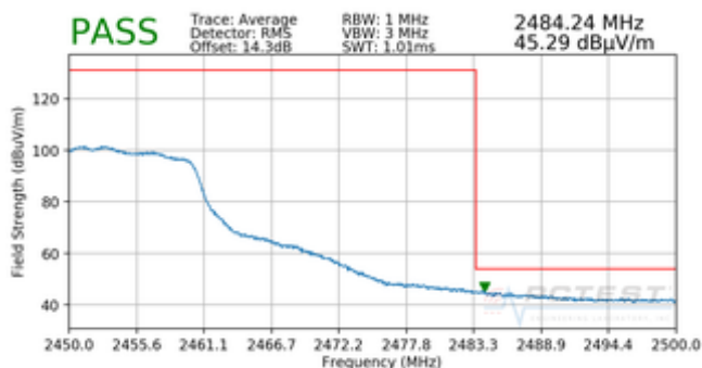
Plot 7-23. Radiated Restricted Upper Band Edge Measurement SISO ANT2 (Average)
