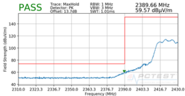
Plot 7-42. Radiated Restricted Lower Band Edge Measurement CDD (Peak)
