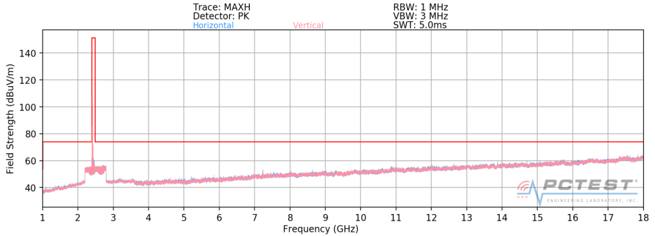
Plot 7-5. Radiated Spurious Plot above 1GHz SISO ANT2 (802.11b – Ch. 1)
