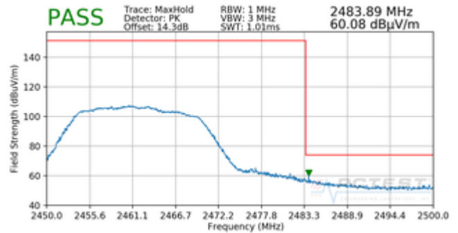
Plot 7-28. Radiated Restricted Band Edge Measurement SISO ANT2 with WCP (Peak)
