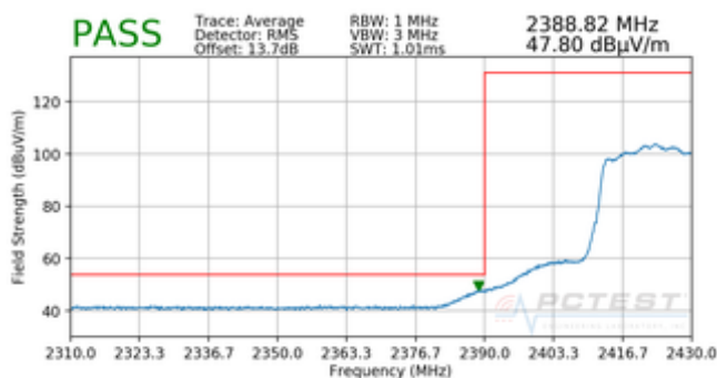
Plot 7-11. Radiated Restricted Lower Band Edge Measurement SISO ANT1 (Average)
