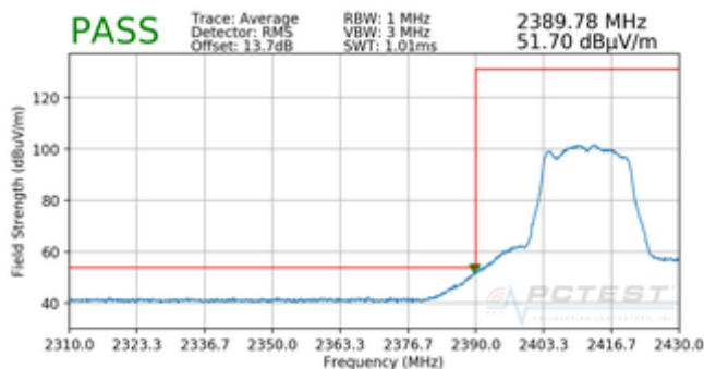
Plot 7-39. Radiated Restricted Lower Band Edge Measurement CDD (Average)
