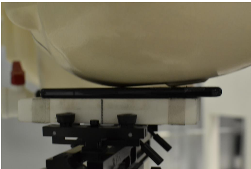
SAR Test Setup Photo 10: Left Cheek Position 3
