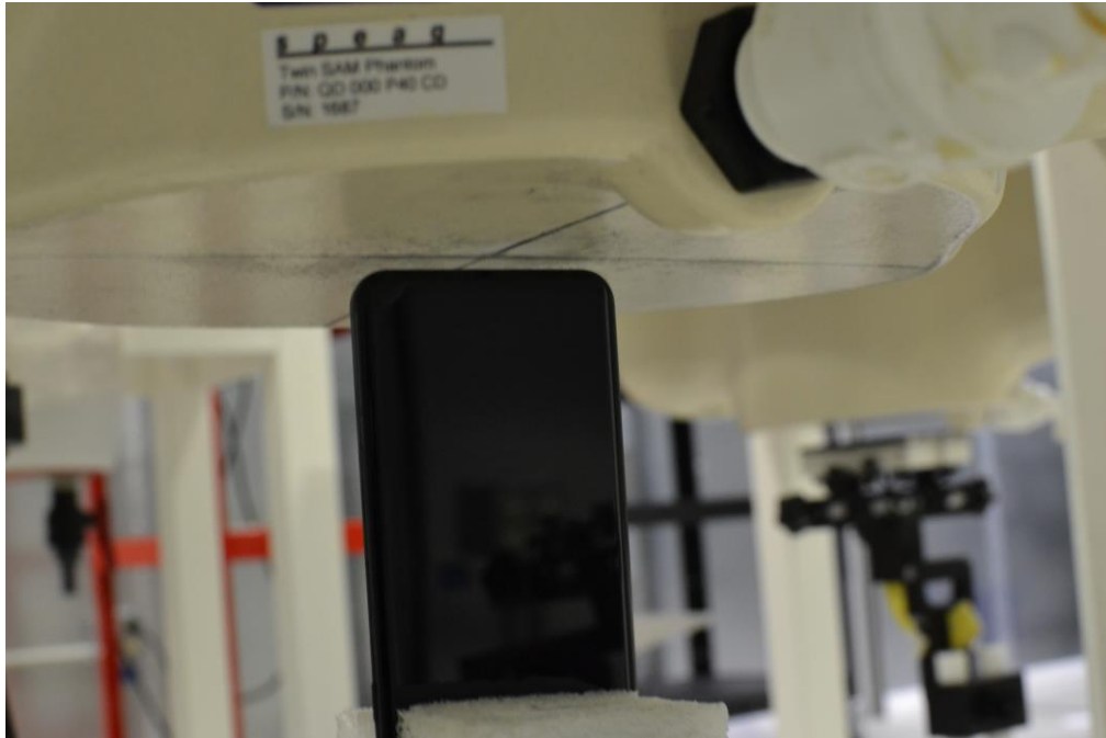
SAR Test Setup Photo 19: Bottom Edge at 3 mm
