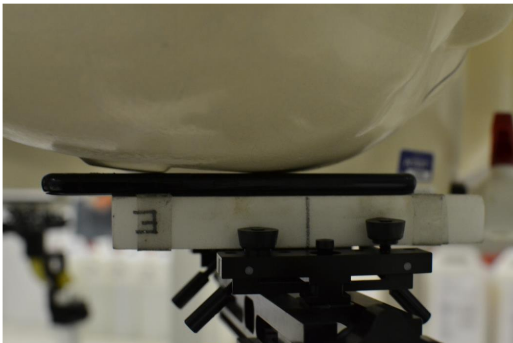
SAR Test Setup Photo 5: Right Cheek Position 3
