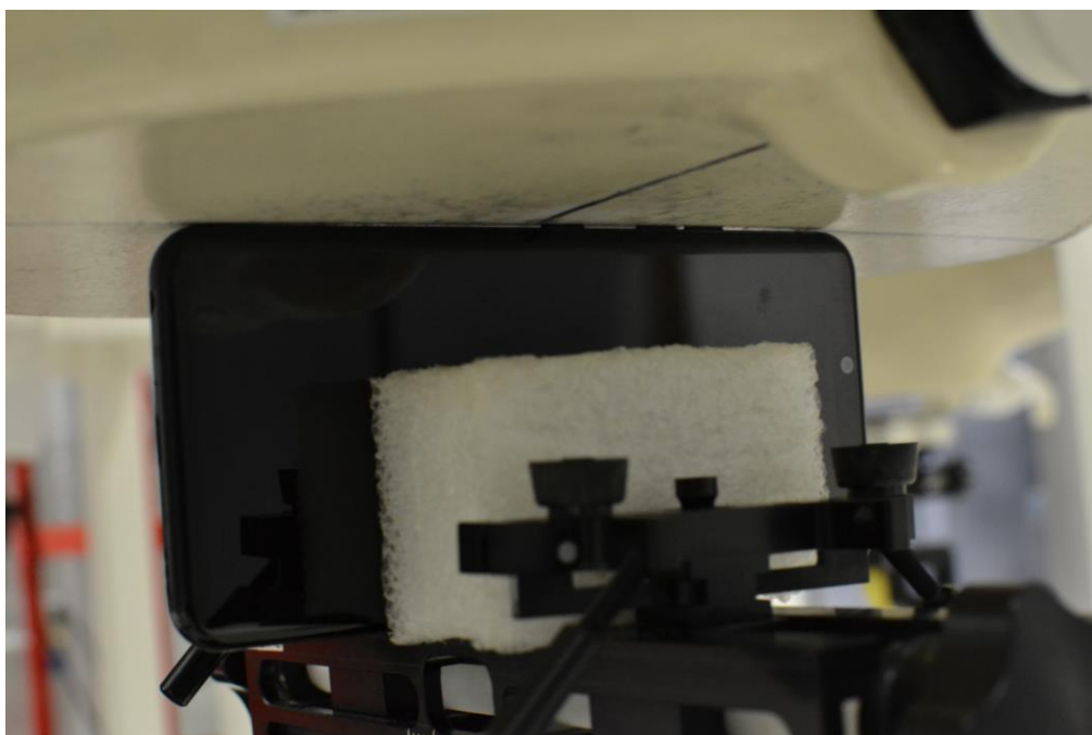
SAR Test Setup Photo 24: Left Edge at 0 mm
