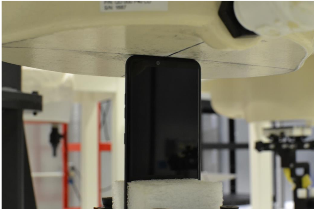
SAR Test Setup Photo 17: Top Edge at 0 mm
