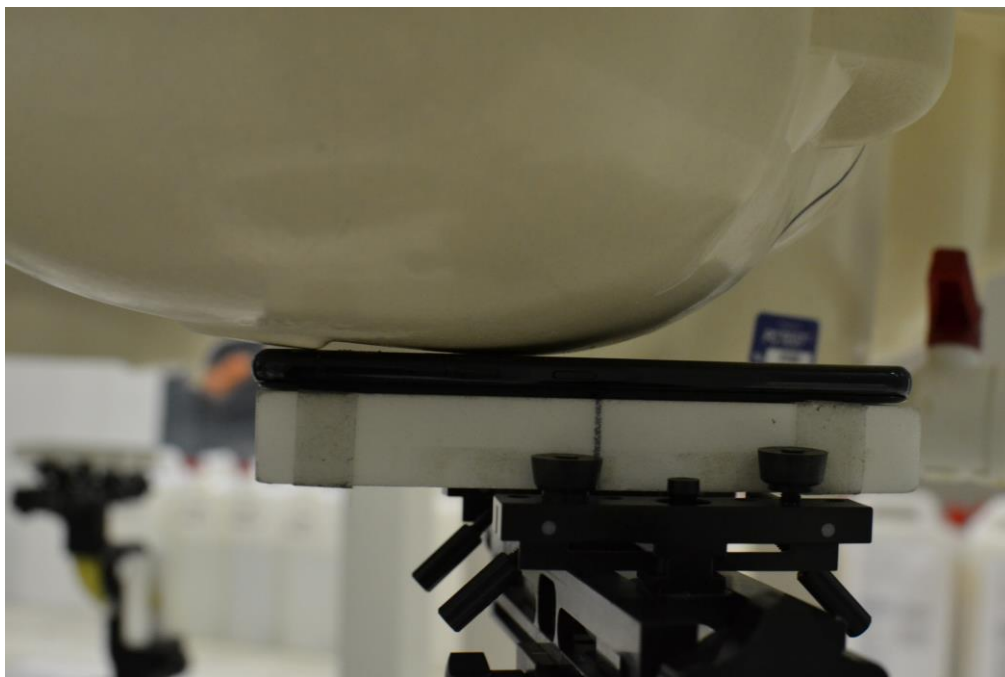
SAR Test Setup Photo 1: Right Cheek Position 1
