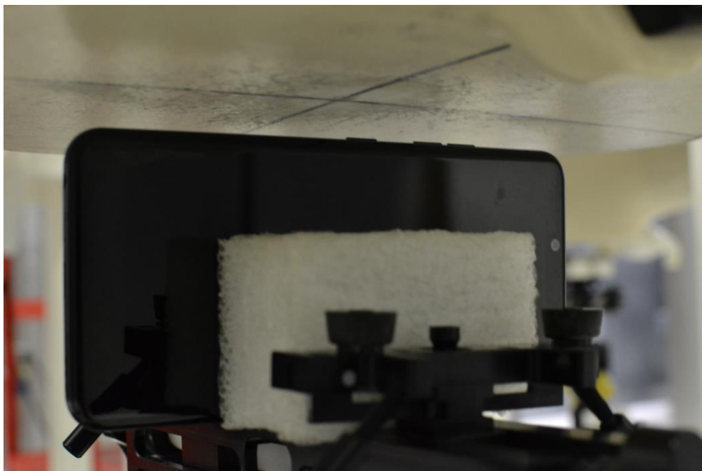
SAR Test Setup Photo 23: Left Edge at 10 mm
