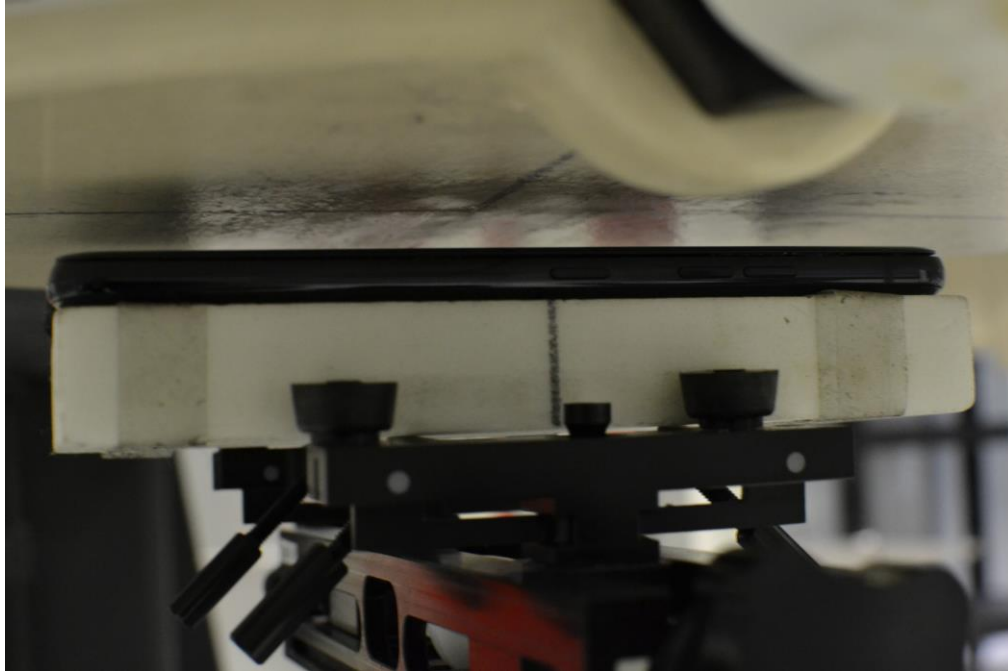
SAR Test Setup Photo 11: Back Side at 10 mm
