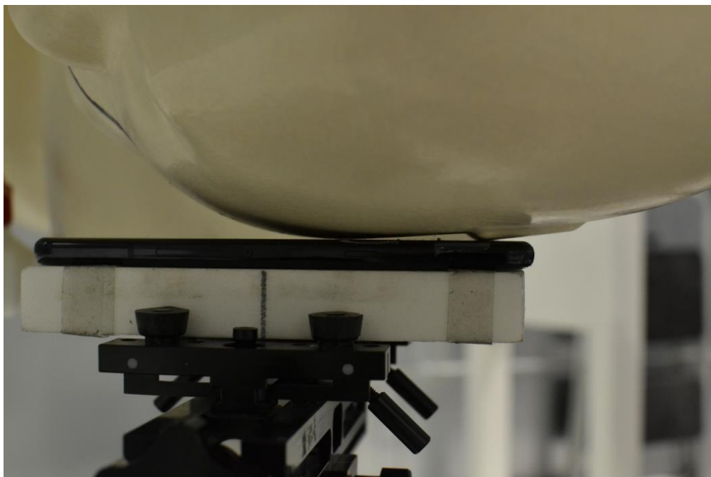
SAR Test Setup Photo 7: Left Cheek Position 1
