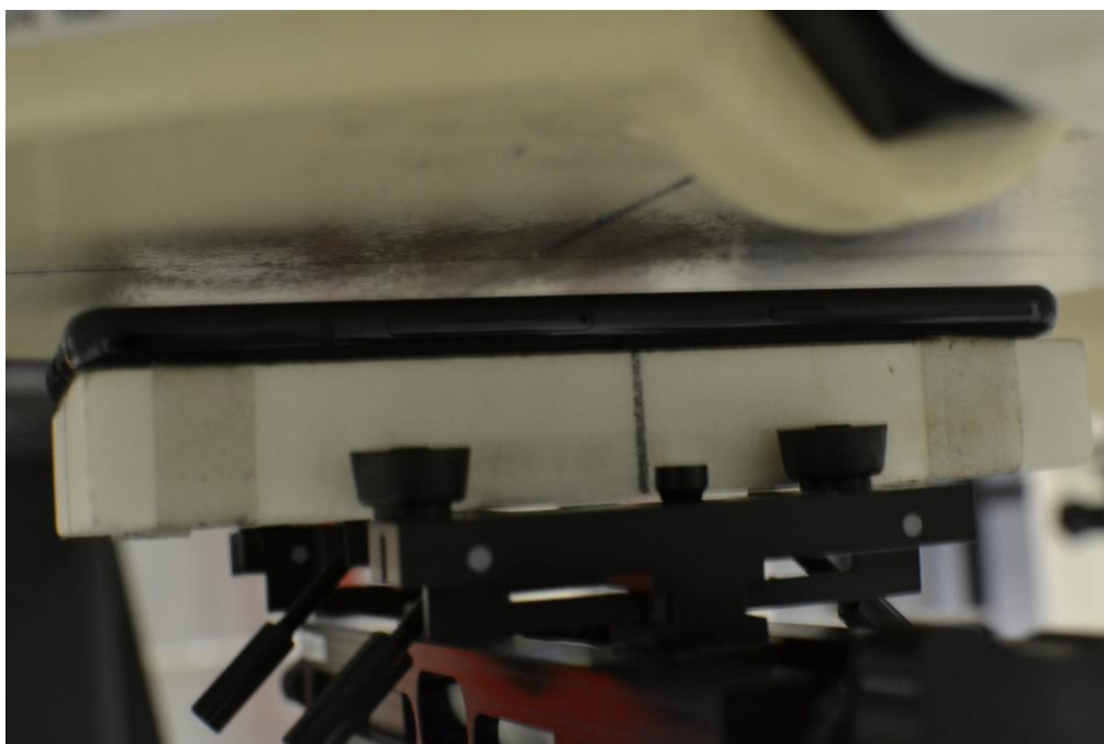
SAR Test Setup Photo 14: Front Side at 10 mm
