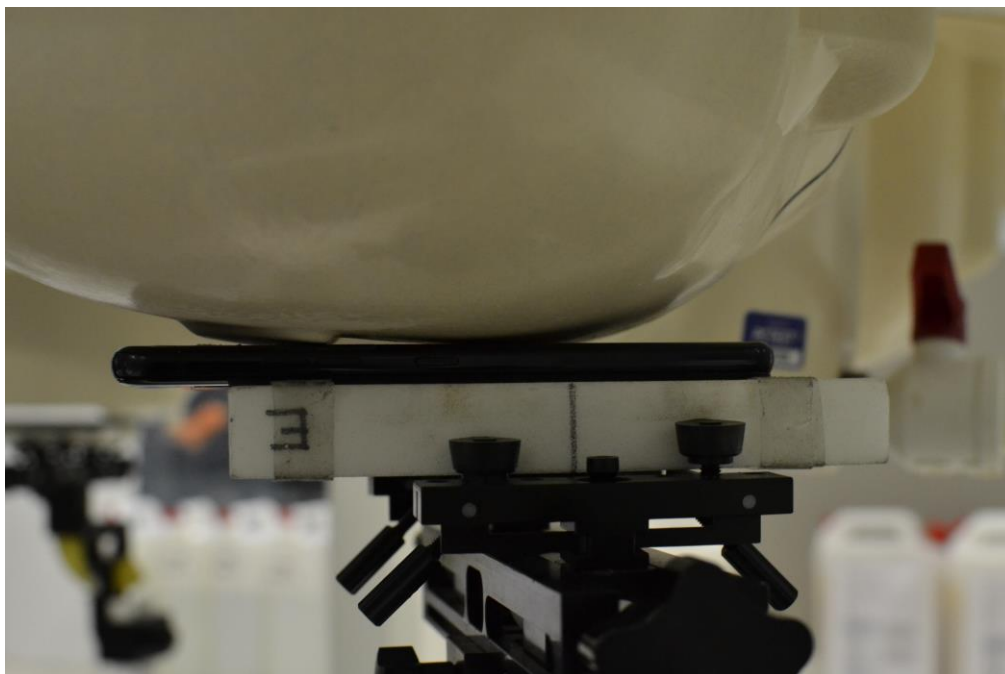
SAR Test Setup Photo 3: Right Cheek Position 2
