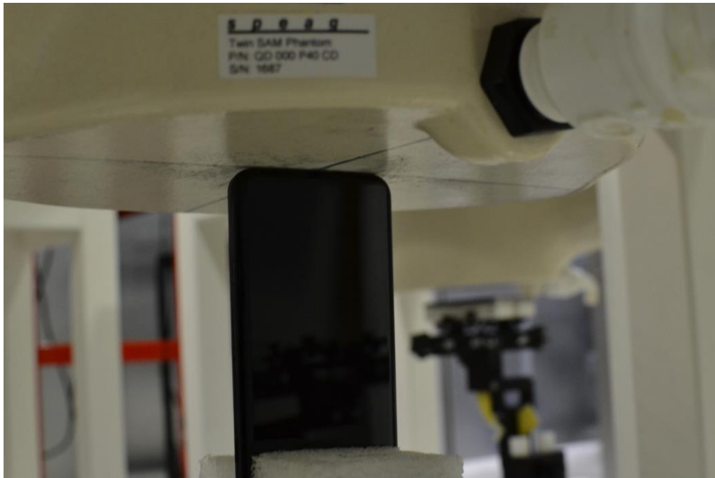
SAR Test Setup Photo 20: Bottom Edge at 0 mm
