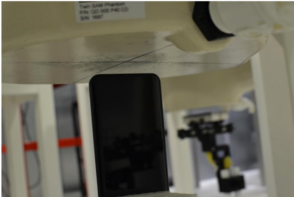
SAR Test Setup Photo 18: Bottom Edge at 10 mm
