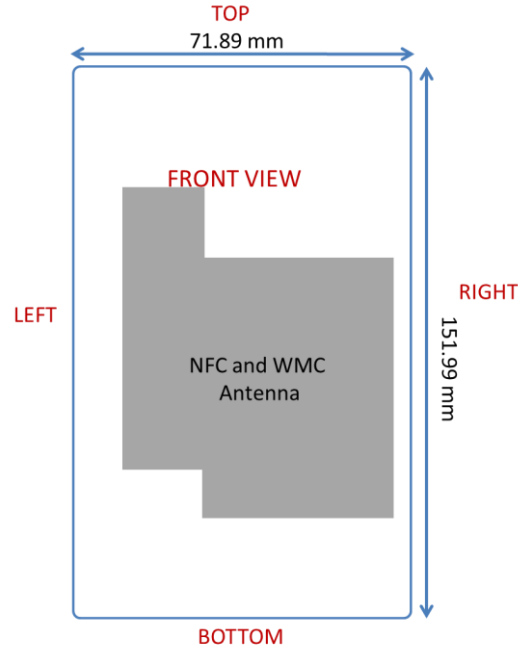
Figure F-2 NFC and WMC Antenna Locations
