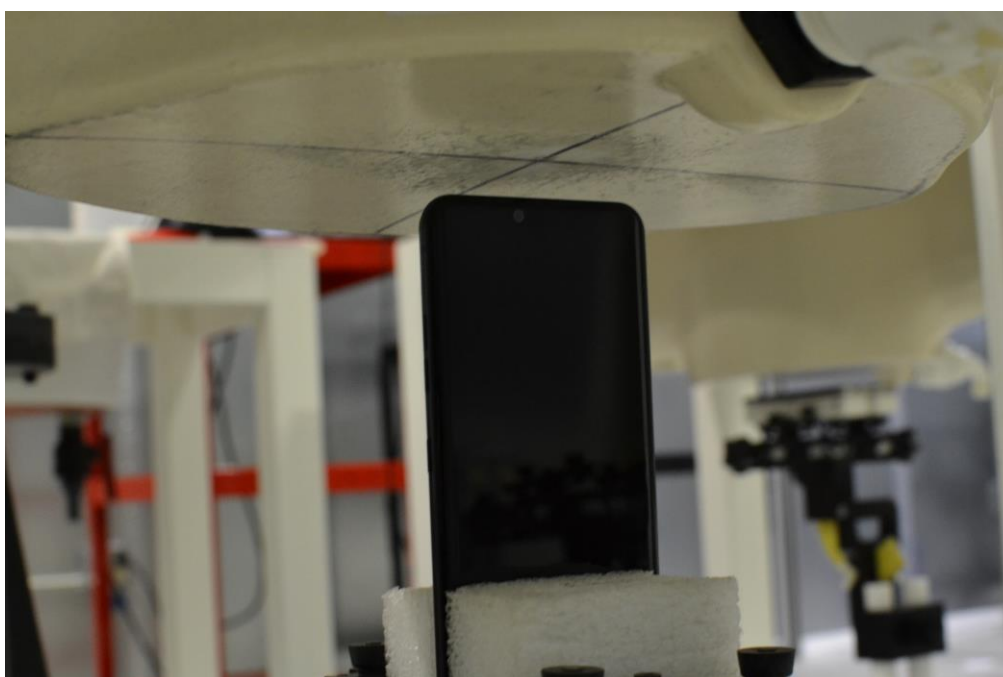
SAR Test Setup Photo 16: Top Edge at 10 mm
