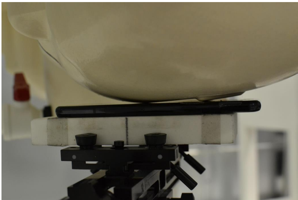
SAR Test Setup Photo 9: Left Cheek Position 2
