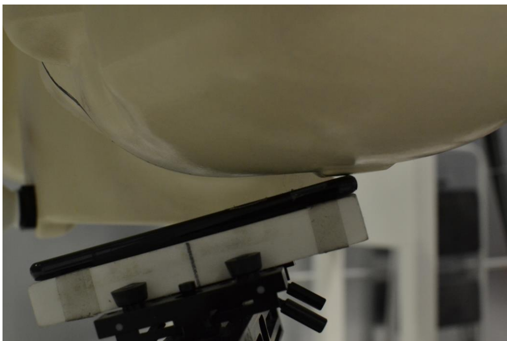
SAR Test Setup Photo 8: Left Tilt Position 1
