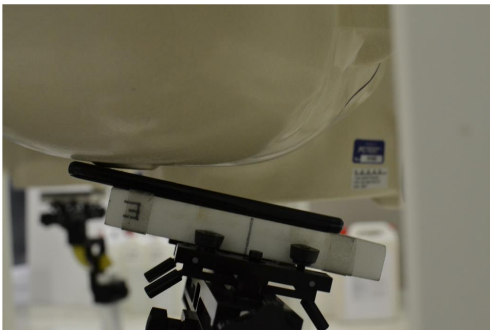
SAR Test Setup Photo 4: Right Tilt Position 2
