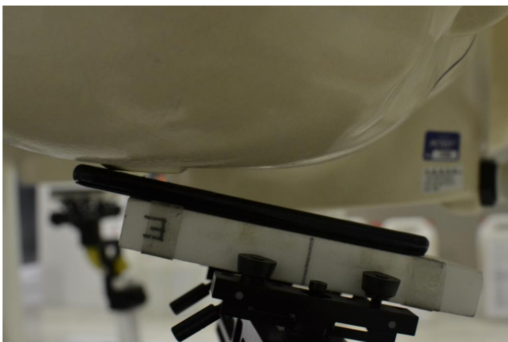
SAR Test Setup Photo 6: Right Tilt Position 3
