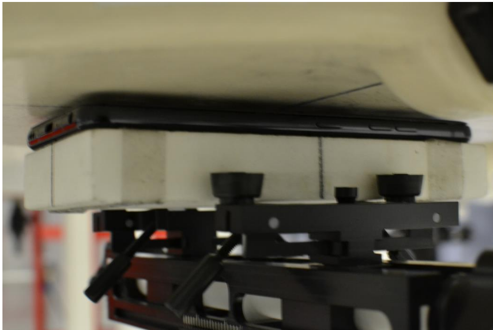
SAR Test Setup Photo 12: Back Side at 2 mm
