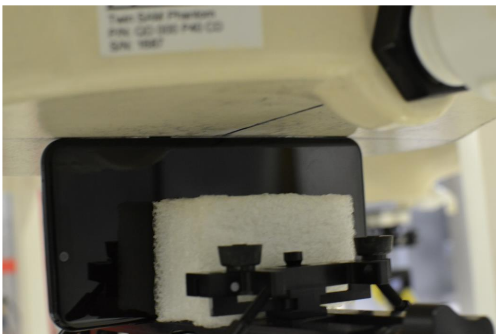
SAR Test Setup Photo 22: Right Edge at 0 mm
