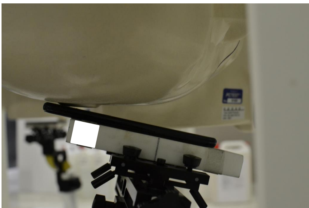
SAR Test Setup Photo 4: Right Tilt Additional Position 1
