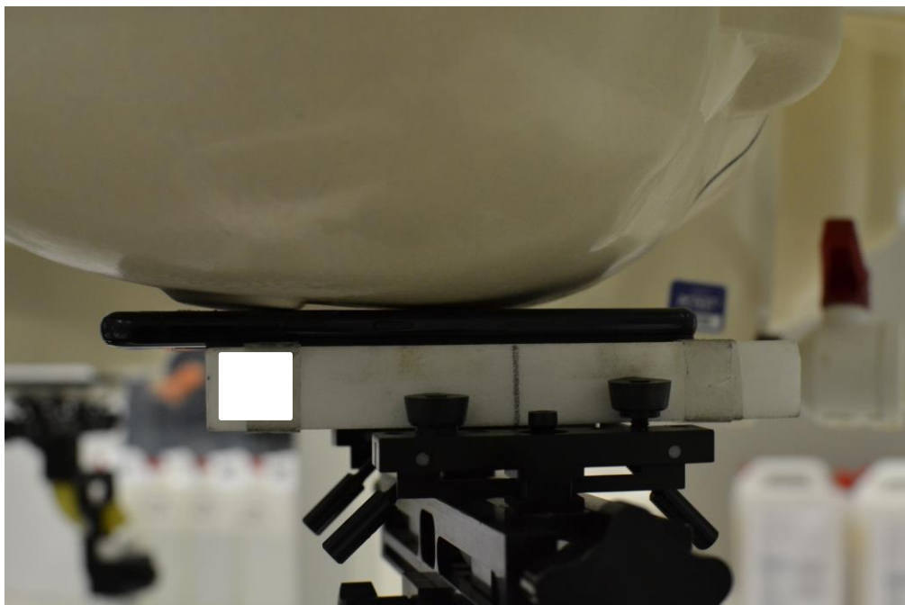
SAR Test Setup Photo 3: Right Cheek Additional Position 1
