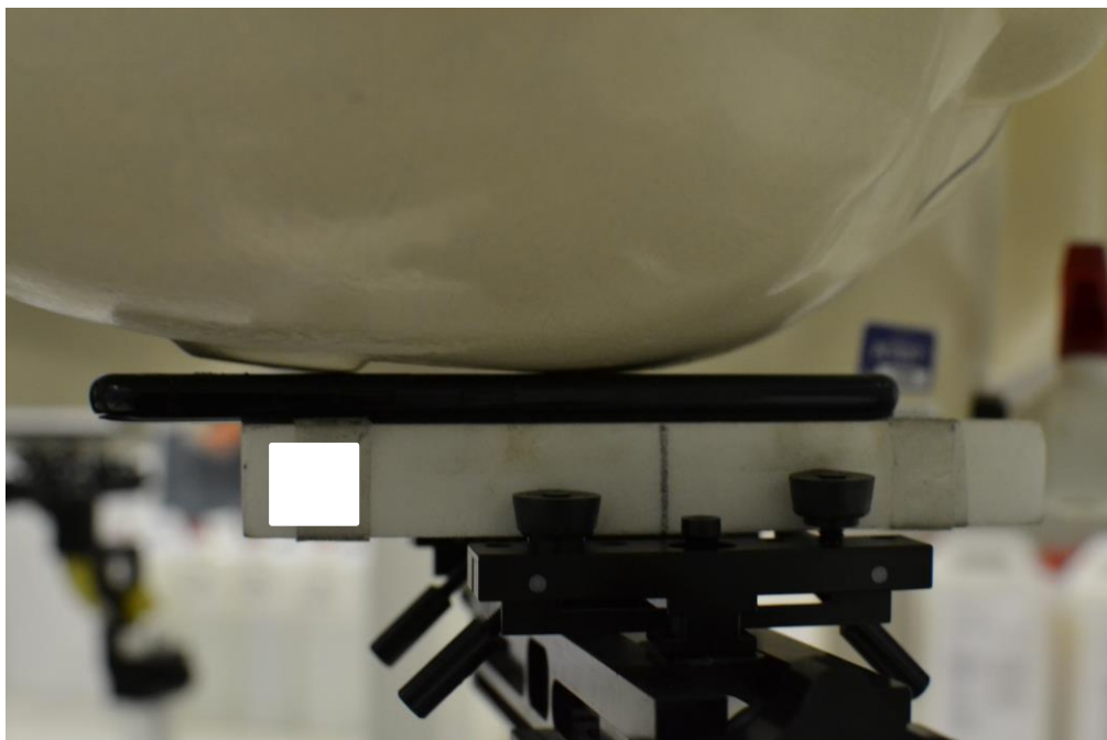
SAR Test Setup Photo 5: Right Cheek Additional Position 2
