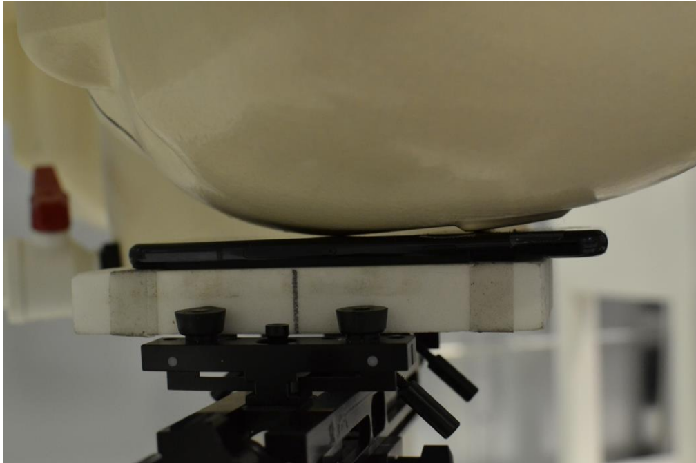
SAR Test Setup Photo 9: Left Cheek Additional Position 1
