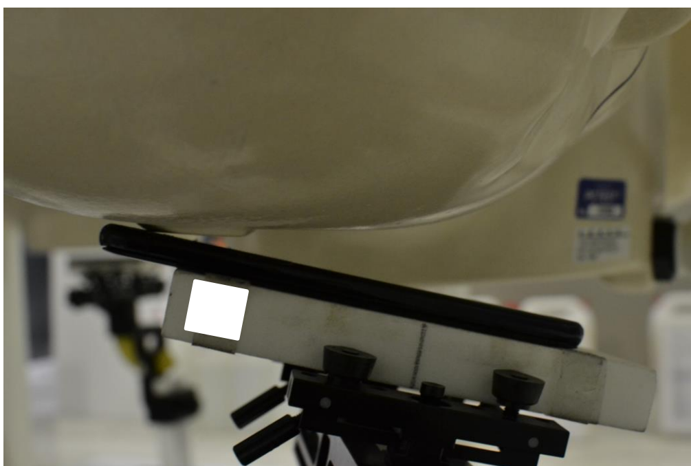
SAR Test Setup Photo 6: Right Tilt Additional Position 2
