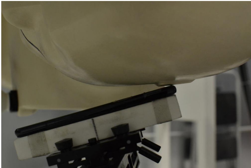
SAR Test Setup Photo 8: Left Tilt
