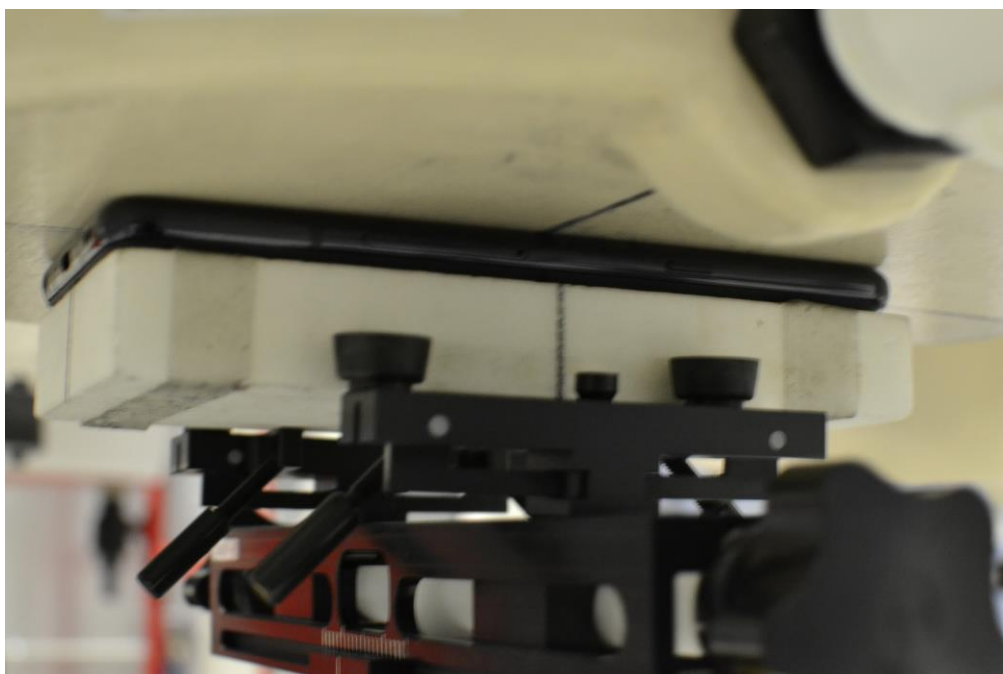
SAR Test Setup Photo 15: Front Side at 0 mm
