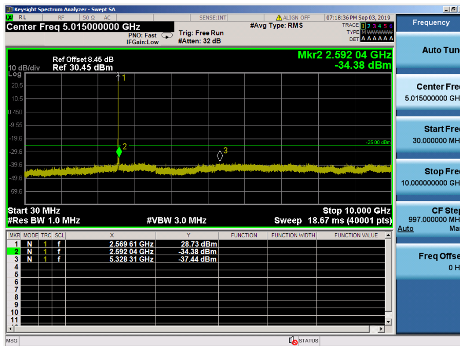
LTE Band 7 / 10MHz / 64QAM - RB Size/Offset (1/49) – High Channel
