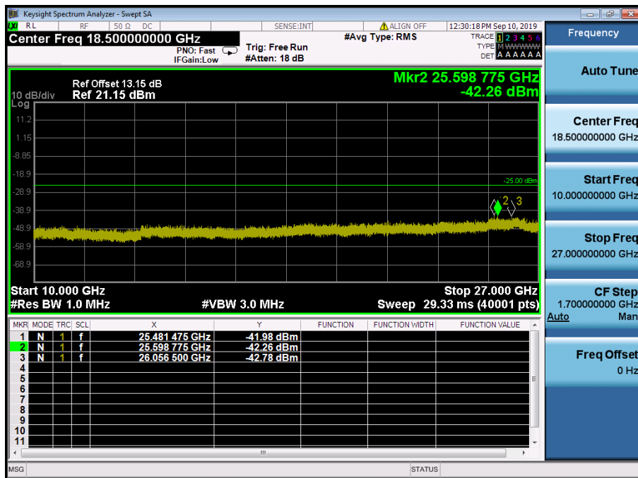
LTE Band 41 / 15MHz / 16QAM - RB Size/Offset (36/18) – High Channel
