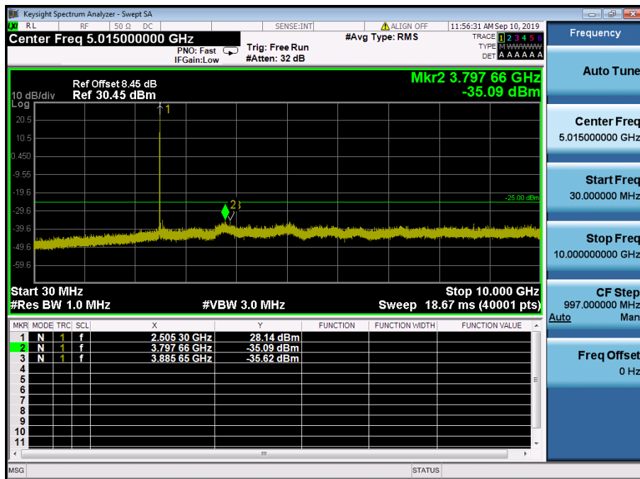
LTE Band 41 / 10MHz / 16QAM - RB Size/Offset (1/49) – Low Channel
