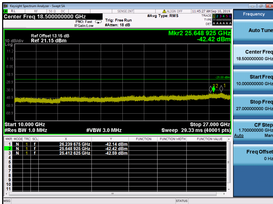
LTE Band 41 / 5MHz / 16QAM - RB Size/Offset (12/6) – Mid Channel
