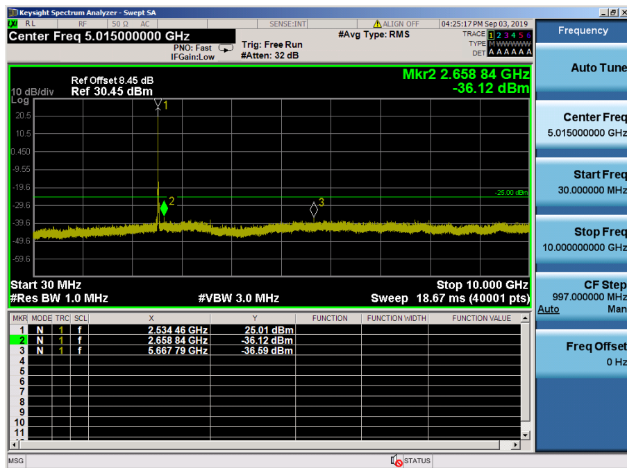
LTE Band 7 / 10MHz / 16QAM - RB Size/Offset (25/12) – Mid Channel
