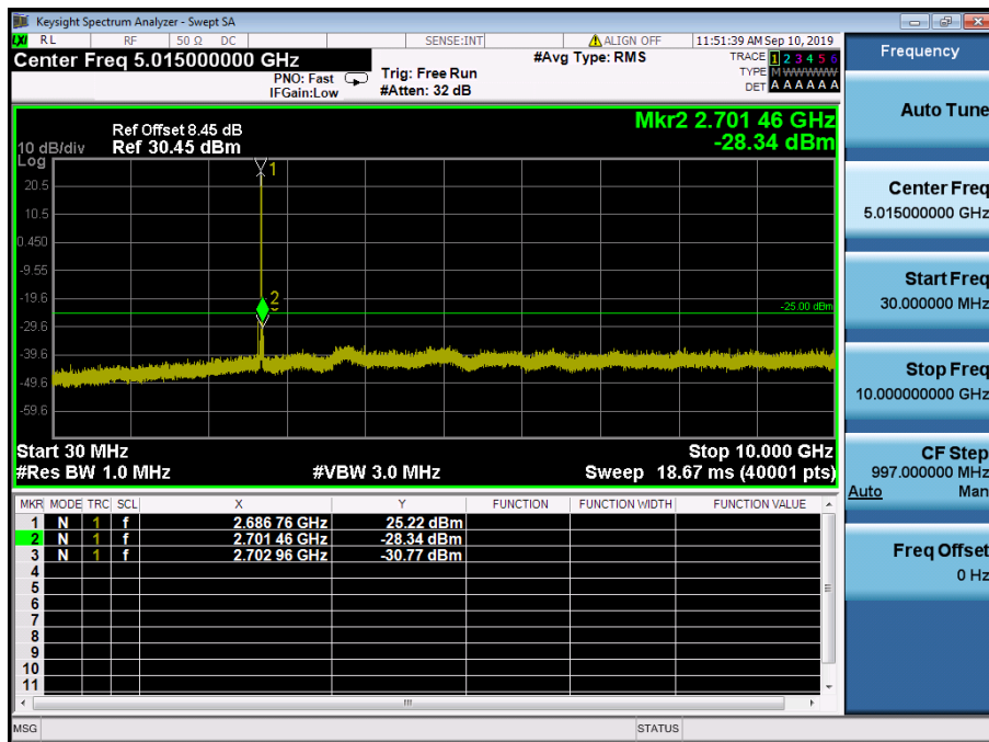
LTE Band 41 / 5MHz / 16QAM - RB Size/Offset (12/6) – High Channel
