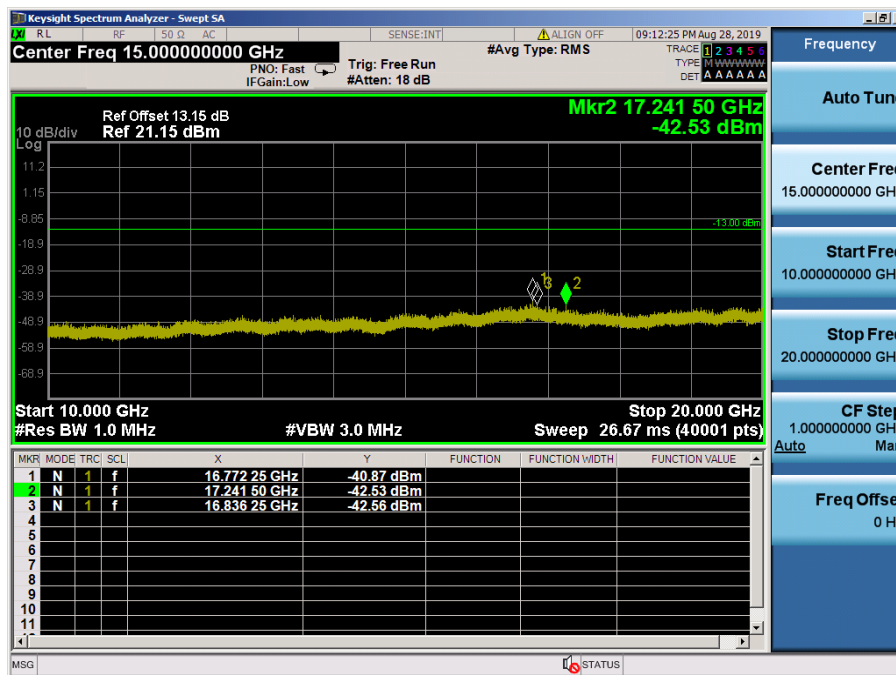
LTE Band 2 / 1.4MHz / QPSK - RB Size/Offset (1/5) – Low Channel
