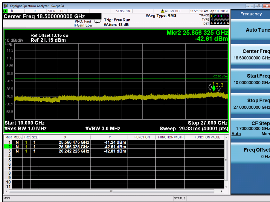
LTE Band 41 / 20MHz / QPSK - RB Size/Offset (50/0) – Mid Channel
