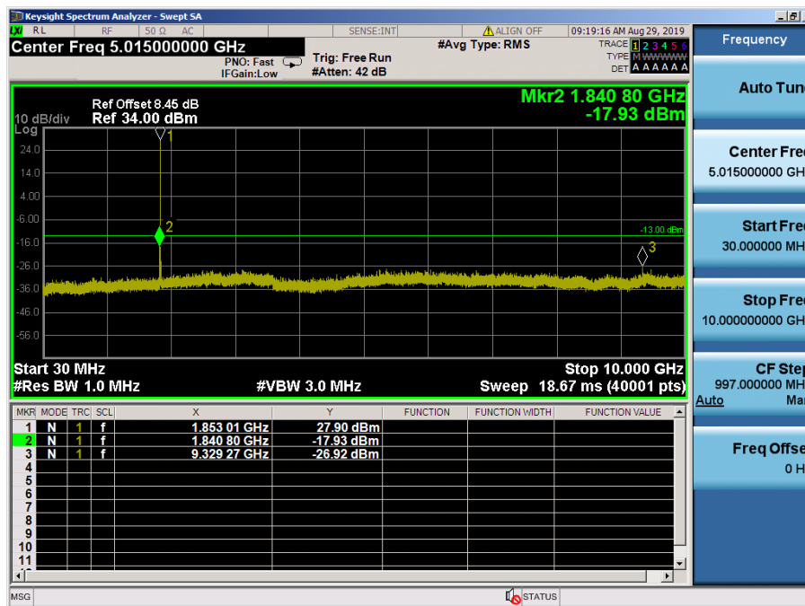
LTE Band 2 / 3MHz / 16QAM - RB Size/Offset (1/14) – Low Channel
