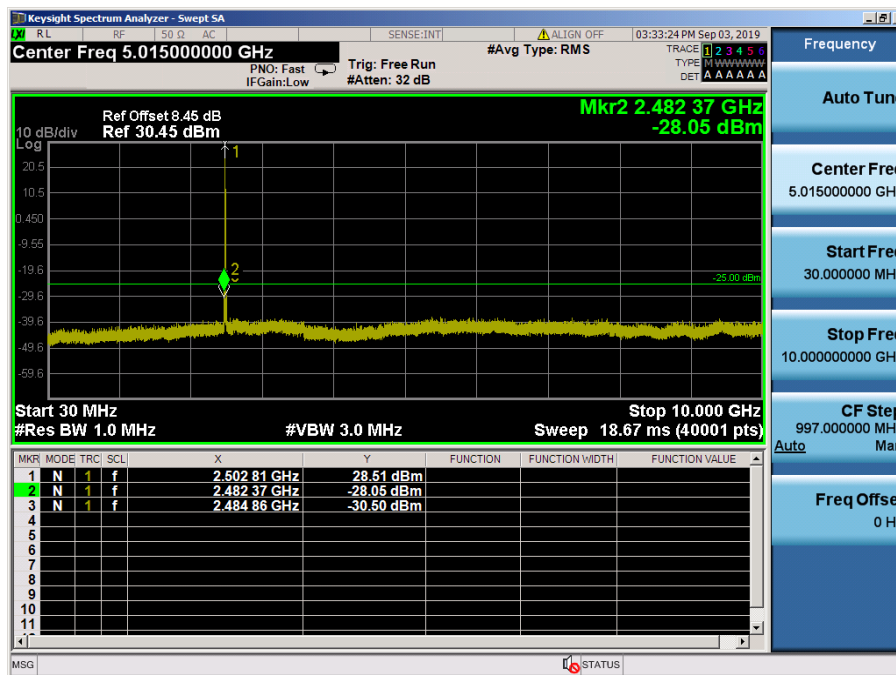
LTE Band 7 / 5MHz / 16QAM - RB Size/Offset (1/12) – Low Channel
