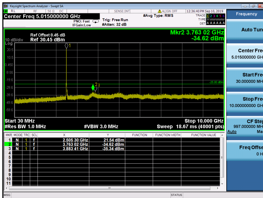
LTE Band 41 / 20MHz / 16QAM - RB Size/Offset (50/25) – Low Channel
