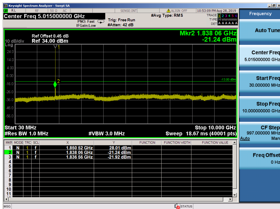
LTE Band 2 / 5MHz / QPSK - RB Size/Offset (1/0) – Low Channel
