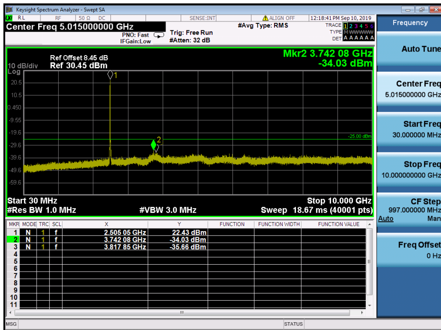
LTE Band 41 / 15MHz / 16QAM - RB Size/Offset (36/39) – Low Channel
