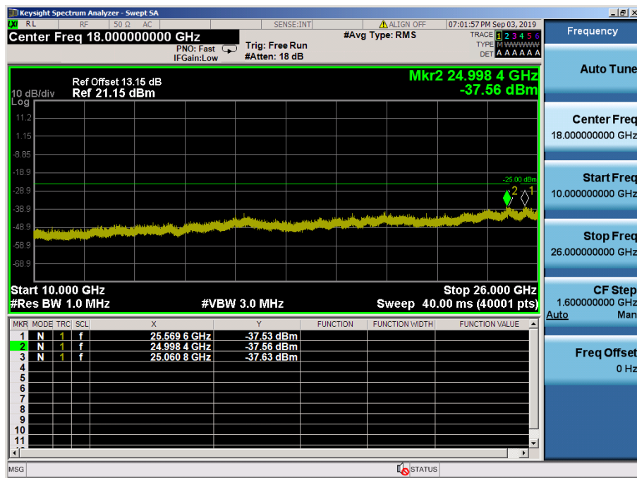
LTE Band 7 / 10MHz / 64QAM - RB Size/Offset (50/0) – Low Channel
