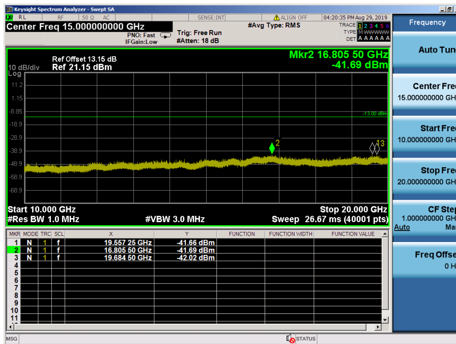
LTE Band 2 / 1.4MHz / 64QAM - RB Size/Offset (3/3) – Mid Channel
