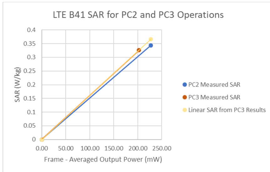
Figure 14-4 LTE Band 41 UCLA Body-Worn Linearity
