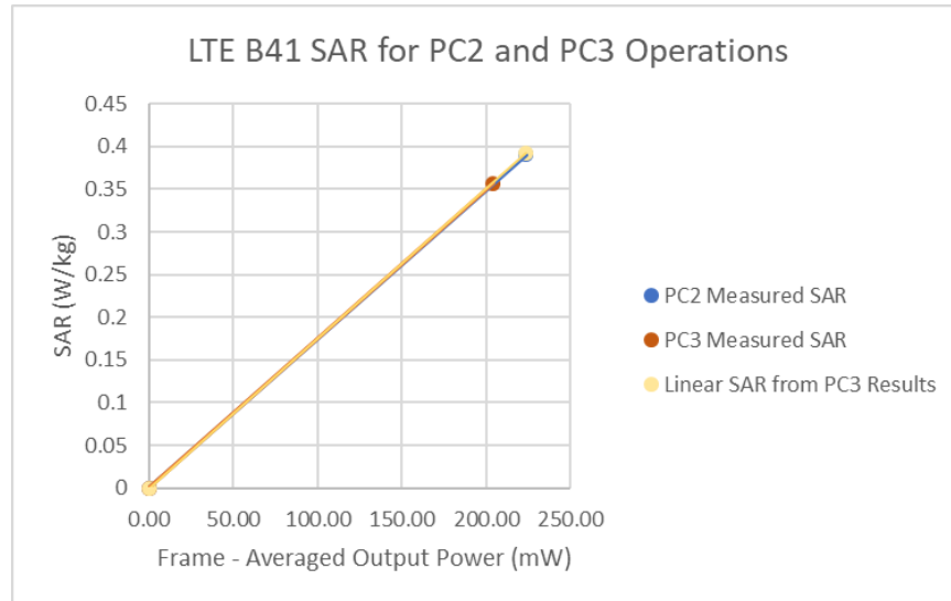
Figure 14-5 LTE Band 41 Standalone Hotspot Linearity
