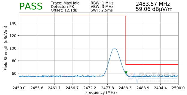
Plot 7-6. Radiated Restricted Upper Band Edge Measurement with Dual Display (Peak)
