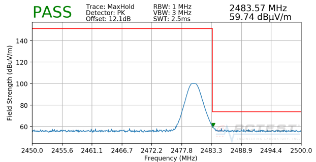
Plot 7-8. Radiated Restricted Upper Band Edge Measurement with WCP and Dual Display (Peak)
