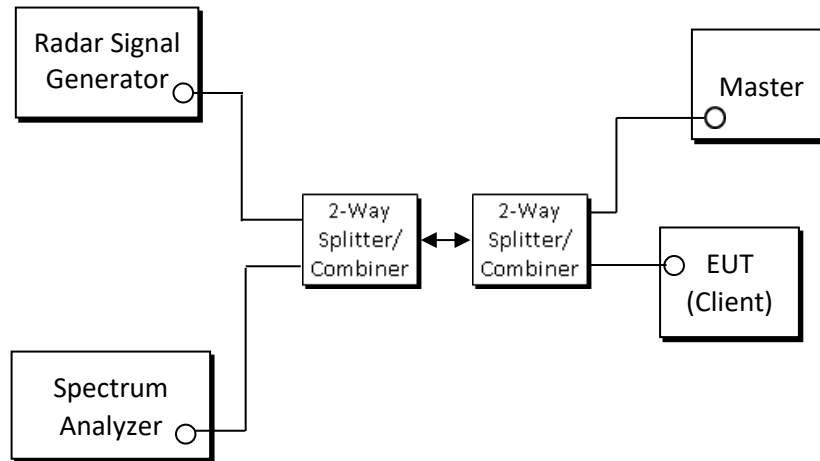
Figure 5-1. Test Setup
