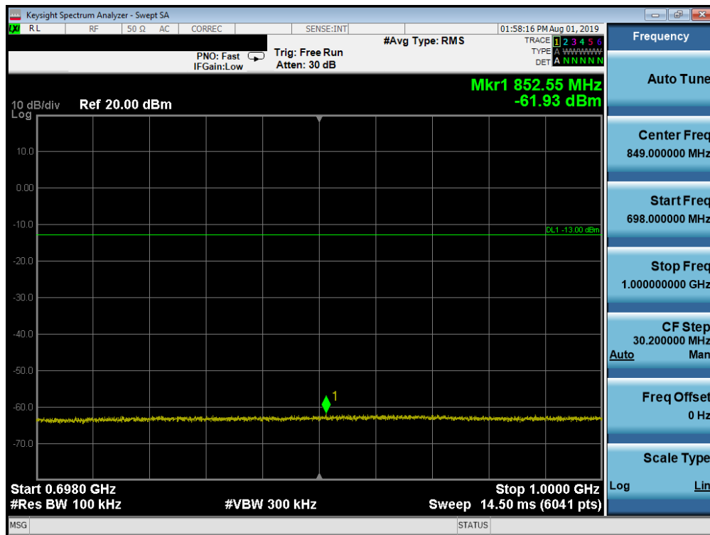
Plot 7-113. Conducted Spurious Plot (Band 71 - 10.0MHz QPSK - RB Size 1, RB Offset 0 - Low Channel)
