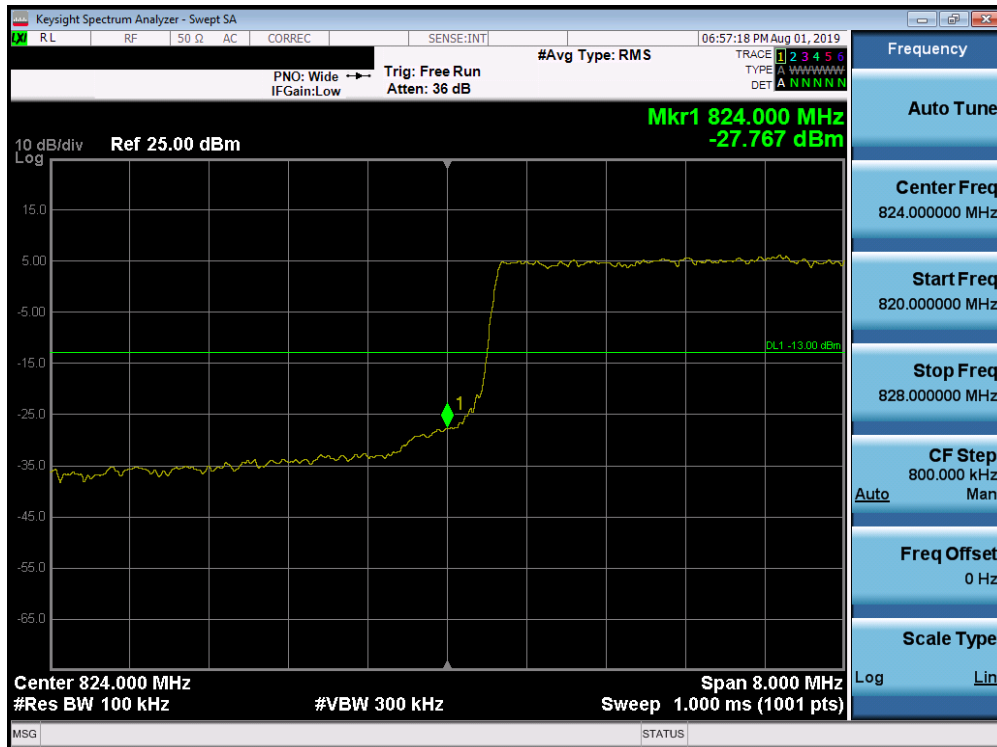
Plot 7-209. Lower Band Edge Plot (Band 26/5 - 10.0MHz QPSK - Full RB Configuration)
