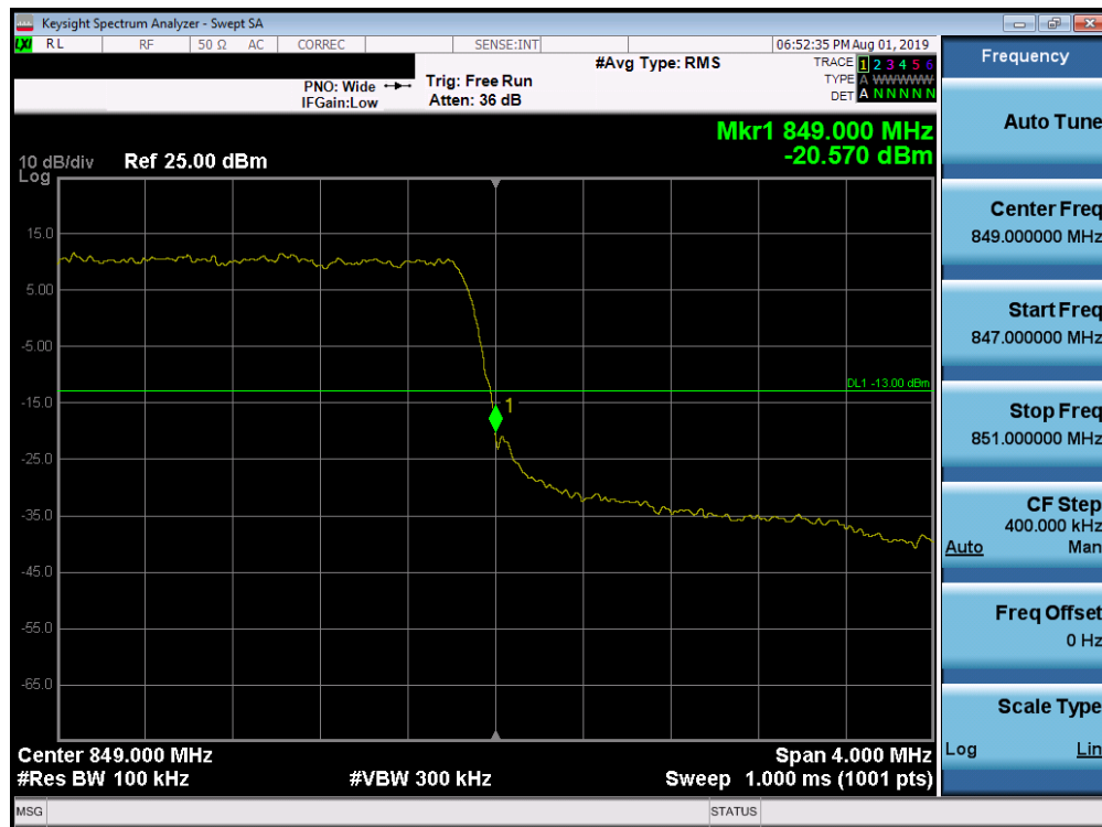
Plot 7-206. Upper Band Edge Plot (Band 26/5 - 3.0MHz QPSK - Full RB Configuration)
