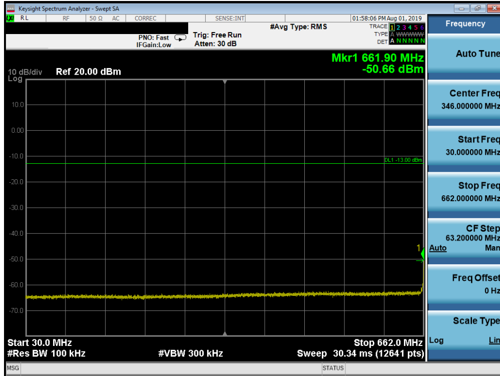
Plot 7-112. Conducted Spurious Plot (Band 71 - 10.0MHz QPSK - RB Size 1, RB Offset 0 - Low Channel)
