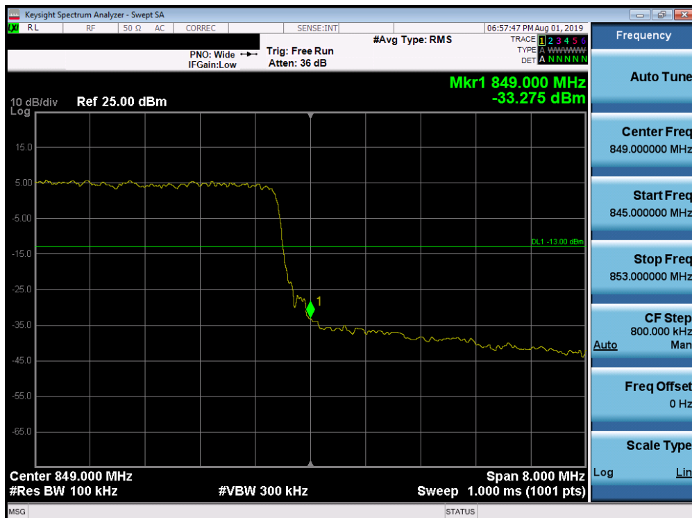
Plot 7-210. Upper Band Edge Plot (Band 26/5 - 10.0MHz QPSK - Full RB Configuration)
