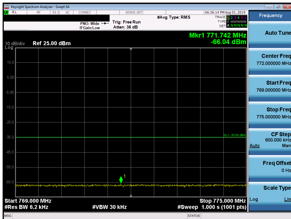
Plot 7-60. Lower Emission Mask Plot (LTE Band 14, 10MHz QPSK – RB Size 50)
