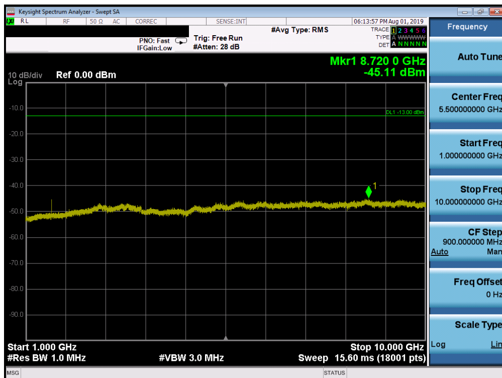
Plot 7-41. Conducted Spurious Plot (LTE Band 14, 5.0 MHz QPSK – RB Size 1, RB Offset 0 – Mid Channel)
