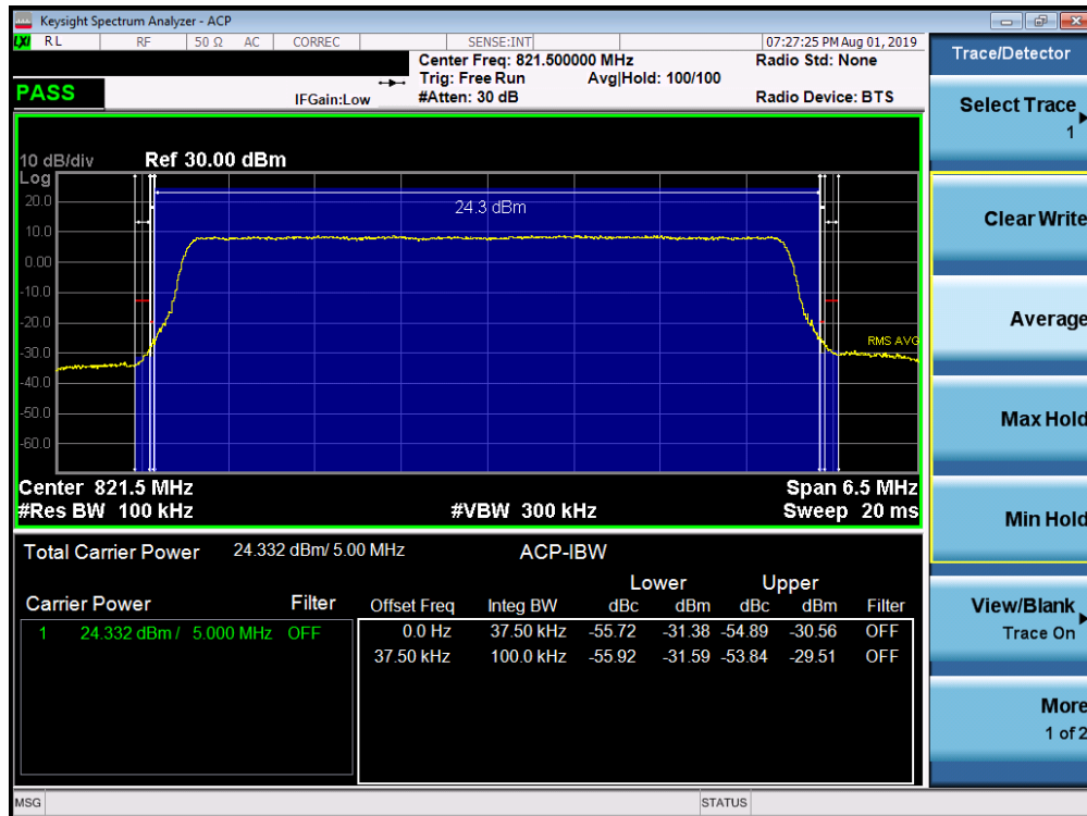
Plot 7-52. Channel Edge Plot (LTE Band 26, 5MHz QPSK – RB Size 25 – High Channel)
