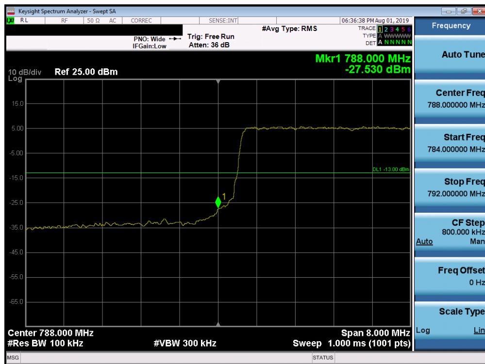
Plot 7-59. Lower Band Edge Plot (LTE Band 14, 10MHz QPSK – RB Size 50)
