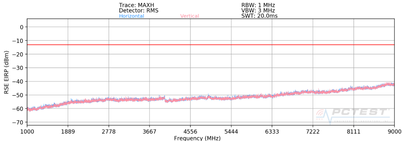
Plot 7-66. Radiated Spurious Plot above 1GHz (LTE Band 26)
