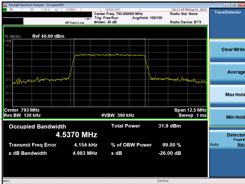
Plot 7-19. Occupied Bandwidth Plot (LTE Band 14, 5MHz 16-QAM – RB Size 25)
