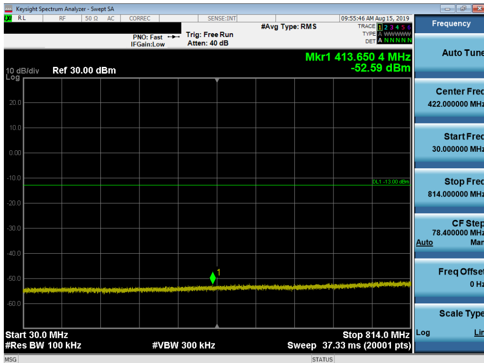
Plot 7-33. Conducted Spurious Plot (LTE Band 26, 5.0 MHz QPSK – RB Size 1, RB Offset 0 – High Channel)
