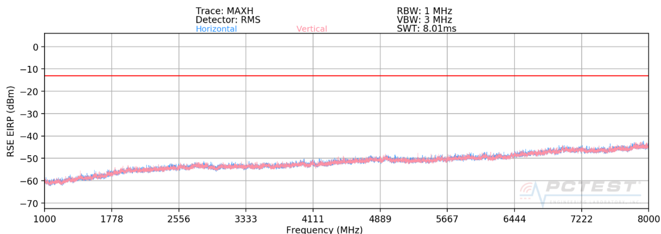
Plot 7-67. Radiated Spurious Plot above 1GHz (LTE Band 14)
