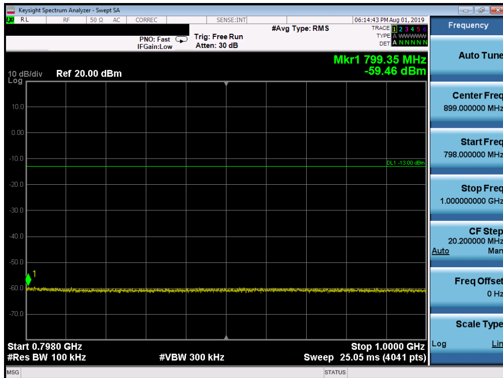
Plot 7-37. Conducted Spurious Plot (LTE Band 14, 5.0 MHz QPSK – RB Size 1, RB Offset 0 – Low Channel)
