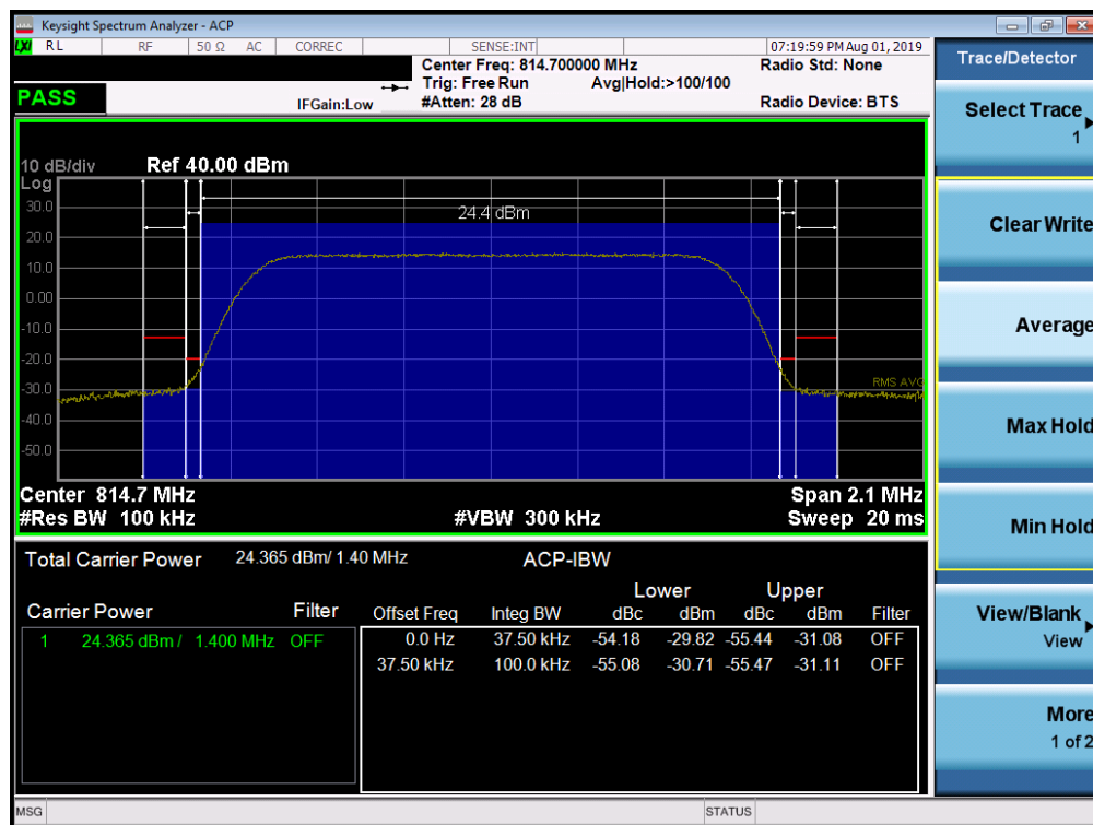
Plot 7-47. Channel Edge Plot (LTE Band 26, 1.4MHz QPSK – RB Size 6– Low Channel)
