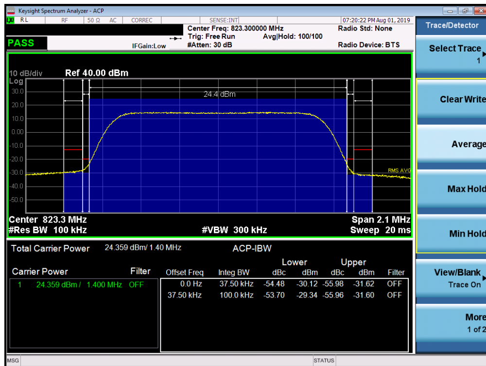
Plot 7-48. Channel Edge Plot (LTE Band 26, 1.4MHz QPSK – RB Size 6 – High Channel)
