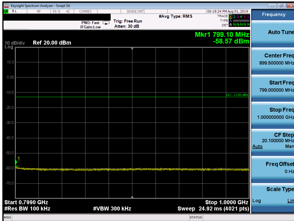
Plot 7-43. Conducted Spurious Plot (LTE Band 14, 5.0 MHz QPSK – RB Size 1, RB Offset 0 – High Channel)
