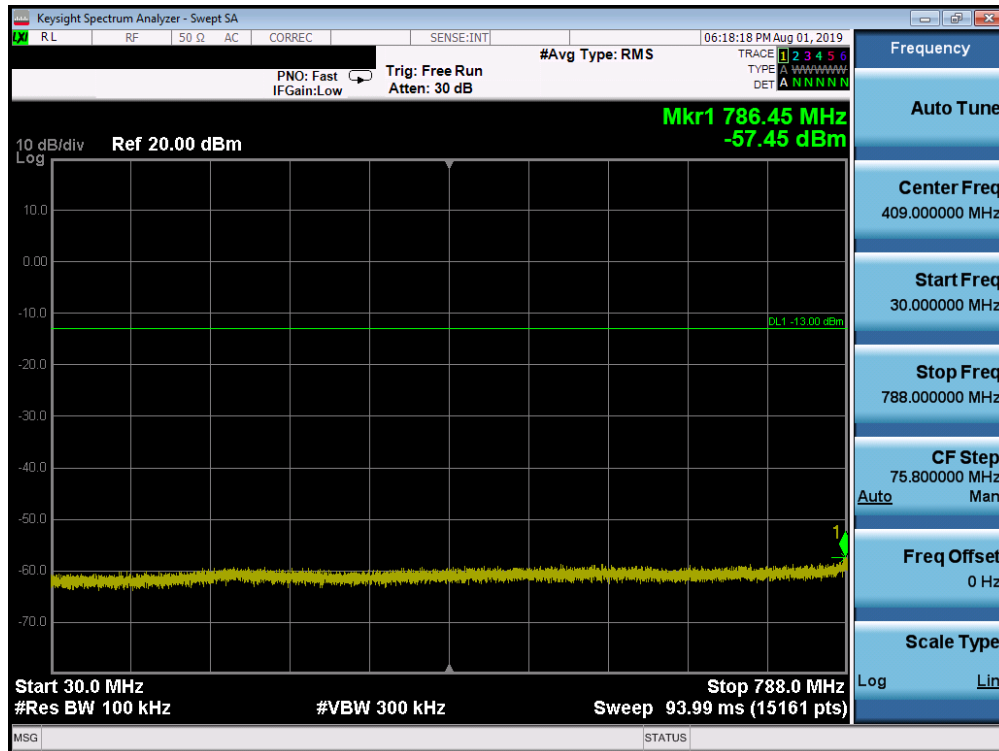
Plot 7-42. Conducted Spurious Plot (LTE Band 14, 5.0 MHz QPSK – RB Size 1, RB Offset 0 – High Channel)
