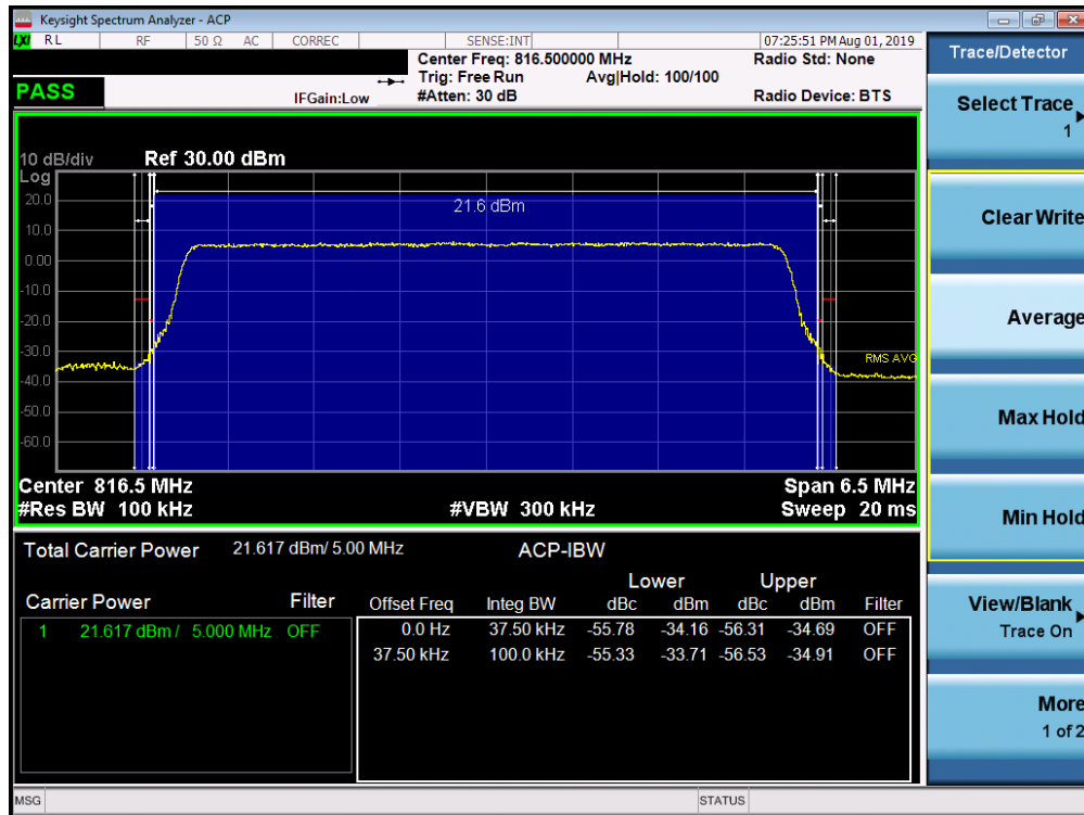
Plot 7-51. Channel Edge Plot (LTE Band 26, 5MHz QPSK – RB Size 25– Low Channel)
