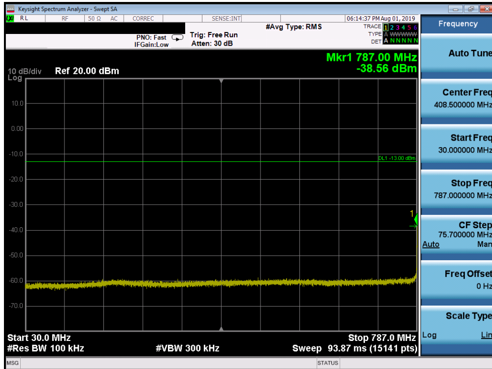
Plot 7-36. Conducted Spurious Plot (LTE Band 14, 5.0 MHz QPSK – RB Size 1, RB Offset 0 – Low Channel)
