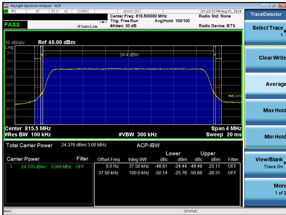
Plot 7-49. Channel Edge Plot (LTE Band 26, 3MHz QPSK – RB Size 15– Low Channel)
