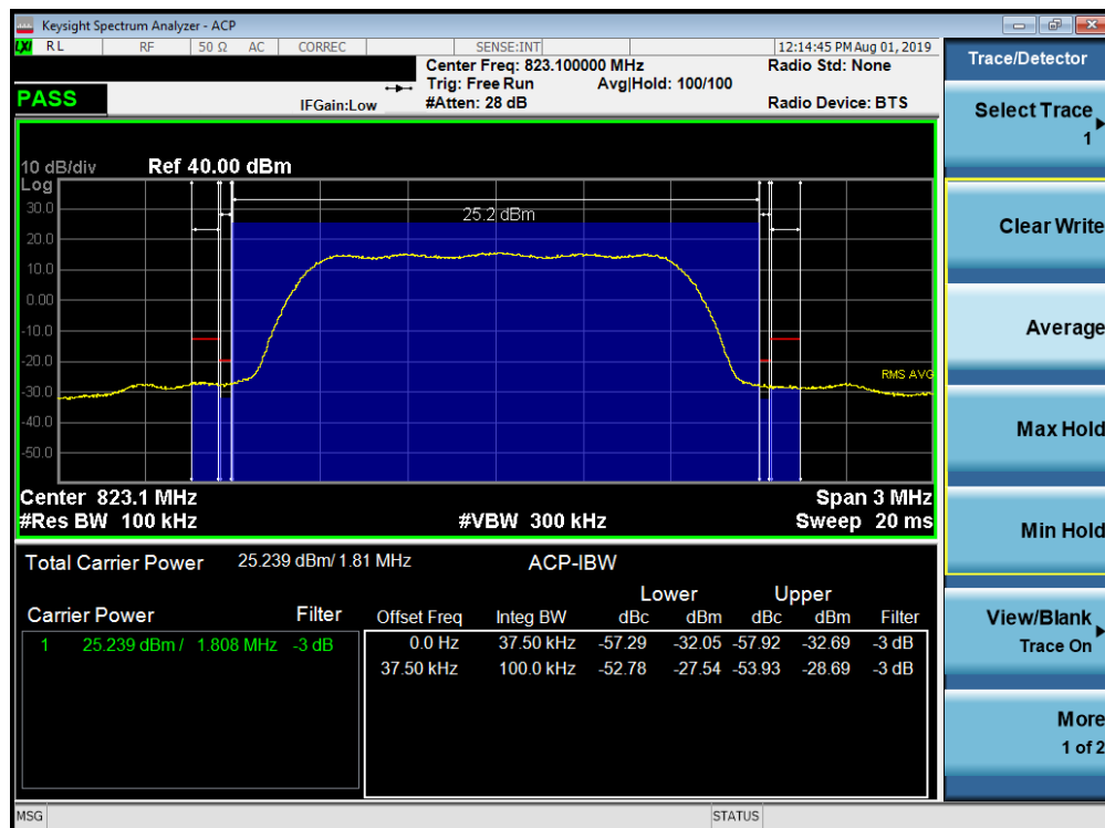
Plot 7-46. Channel Edge Plot (CDMA BC10 - Ch. 684)
