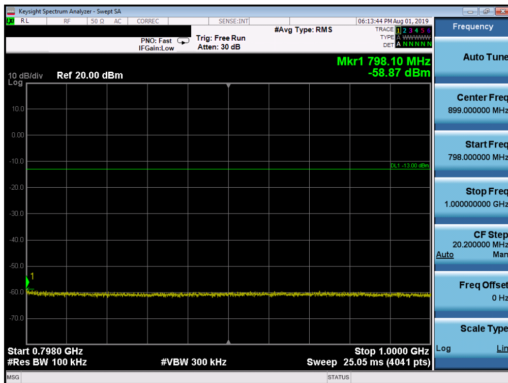
Plot 7-40. Conducted Spurious Plot (LTE Band 14, 5.0 MHz QPSK – RB Size 1, RB Offset 0 – Mid Channel)
