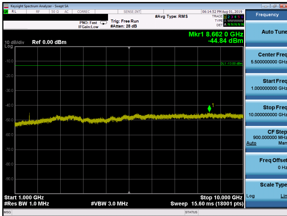
Plot 7-38. Conducted Spurious Plot (LTE Band 14, 5.0 MHz QPSK – RB Size 1, RB Offset 0 – Low Channel)
