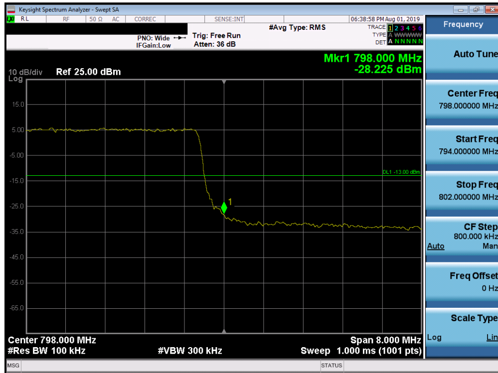
Plot 7-61. Upper Band Edge Plot (LTE Band 14, 10MHz QPSK – RB Size 50)
