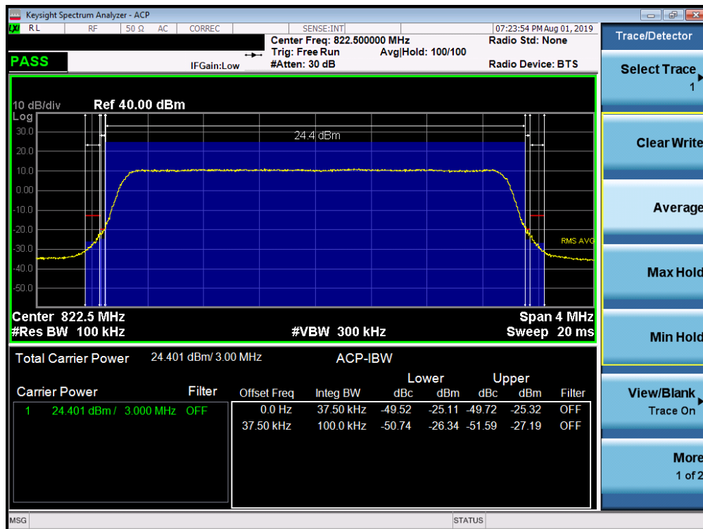
Plot 7-50. Channel Edge Plot (LTE Band 26, 3MHz QPSK – RB Size 15 – High Channel)
