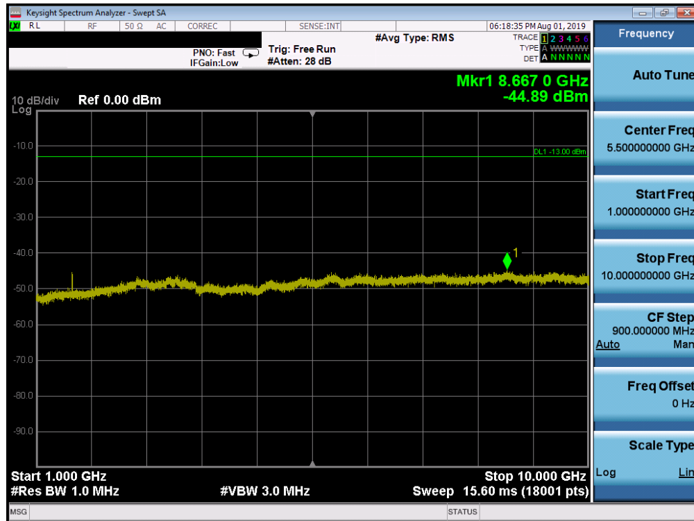
Plot 7-44. Conducted Spurious Plot (LTE Band 14, 5.0 MHz QPSK – RB Size 1, RB Offset 0 – High Channel)
