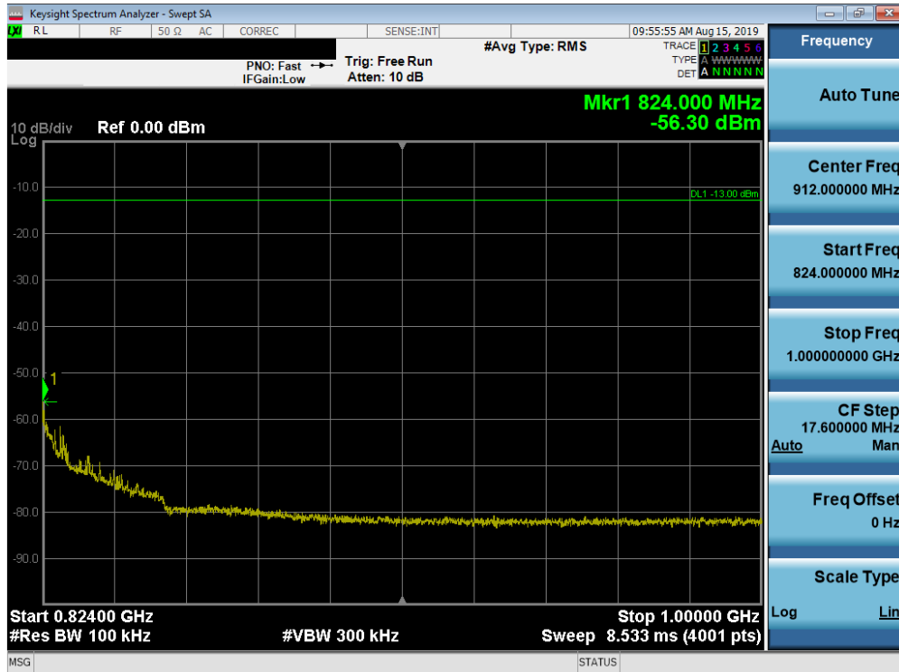
Plot 7-34. Conducted Spurious Plot (LTE Band 26, 5.0 MHz QPSK – RB Size 1, RB Offset 0 – High Channel)
