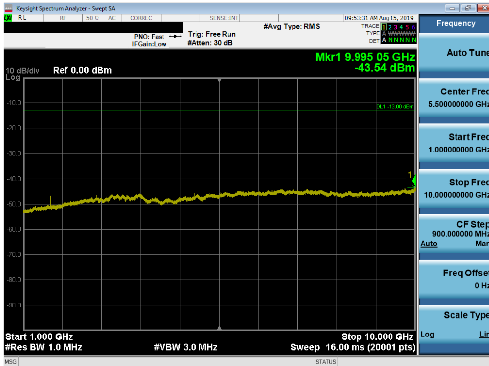
Plot 7-32. Conducted Spurious Plot (LTE Band 26, 5.0 MHz QPSK – RB Size 1, RB Offset 0 – Low Channel)
