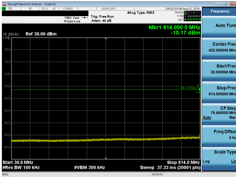
Plot 7-30. Conducted Spurious Plot (LTE Band 26, 5.0 MHz QPSK – RB Size 1, RB Offset 0 – Low Channel)
