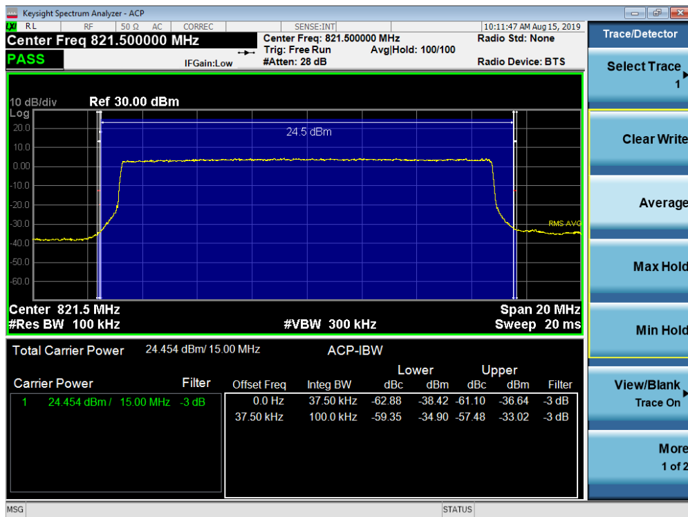
Plot 7-54. Channel Edge Plot (LTE Band 26, 15MHz QPSK – RB Size 75)
