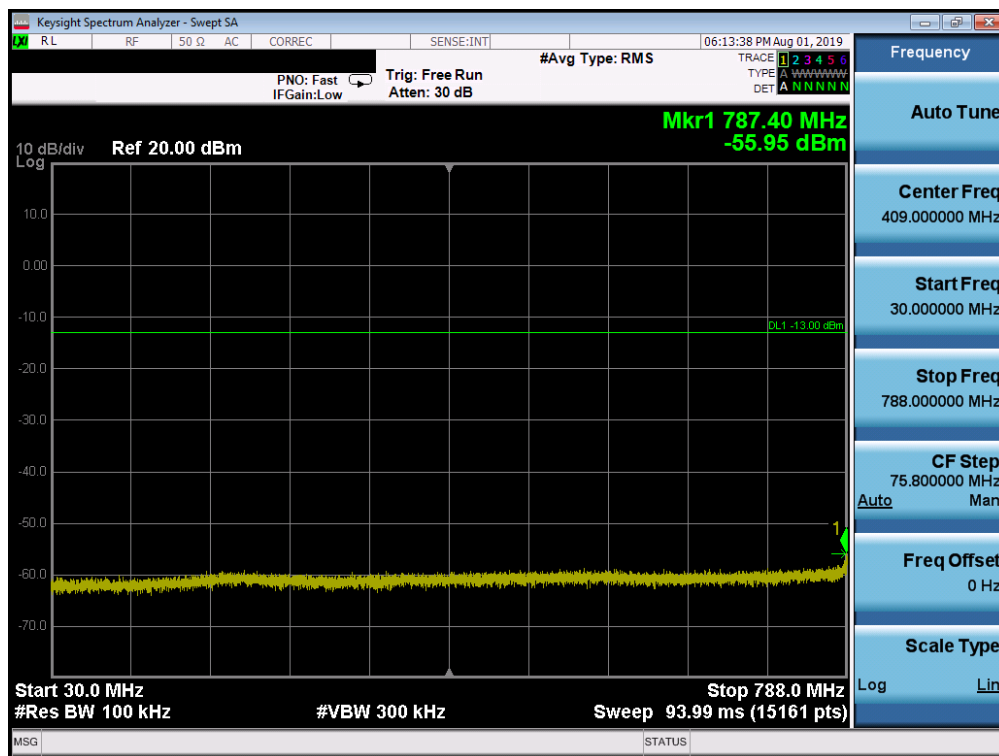
Plot 7-39. Conducted Spurious Plot (LTE Band 14, 5.0 MHz QPSK – RB Size 1, RB Offset 0 – Mid Channel)
