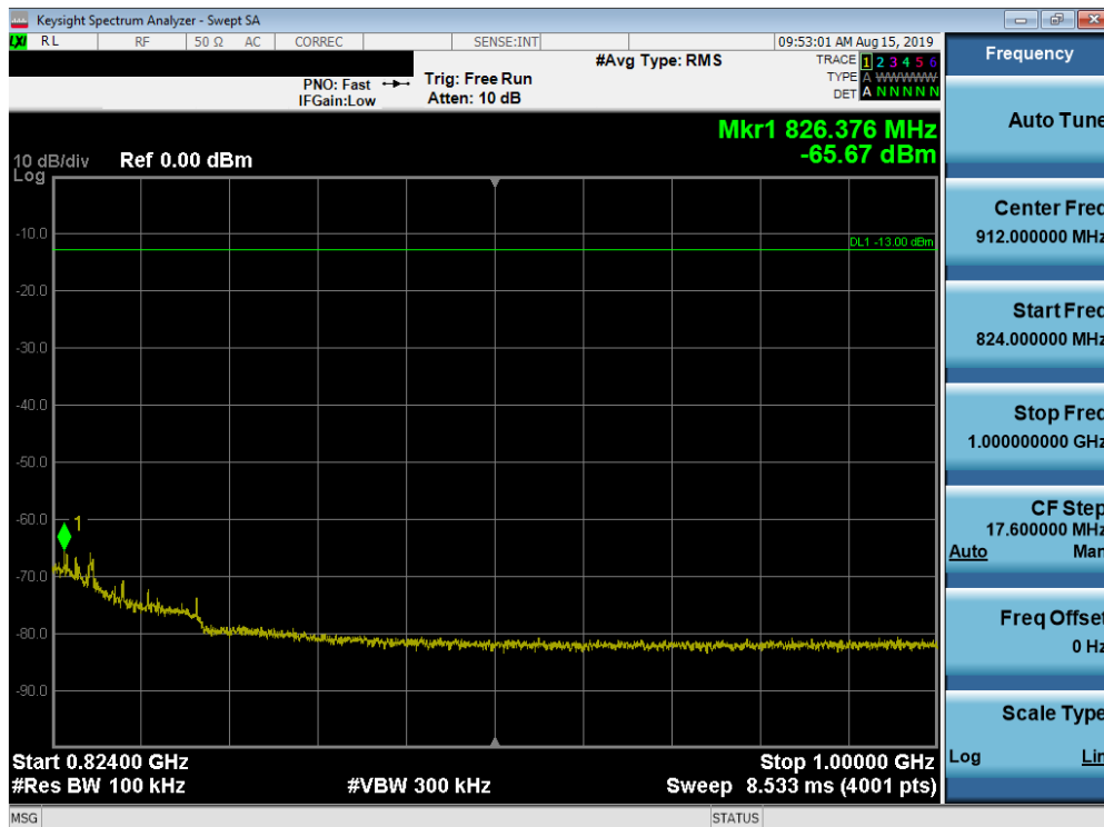
Plot 7-31. Conducted Spurious Plot (LTE Band 26, 5.0 MHz QPSK – RB Size 1, RB Offset 0 – Low Channel)
