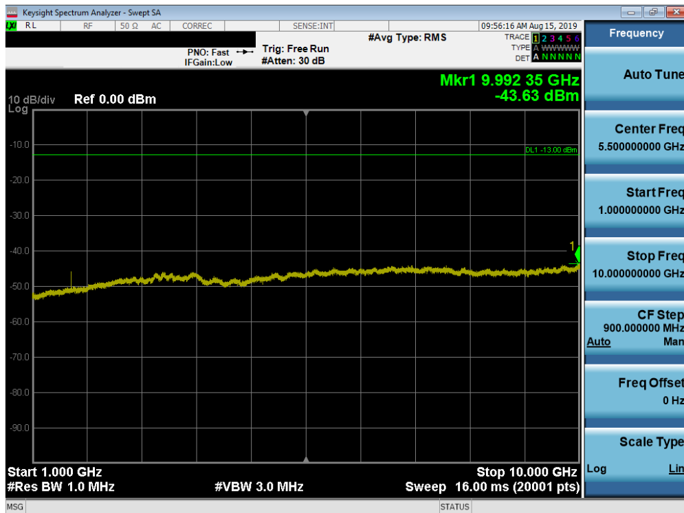
Plot 7-35. Conducted Spurious Plot (LTE Band 26, 5.0 MHz QPSK – RB Size 1, RB Offset 0 – High Channel)
