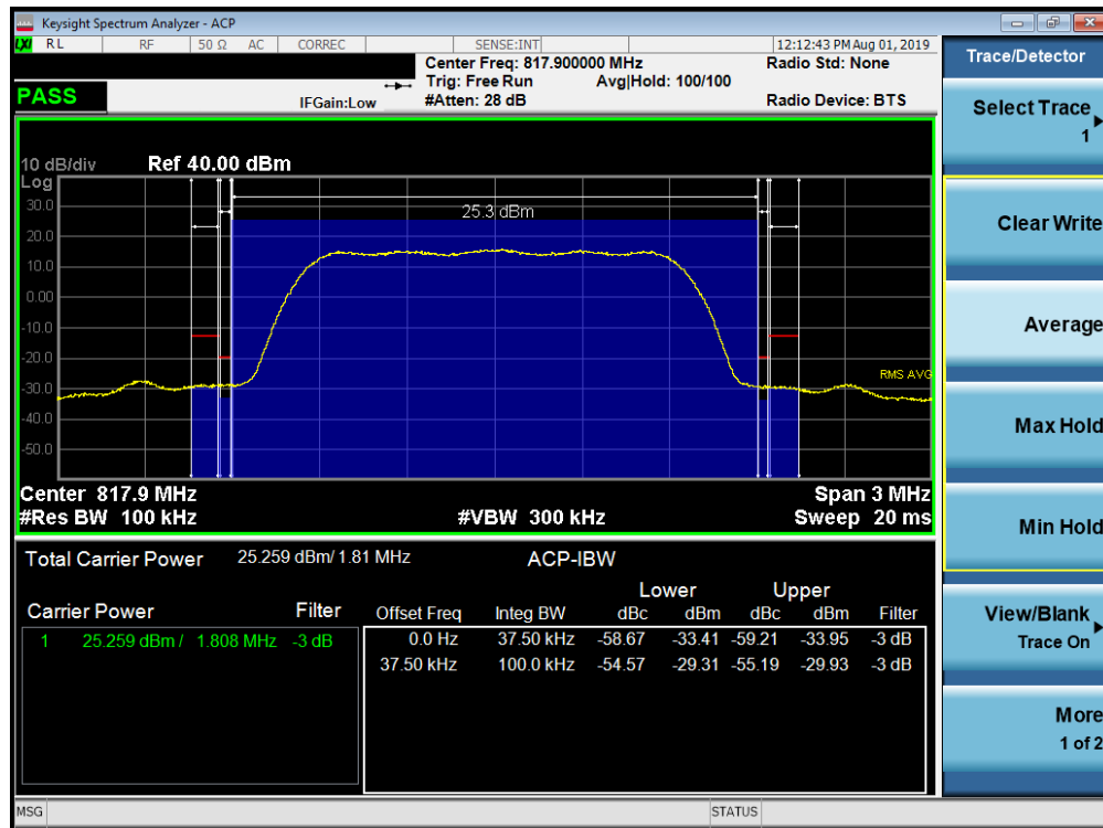
Plot 7-45. Channel Edge Plot (CDMA BC10 - Ch. 476)
