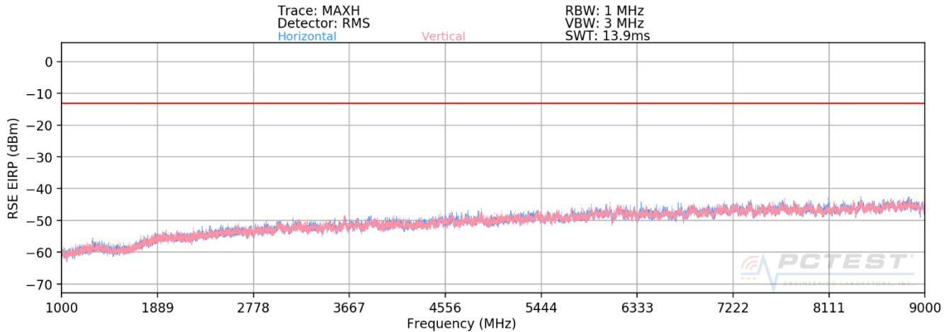
Plot 7-65. Radiated Spurious Plot above 1GHz (CDMA BC10)
