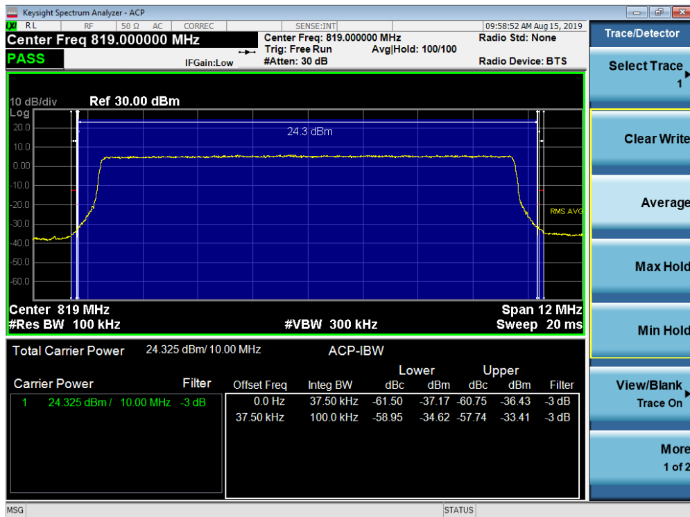
Plot 7-53. Channel Edge Plot (LTE Band 26, 10MHz QPSK – RB Size 50)
