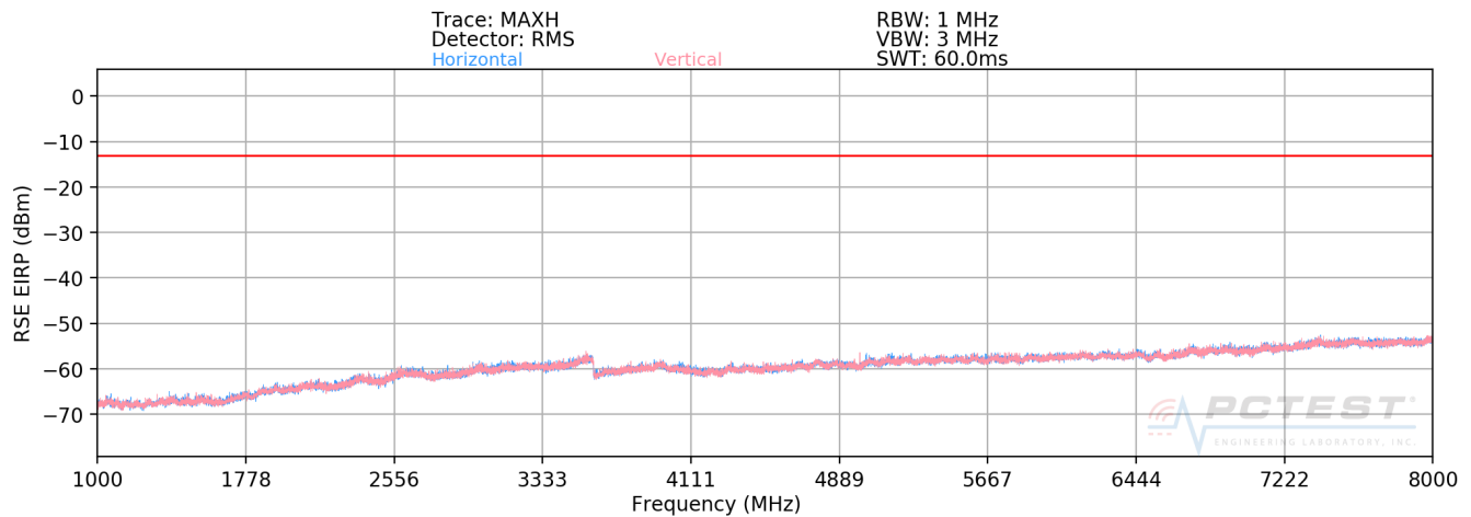
Plot 7-5. Radiated Spurious Plot above 1 GHz (LTE Band 14)
