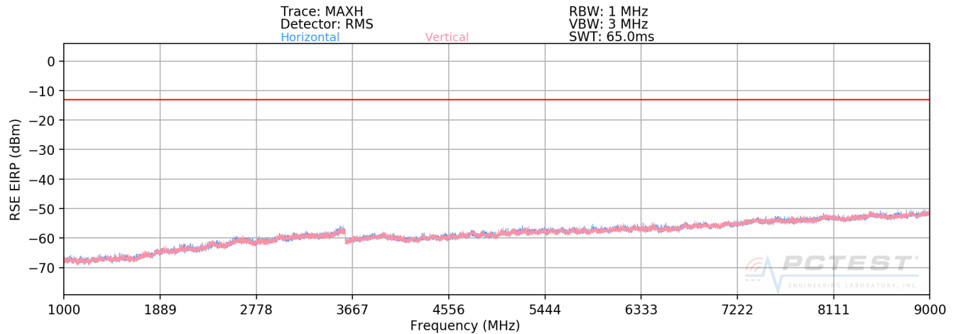
Plot 7-3. Radiated Spurious Plot above 1GHz (CDMA BC10)
