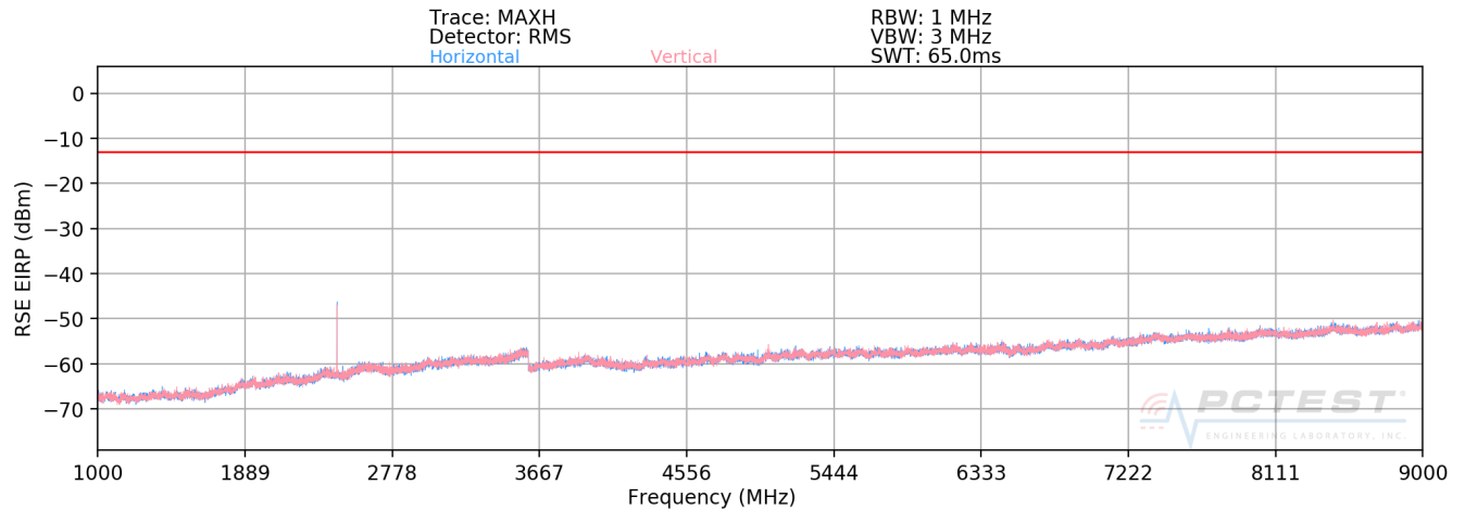
Plot 7-4. Radiated Spurious Plot above 1GHz (LTE Band 26)
