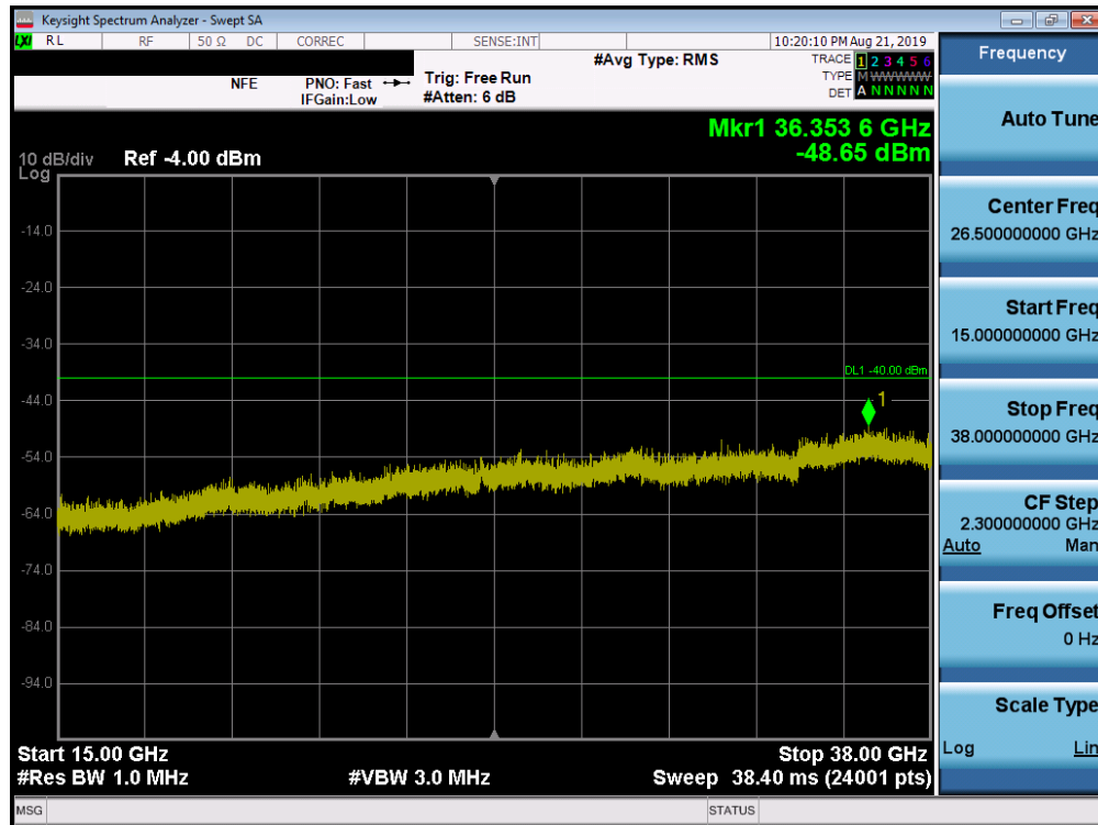
Plot 7-27. Conducted Spurious Plot (Band 48 - 20.0MHz QPSK - RB Size 1, RB Offset 99 - High Channel)
