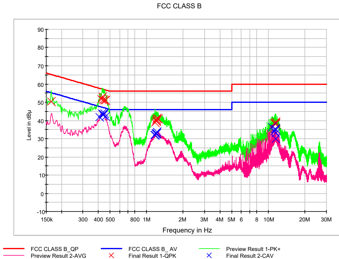
Figure 5: Conducted Emission, DISPLAY mode, Line (L1)
