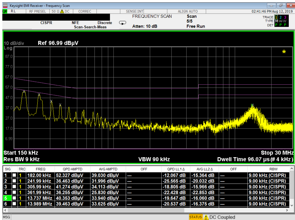
Plot 7-9. Line-Conducted Test Plot with WCP (N) with Antenna Terminated in 50Ω
