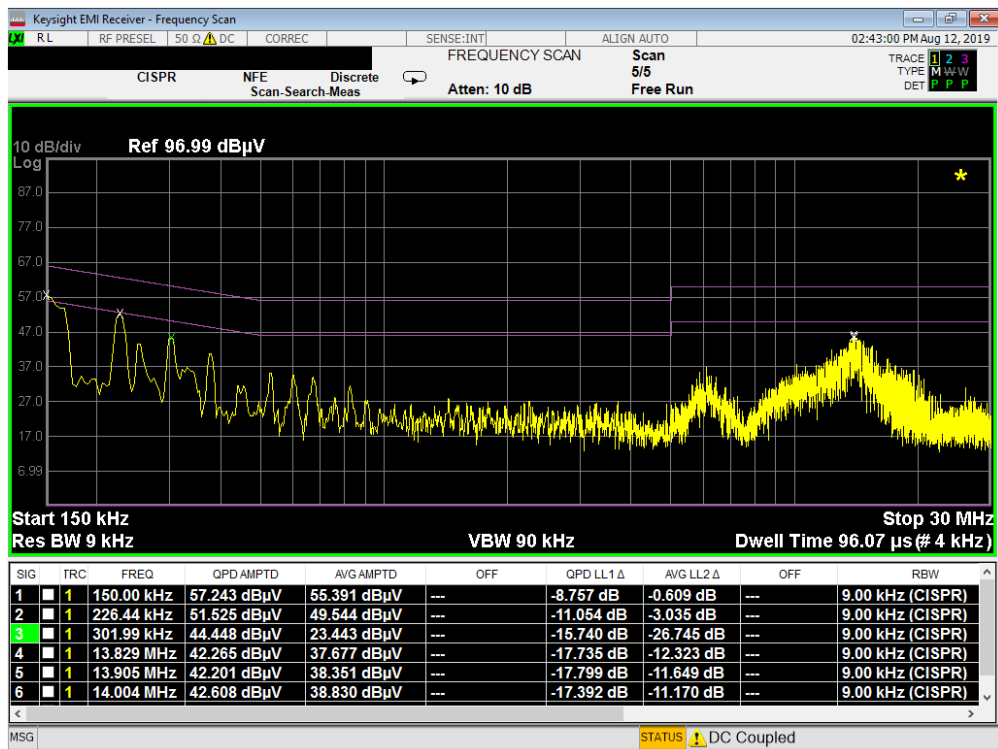
Plot 7-8. Line-Conducted Test Plot (L1) with Antenna Terminated in 50Ω
