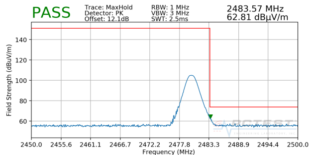
Plot 7-6. Radiated Restricted Upper Band Edge Measurement (Peak)
