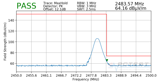
Plot 7-10. Radiated Restricted Upper Band Edge Measurement with Dual Display (Peak)
