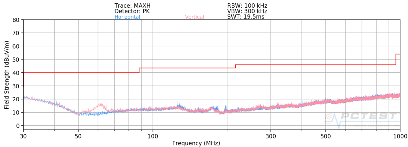
Plot 7-13. Radiated Spurious Plot below 1GHz
