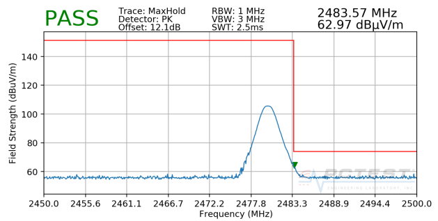
Plot 7-12. Radiated Restricted Upper Band Edge Measurement with Dual Display and WCP (Peak)
