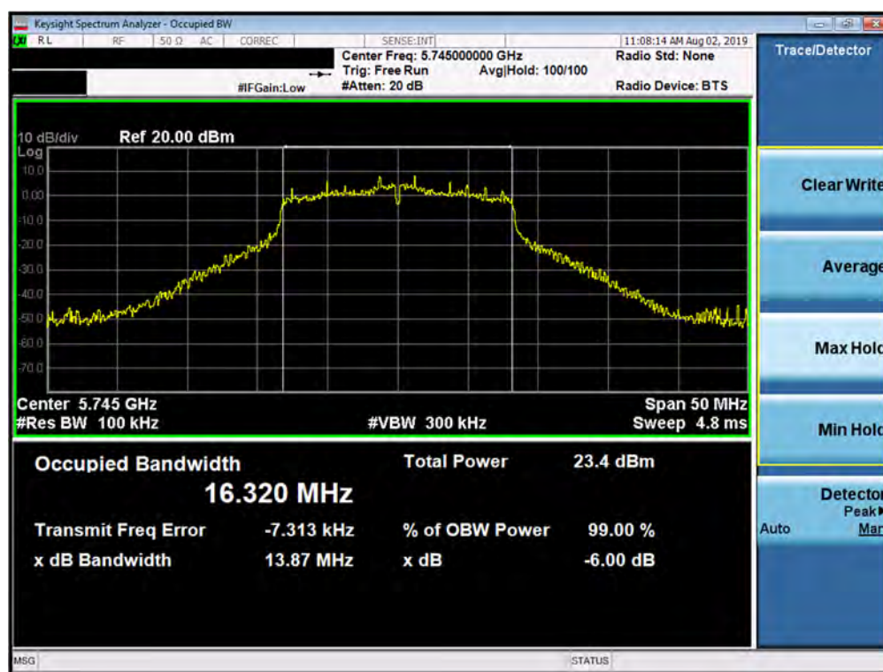
Plot 7-61. 6dB Bandwidth Plot SISO ANT1 (802.11a (UNII Band 3) – Ch. 149)
