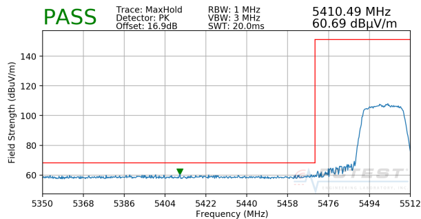
Plot 7-27. Radiated Lower Band Edge Plot SISO ANT1 (Peak – UNII Band 2C)
