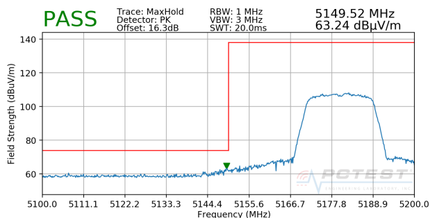
Plot 7-23. Radiated Lower Band Edge Plot SISO ANT1 (Peak – UNII Band 1)
