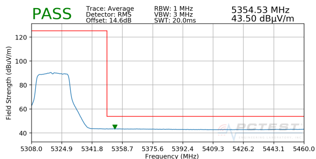
Plot 7-33. Radiated Band Edge Plot SISO ANT1 (Average – Dual Display and WCP)
