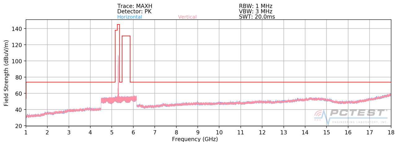
Plot 7-2. Radiated Spurious Plot above 1GHz SISO ANT1 (802.11a – U2A Ch. 56)
