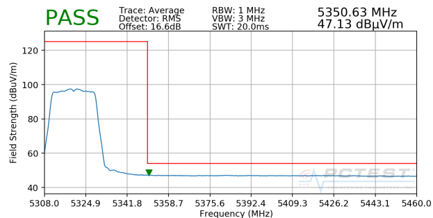
Plot 7-24. Radiated Upper Band Edge Plot SISO ANT1 (Average – UNII Band 2A)
