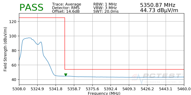
Plot 7-29. Radiated Band Edge Plot SISO ANT1 (Average – WCP)
