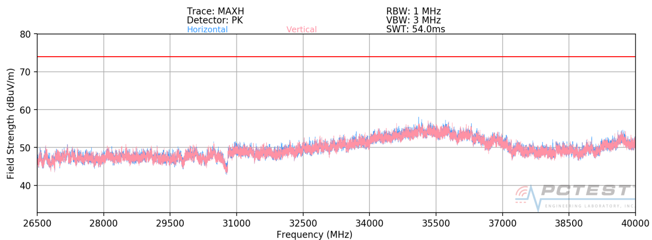
Plot 7-18. Radiated Spurious Plot 26.5GHz - 40GHz MIMO/CDD (802.11a)
