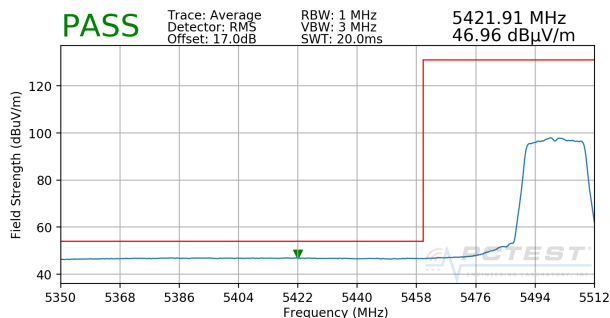
Plot 7-26. Radiated Lower Band Edge Plot SISO ANT1 (Average – UNII Band 2C)
