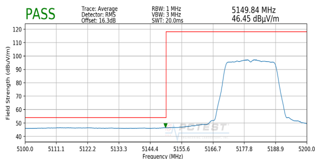
Plot 7-22. Radiated Lower Band Edge Plot SISO ANT1 (Average – UNII Band 1)
