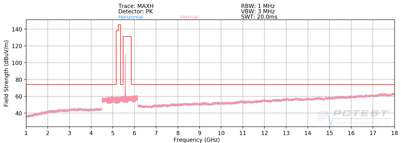
Plot 7-15. Radiated Spurious Plot above 1GHz MIMO/CDD (802.11a – U2C Ch. 116120)
