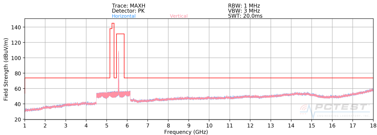
Plot 7-3. Radiated Spurious Plot above 1GHz SISO ANT1 (802.11a – U2C Ch. 120)
