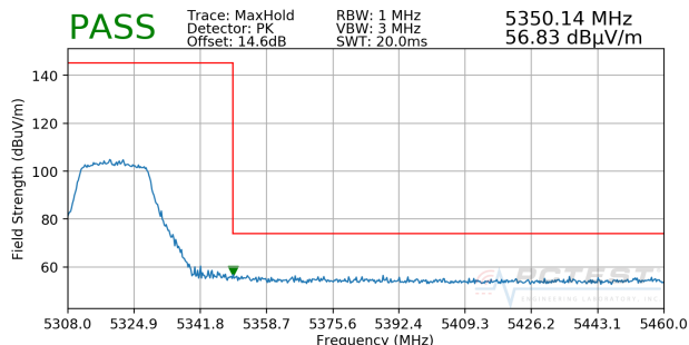
Plot 7-32. Radiated Band Edge Plot SISO ANT1 (Peak – Dual Display)
