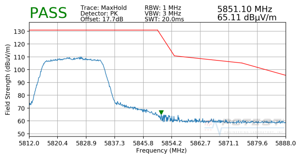
Plot 7-28. Radiated Upper Band Edge Plot SISO ANT1 (Peak – UNII Band 3)
