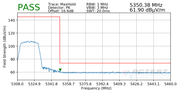
Plot 7-25. Radiated Upper Band Edge Plot SISO ANT1 (Peak – UNII Band 2A)
