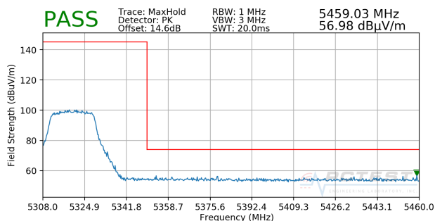
Plot 7-34. Radiated Band Edge Plot SISO ANT1 (Peak – Dual Display and WCP)
