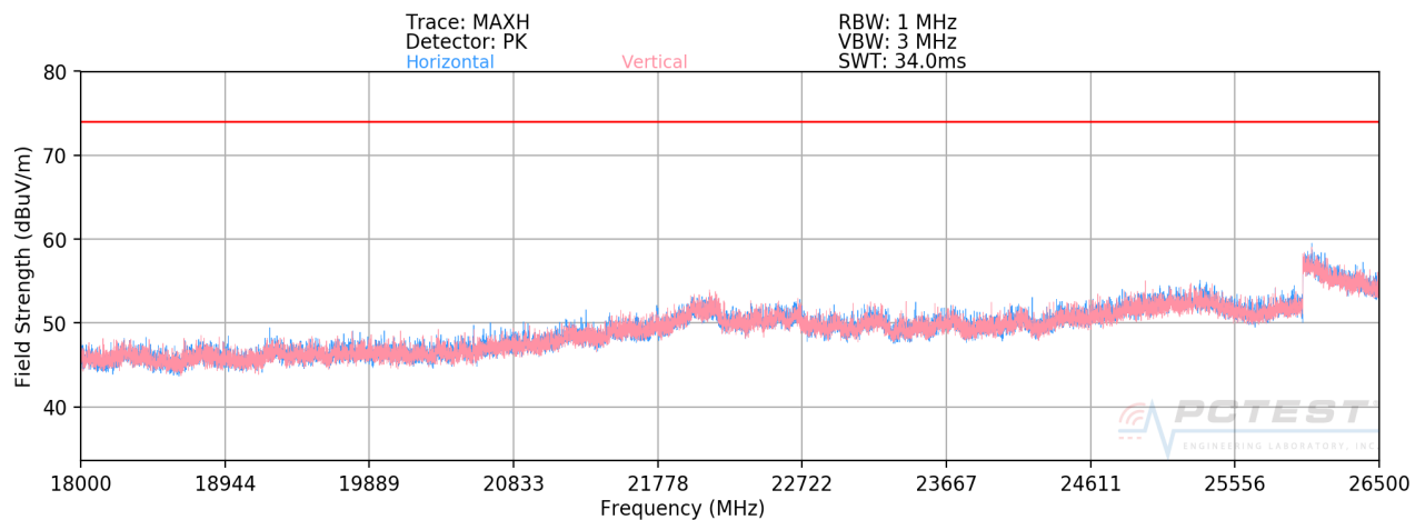
Plot 7-17. Radiated Spurious Plot above 18GHz - 26.5GHz MIMO/CDD (802.11a)
