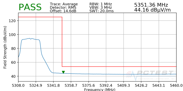
Plot 7-31. Radiated Band Edge Plot SISO ANT1 (Average – Dual Display)
