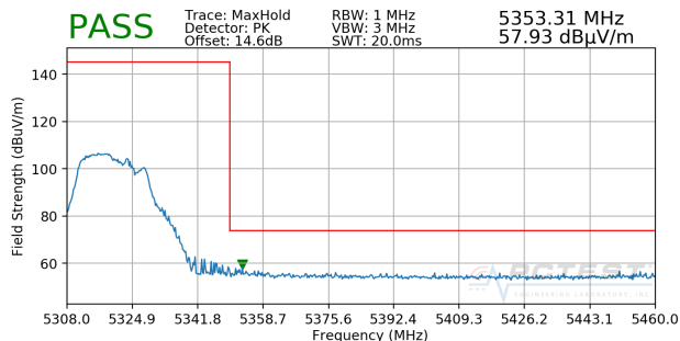
Plot 7-30. Radiated Band Edge Plot SISO ANT1 (Peak – WCP)
