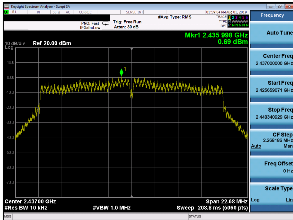
Plot 7-41. Power Spectral Density Plot SISO ANT2 (802.11n (2.4GHz) – Ch. 6)
