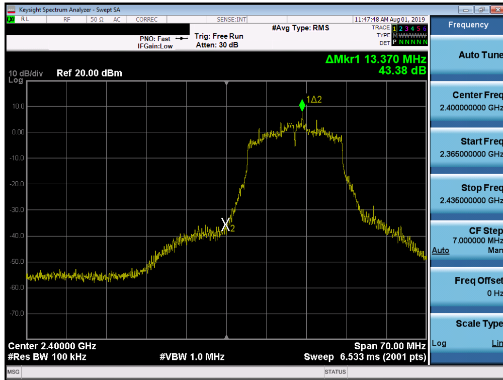
Plot 7-45. Band Edge Plot SISO ANT1 (802.11g- Ch. 1)
