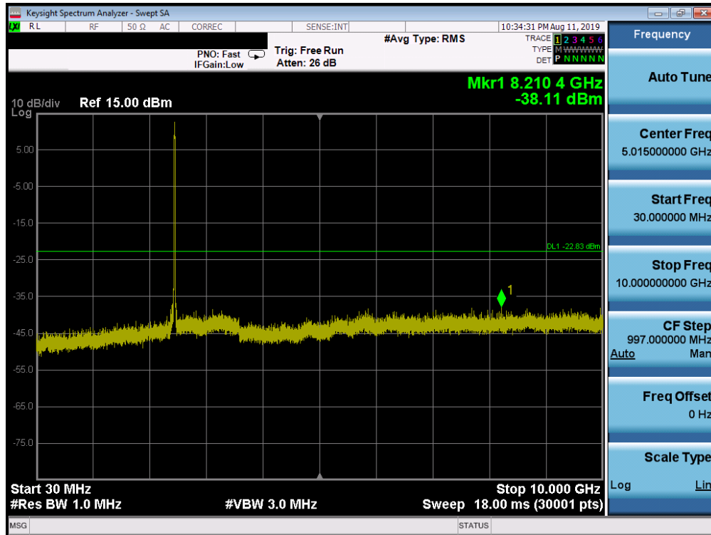
Plot 7-93. Conducted Spurious Plot SISO ANT2 (802.11ac – Ch. 11)
