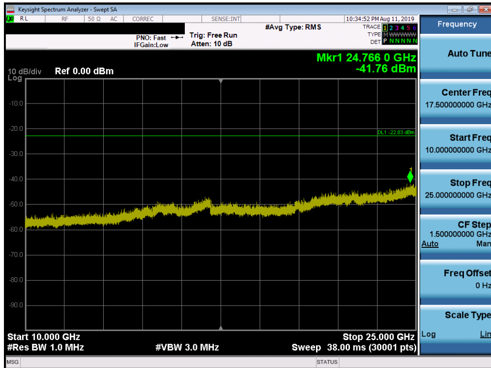
Plot 7-94. Conducted Spurious Plot SISO ANT2 (802.11ac – Ch. 11)
