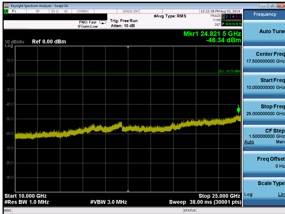
Plot 7-86. Conducted Spurious Plot SISO ANT2 (802.11b – Ch. 6)
