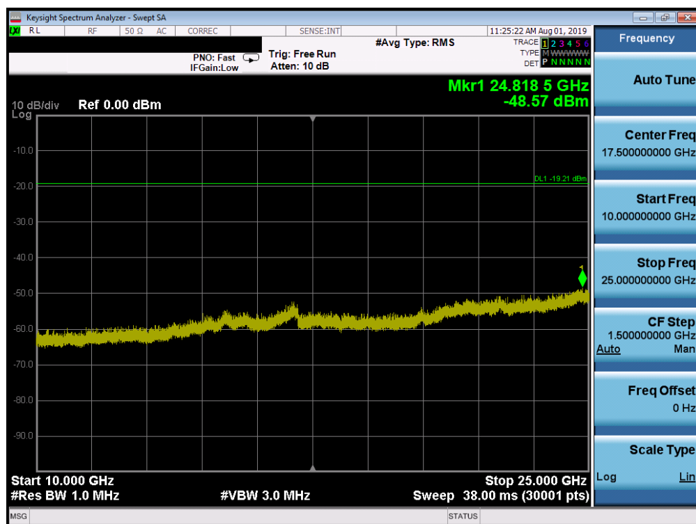
Plot 7-74. Conducted Spurious Plot SISO ANT1 (802.11b – Ch. 6)
