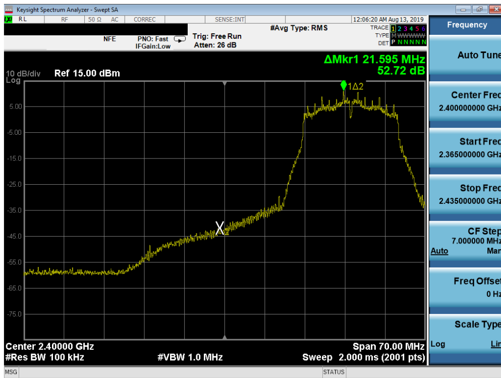
Plot 7-61. Band Edge Plot SISO ANT2 (802.11g- Ch. 3)
