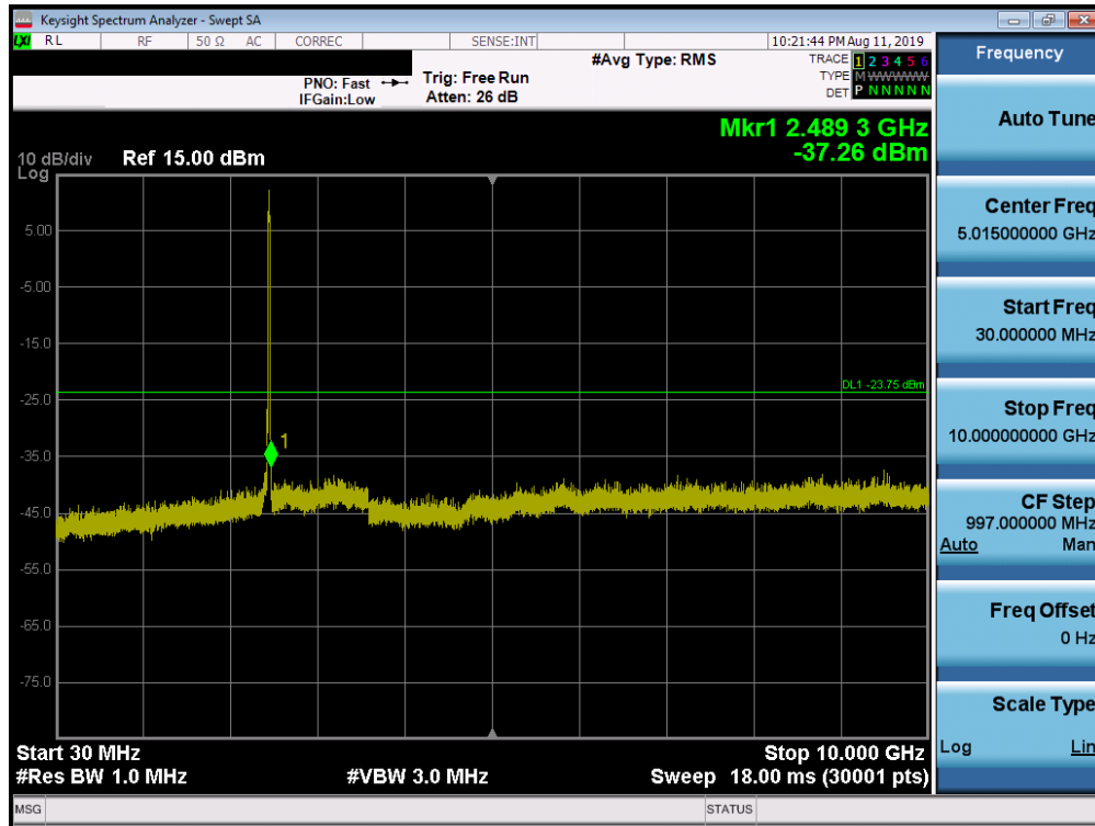
Plot 7-81. Conducted Spurious Plot SISO ANT1 (802.11ac – Ch. 11)
