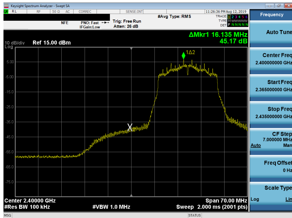
Plot 7-52. Band Edge Plot SISO ANT1 (802.11n (2.4GHz) – Ch. 2)
