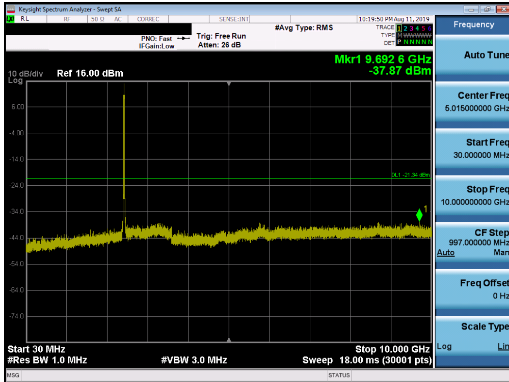
Plot 7-79. Conducted Spurious Plot SISO ANT1 (802.11ac – Ch. 6)
