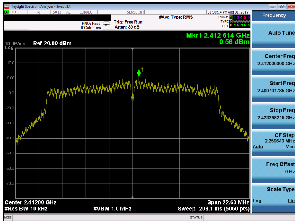
Plot 7-37. Power Spectral Density Plot SISO ANT2 (802.11g – Ch. 1)
