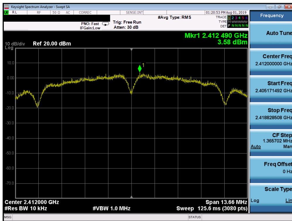
Plot 7-34. Power Spectral Density Plot SISO ANT2 (802.11b – Ch. 1)
