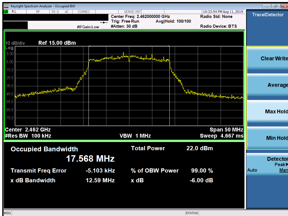
Plot 7-24. 6dB Bandwidth Plot SISO ANT2 (802.11ac (2.4GHz) – Ch. 11)
