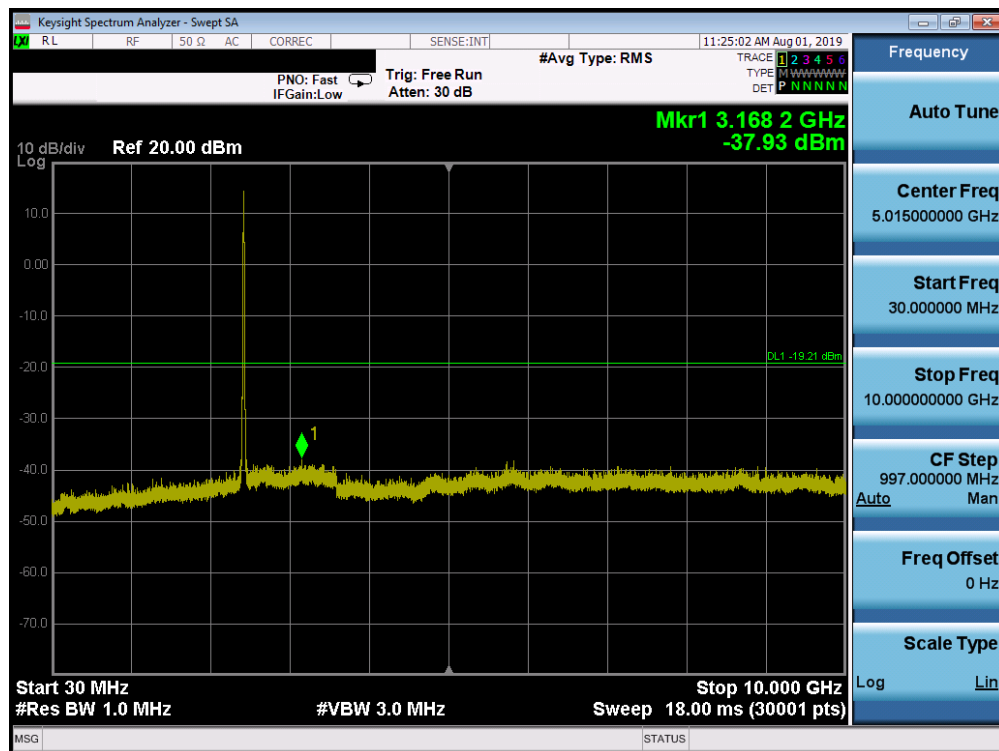
Plot 7-73. Conducted Spurious Plot SISO ANT1 (802.11b – Ch. 6)
