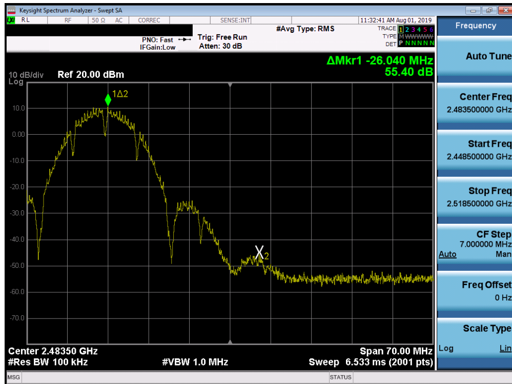
Plot 7-44. Band Edge Plot SISO ANT1 (802.11b – Ch. 11)
