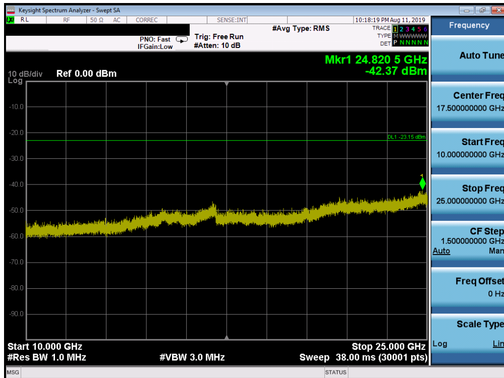
Plot 7-78. Conducted Spurious Plot SISO ANT1 (802.11ac – Ch. 1)
