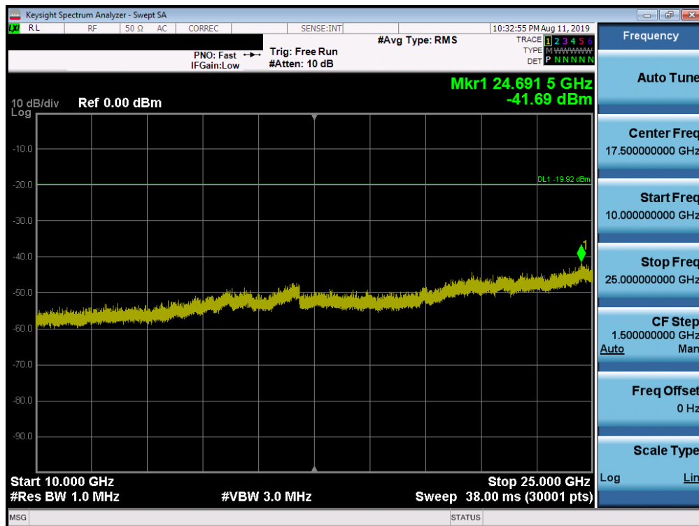
Plot 7-92. Conducted Spurious Plot SISO ANT2 (802.11ac – Ch. 6)
