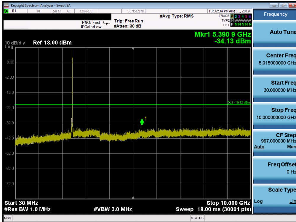
Plot 7-91. Conducted Spurious Plot SISO ANT2 (802.11ac – Ch. 6)
