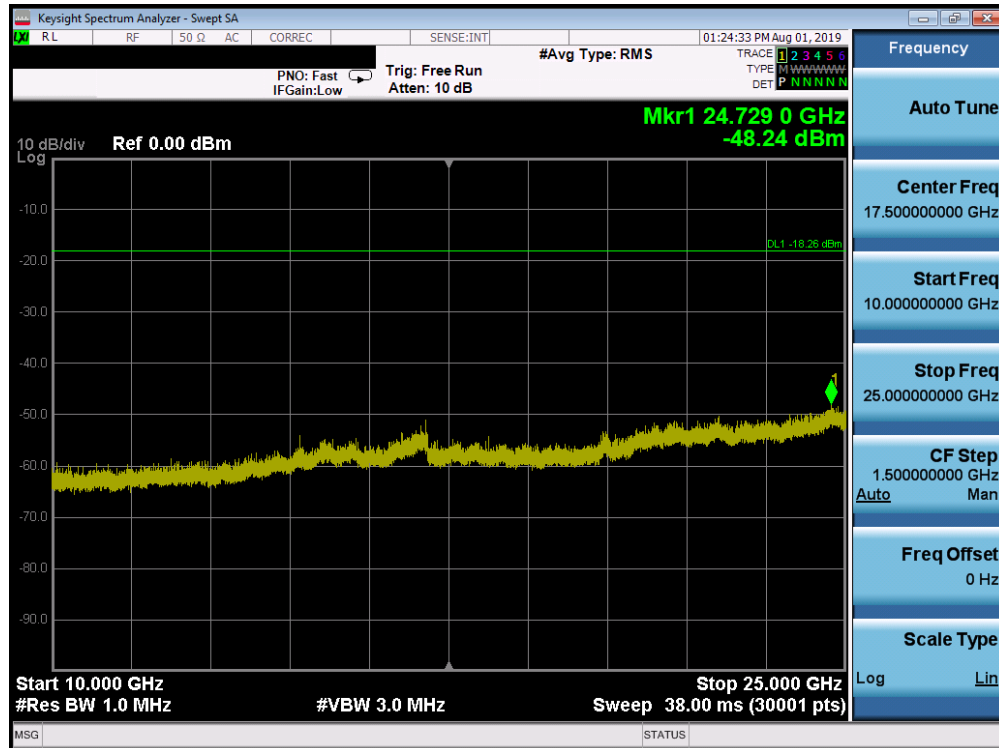
Plot 7-84. Conducted Spurious Plot SISO ANT2 (802.11b – Ch. 1)
