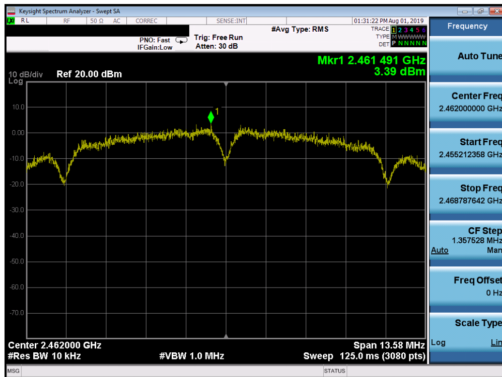
Plot 7-36. Power Spectral Density Plot SISO ANT2 (802.11b – Ch. 11)
