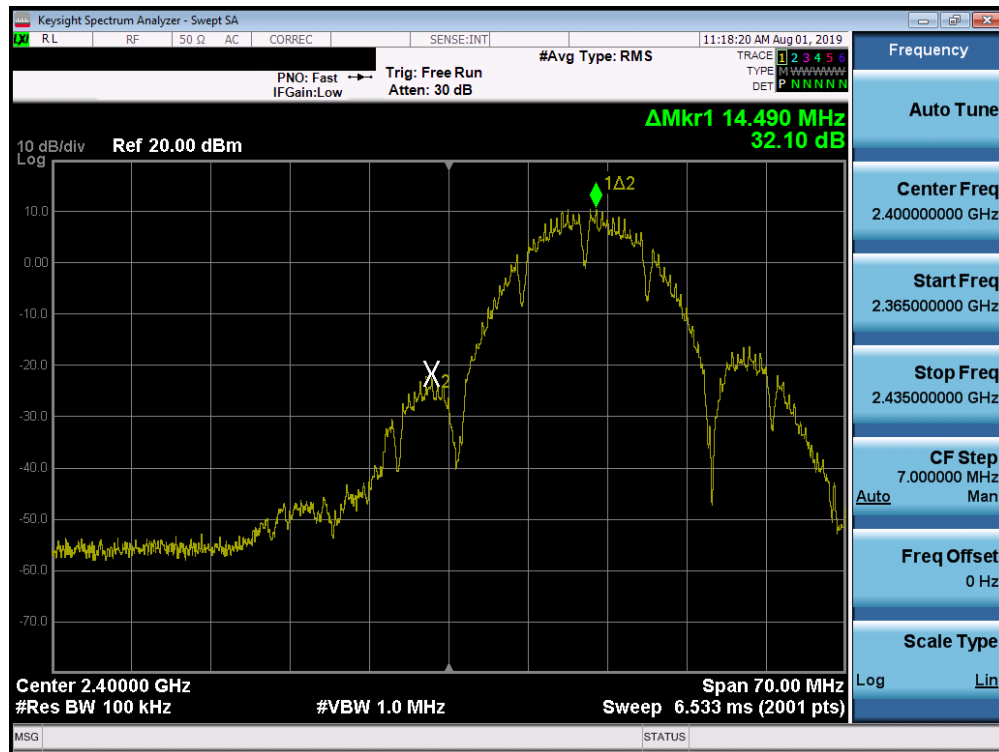
Plot 7-43. Band Edge Plot SISO ANT1 (802.11b – Ch. 1)
