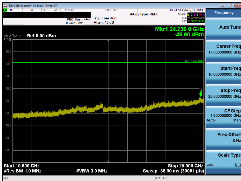
Plot 7-88. Conducted Spurious Plot SISO ANT2 (802.11b – Ch. 11)
