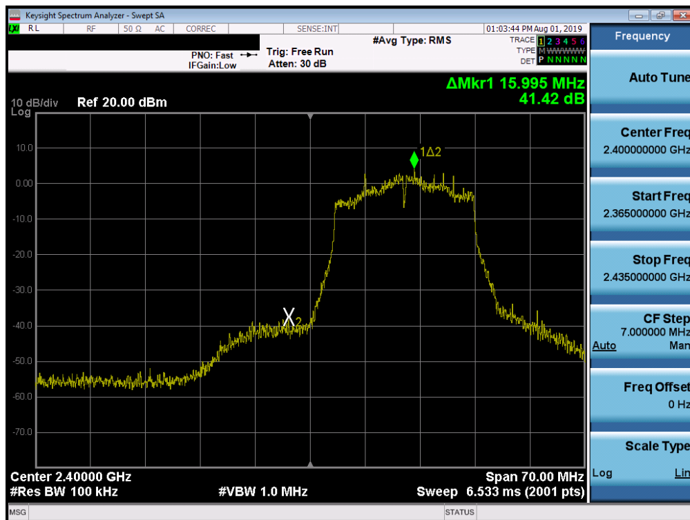
Plot 7-51. Band Edge Plot SISO ANT1 (802.11n (2.4GHz) – Ch. 1)
