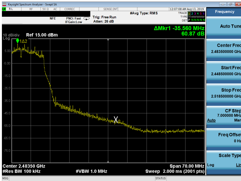
Plot 7-62. Band Edge Plot SISO ANT2 (802.11g- Ch. 9)
