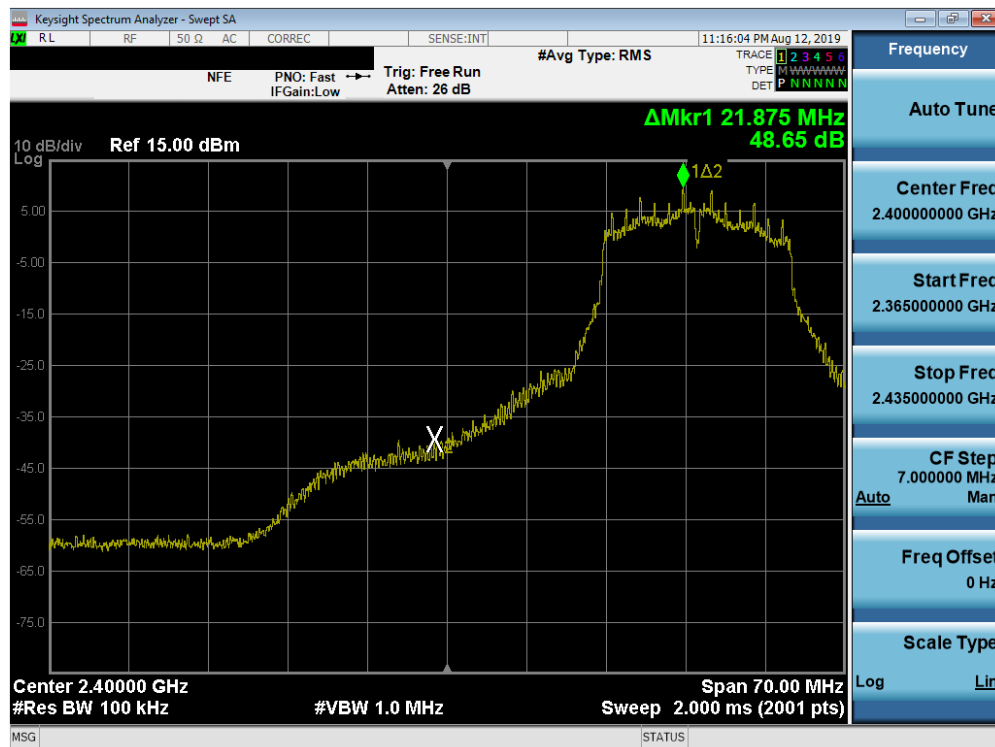
Plot 7-47. Band Edge Plot SISO ANT1 (802.11g- Ch. 3)
