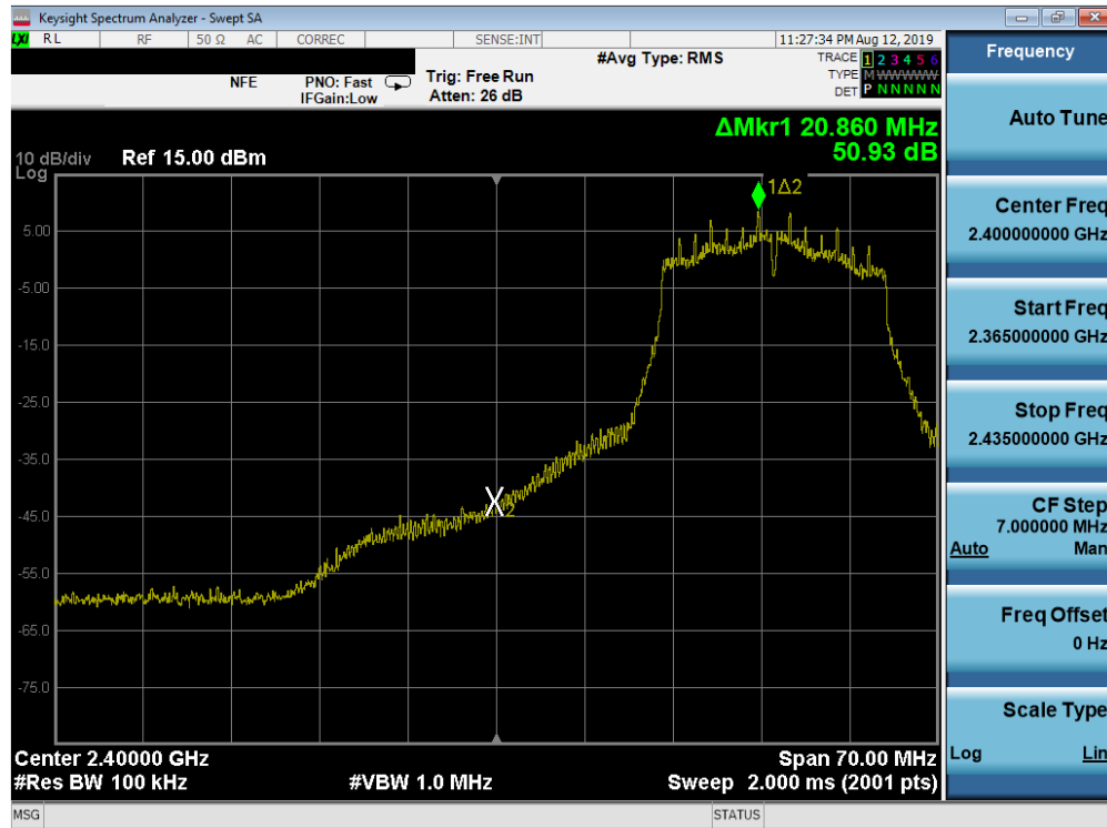
Plot 7-53. Band Edge Plot SISO ANT1 (802.11n (2.4GHz) – Ch. 3)
