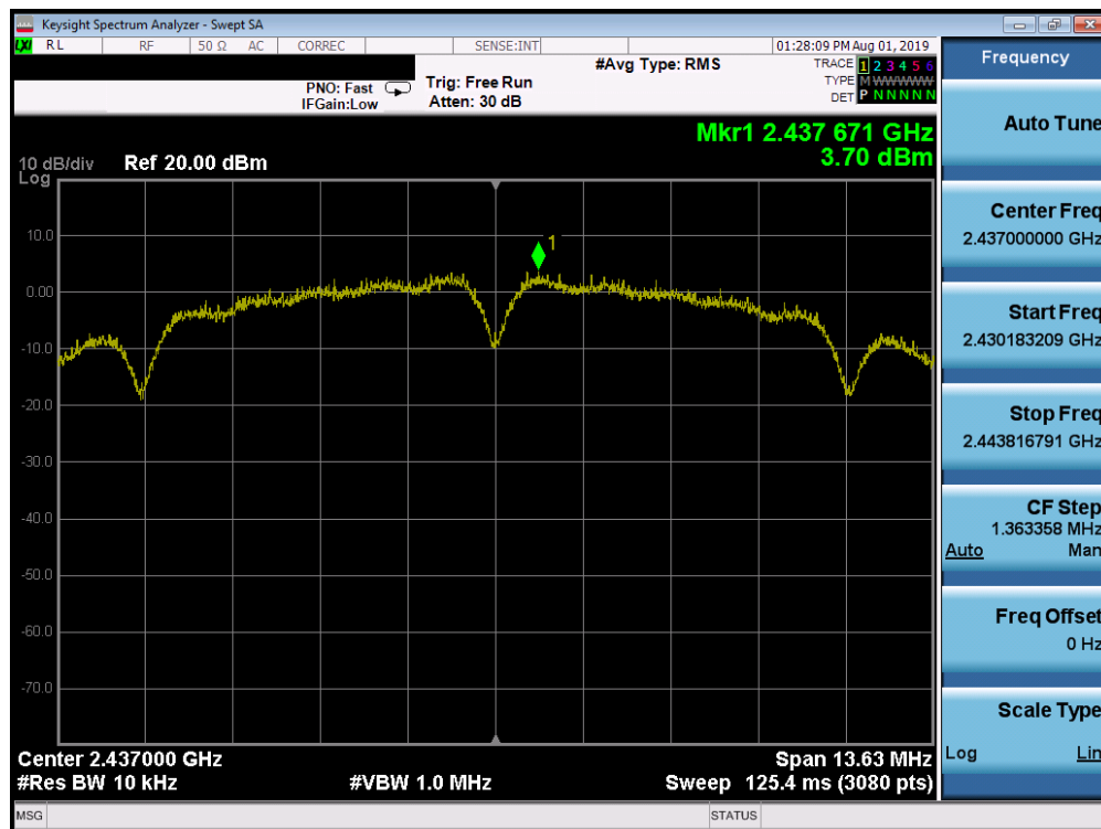
Plot 7-35. Power Spectral Density Plot SISO ANT2 (802.11b – Ch. 6)
