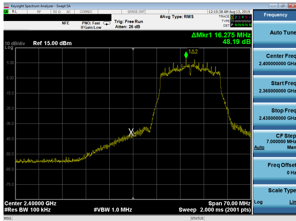
Plot 7-66. Band Edge Plot SISO ANT2 (802.11n (2.4GHz) – Ch. 2)
