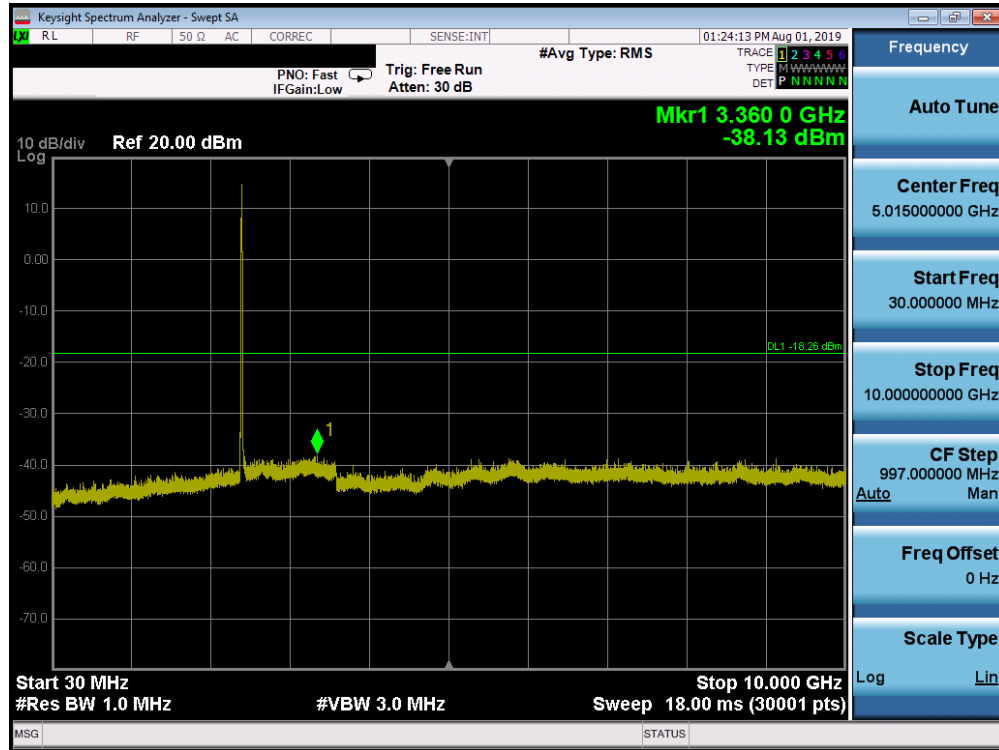
Plot 7-83. Conducted Spurious Plot SISO ANT2 (802.11b – Ch. 1)
