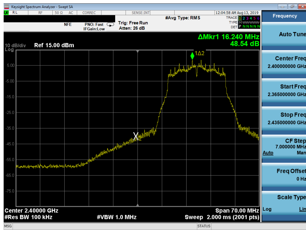
Plot 7-60. Band Edge Plot SISO ANT2 (802.11g- Ch. 2)
