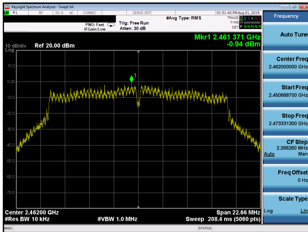
Plot 7-39. Power Spectral Density Plot SISO ANT2 (802.11g – Ch. 11)
