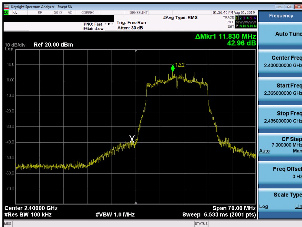
Plot 7-65. Band Edge Plot SISO ANT2 (802.11n (2.4GHz) – Ch. 1)
