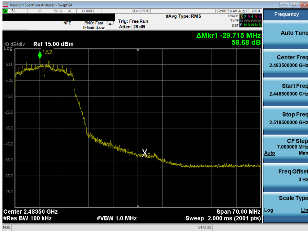
Plot 7-63. Band Edge Plot SISO ANT2 (802.11g– Ch. 10)
