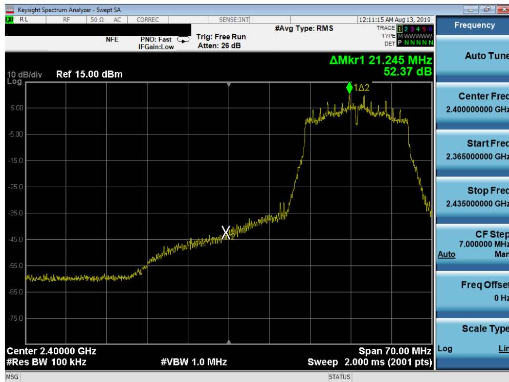
Plot 7-67. Band Edge Plot SISO ANT2 (802.11n (2.4GHz) – Ch. 3)
