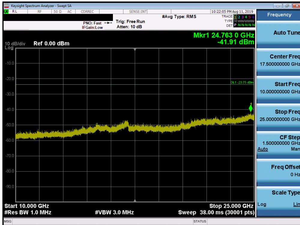
Plot 7-82. Conducted Spurious Plot SISO ANT1 (802.11ac – Ch. 11)
