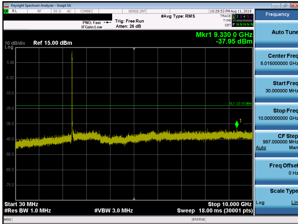
Plot 7-89. Conducted Spurious Plot SISO ANT2 (802.11ac – Ch. 1)
