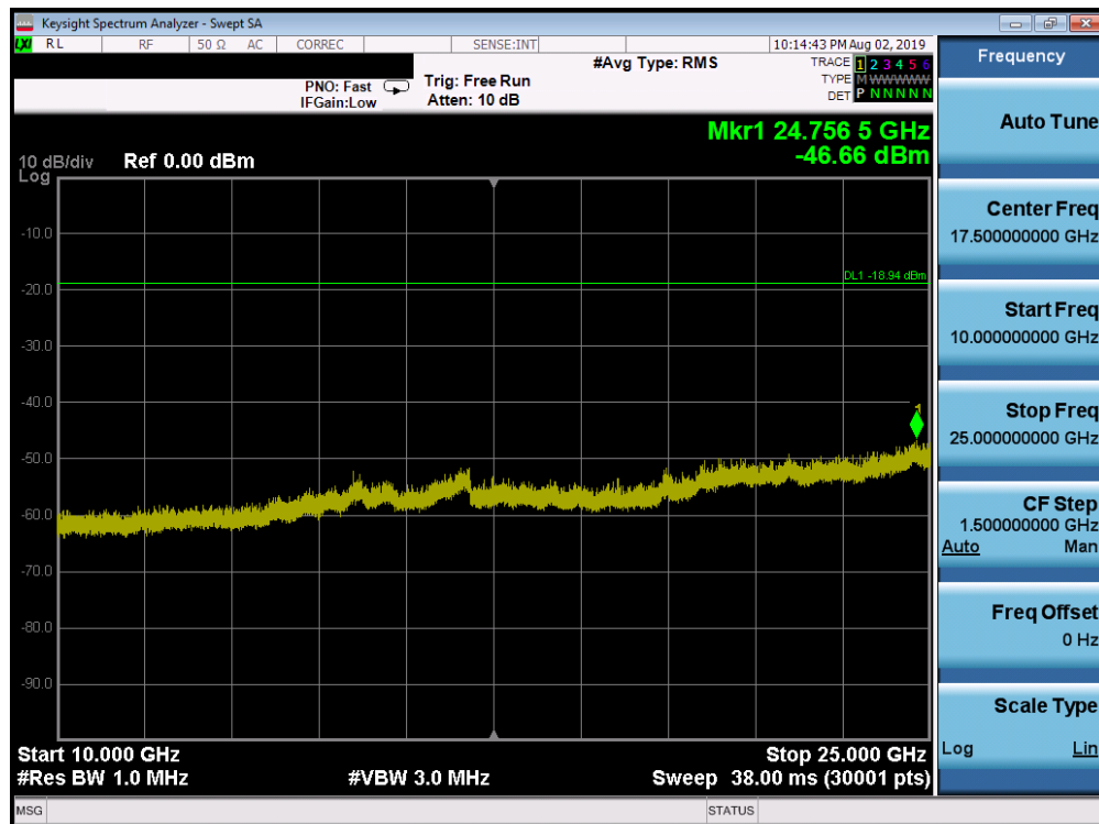
Plot 7-76. Conducted Spurious Plot SISO ANT1 (802.11b – Ch. 11)
