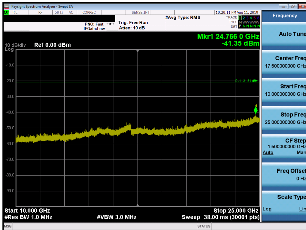
Plot 7-80. Conducted Spurious Plot SISO ANT1 (802.11ac – Ch. 6)
