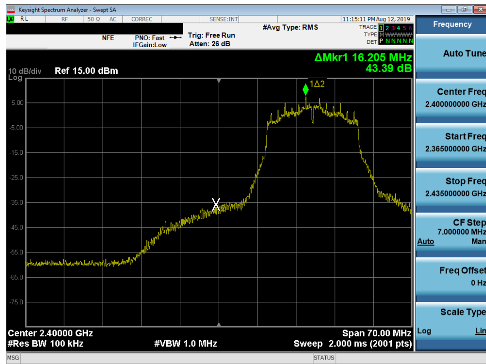
Plot 7-46. Band Edge Plot SISO ANT1 (802.11g- Ch. 2)
