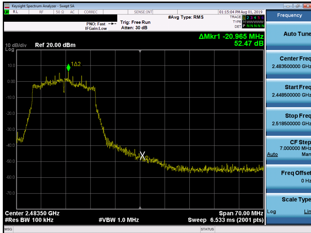
Plot 7-56. Band Edge Plot SISO ANT1 (802.11n (2.4GHz) – Ch. 11)
