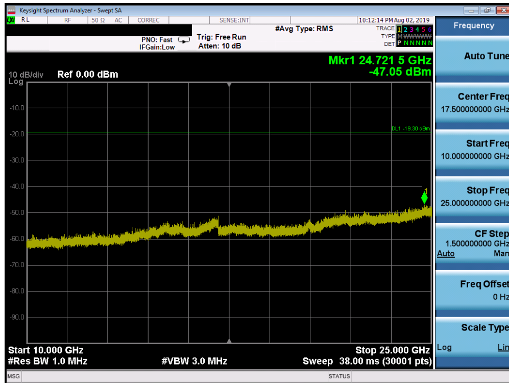
Plot 7-72. Conducted Spurious Plot SISO ANT1 (802.11b – Ch. 1)
