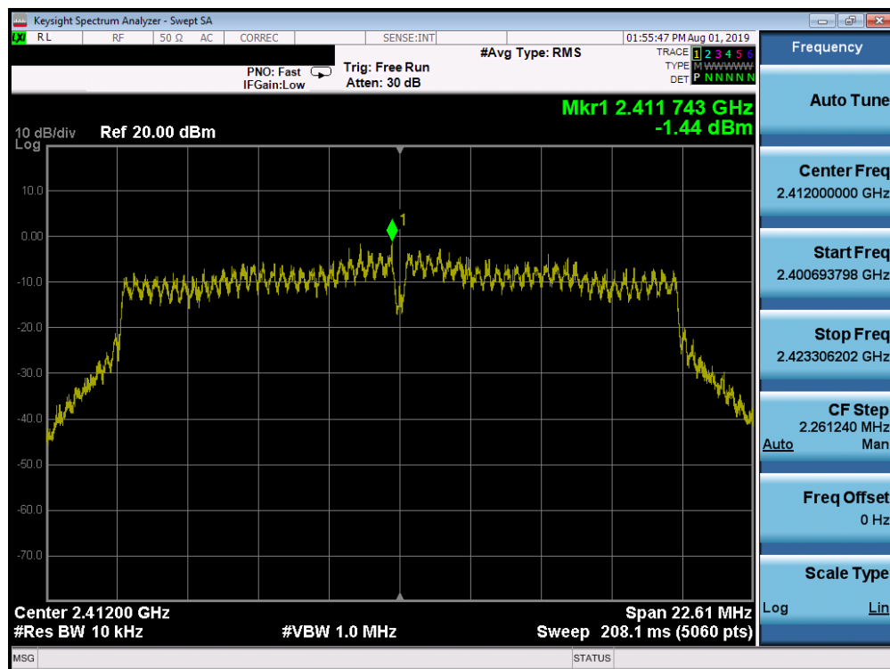
Plot 7-40. Power Spectral Density Plot SISO ANT2 (802.11n (2.4GHz) – Ch. 1)
