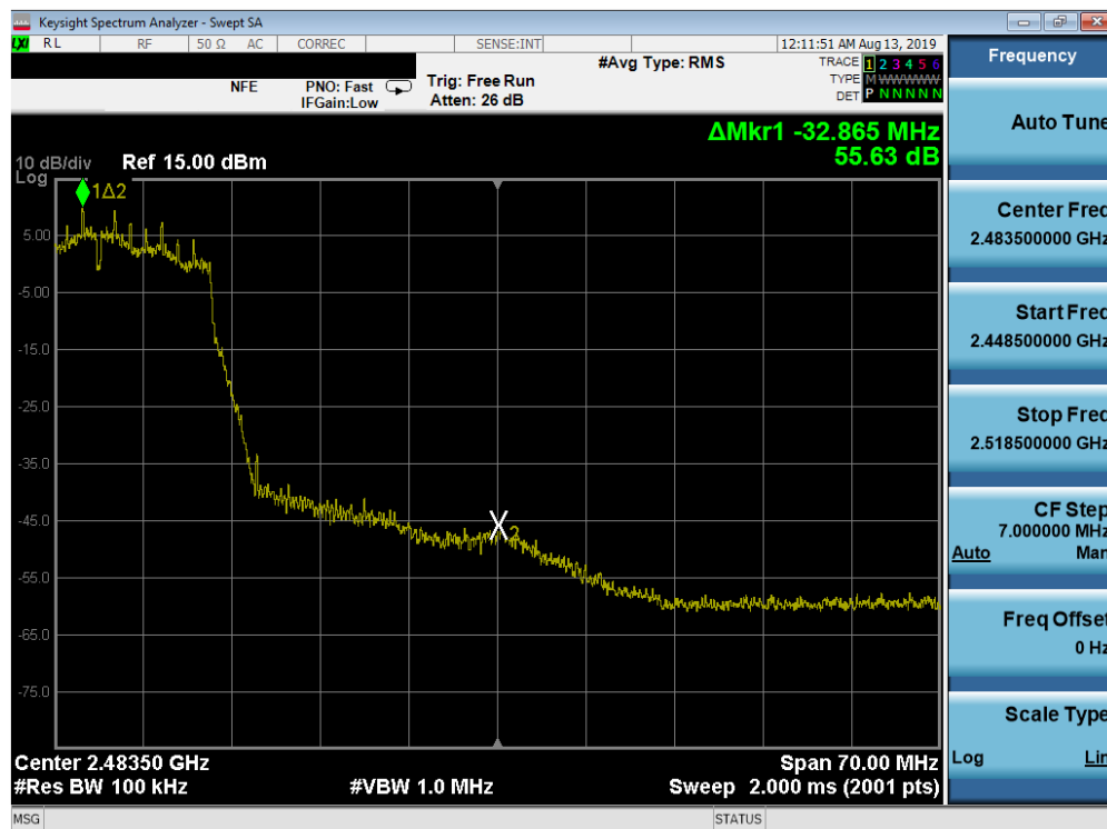
Plot 7-68. Band Edge Plot SISO ANT2 (802.11n (2.4GHz) – Ch. 9)
