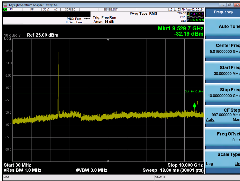
Plot 7-71. Conducted Spurious Plot SISO ANT1 (802.11b – Ch. 1)
