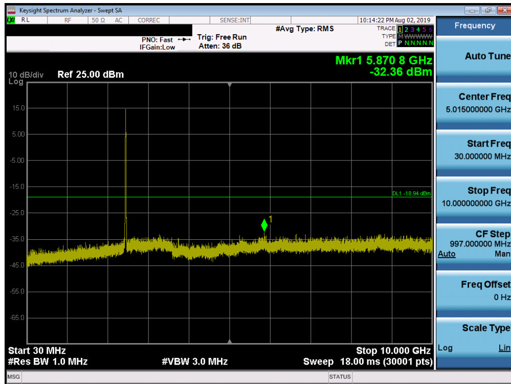
Plot 7-75. Conducted Spurious Plot SISO ANT1 (802.11b – Ch. 11)
