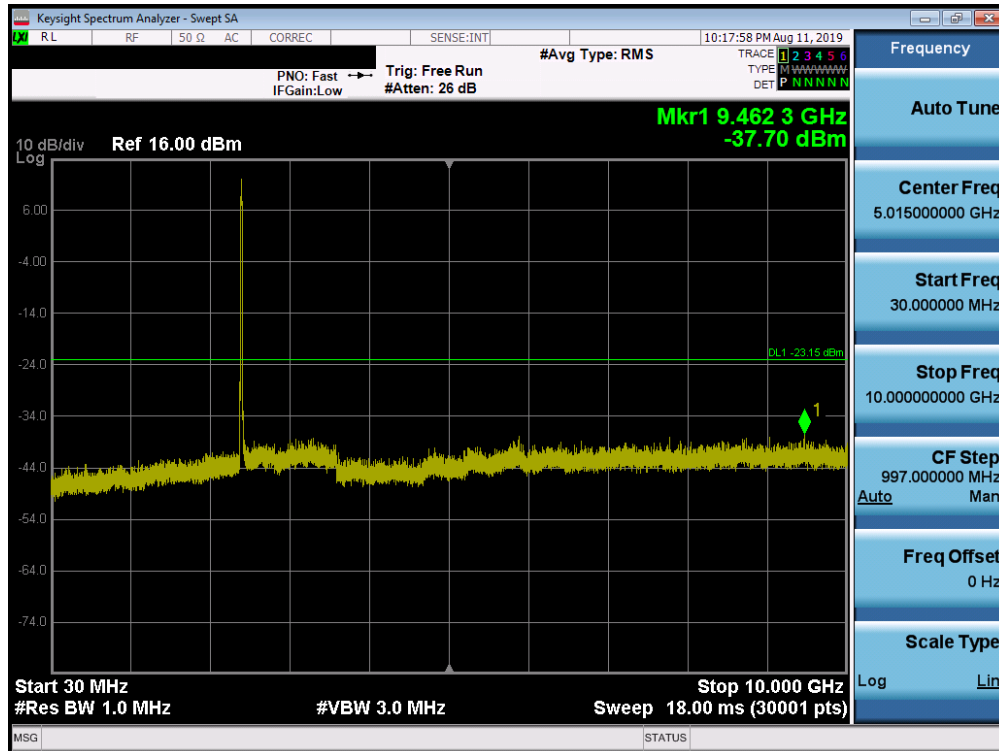
Plot 7-77. Conducted Spurious Plot SISO ANT1 (802.11ac – Ch. 1)
