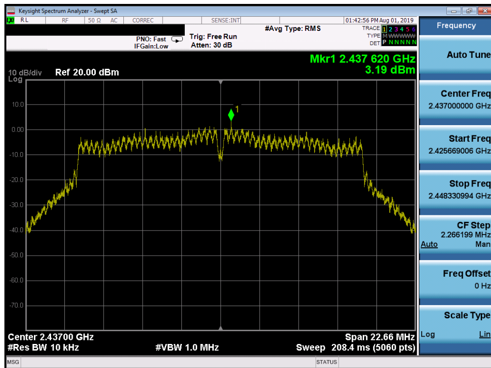
Plot 7-38. Power Spectral Density Plot SISO ANT2 (802.11g – Ch. 6)
