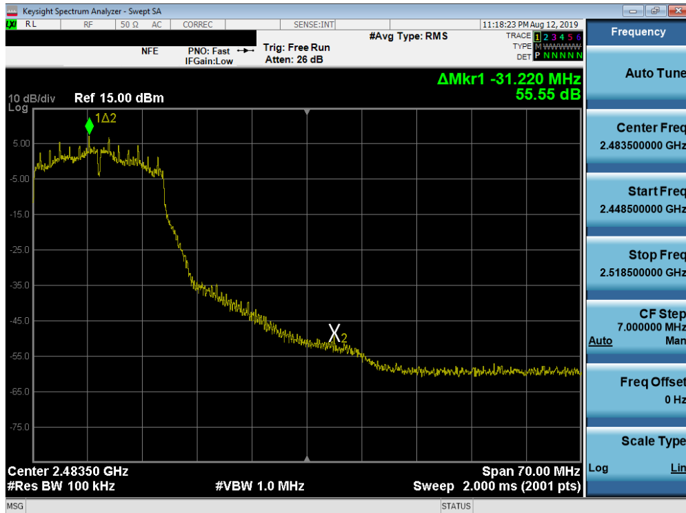
Plot 7-49. Band Edge Plot SISO ANT1 (802.11g– Ch. 10)
