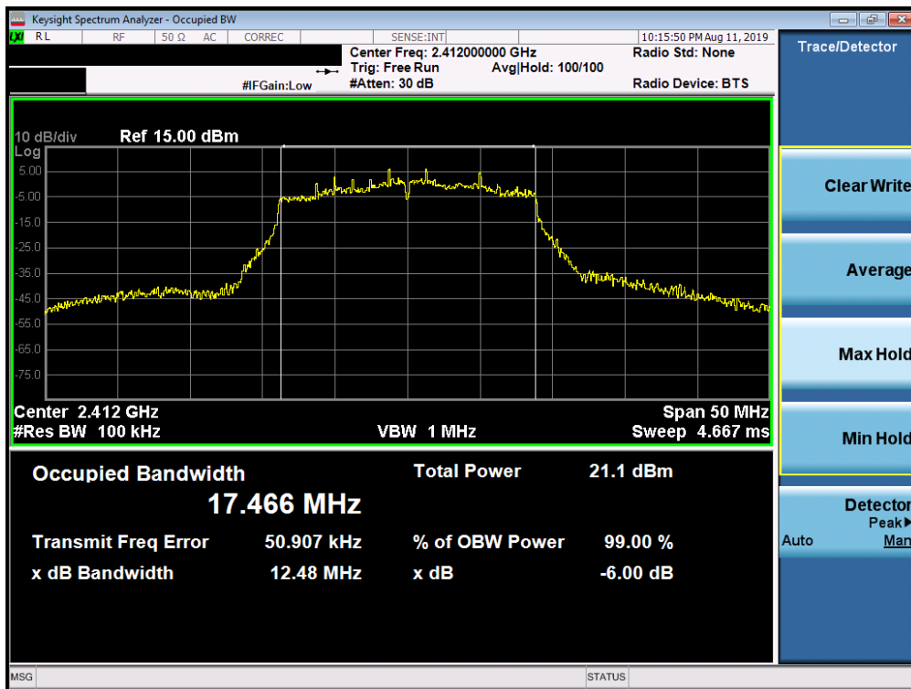
Plot 7-10. 6dB Bandwidth Plot SISO ANT1 (802.11ac) (2.4GHz) – Ch. 1)
