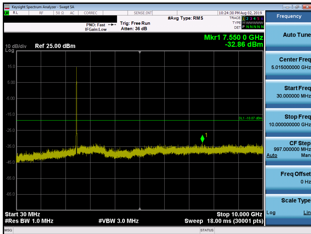
Plot 7-87. Conducted Spurious Plot SISO ANT2 (802.11b – Ch. 11)
