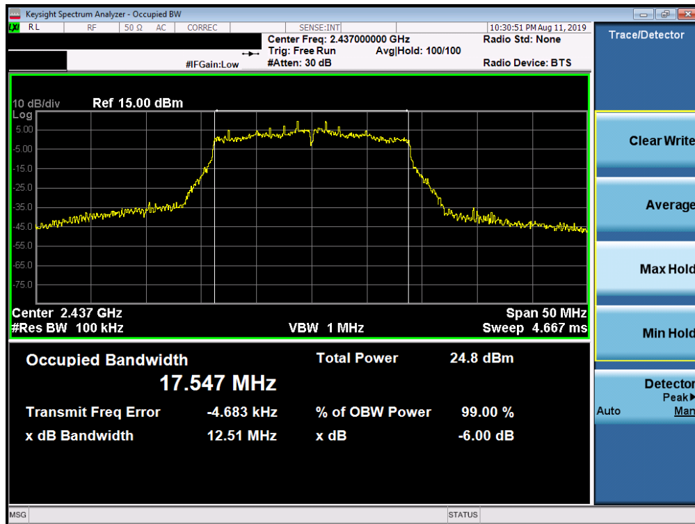
Plot 7-23. 6dB Bandwidth Plot SISO ANT2 (802.11ac (2.4GHz) – Ch. 6)
