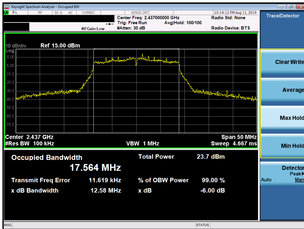
Plot 7-11. 6dB Bandwidth Plot SISO ANT1 (802.11ac (2.4GHz) – Ch. 6)
