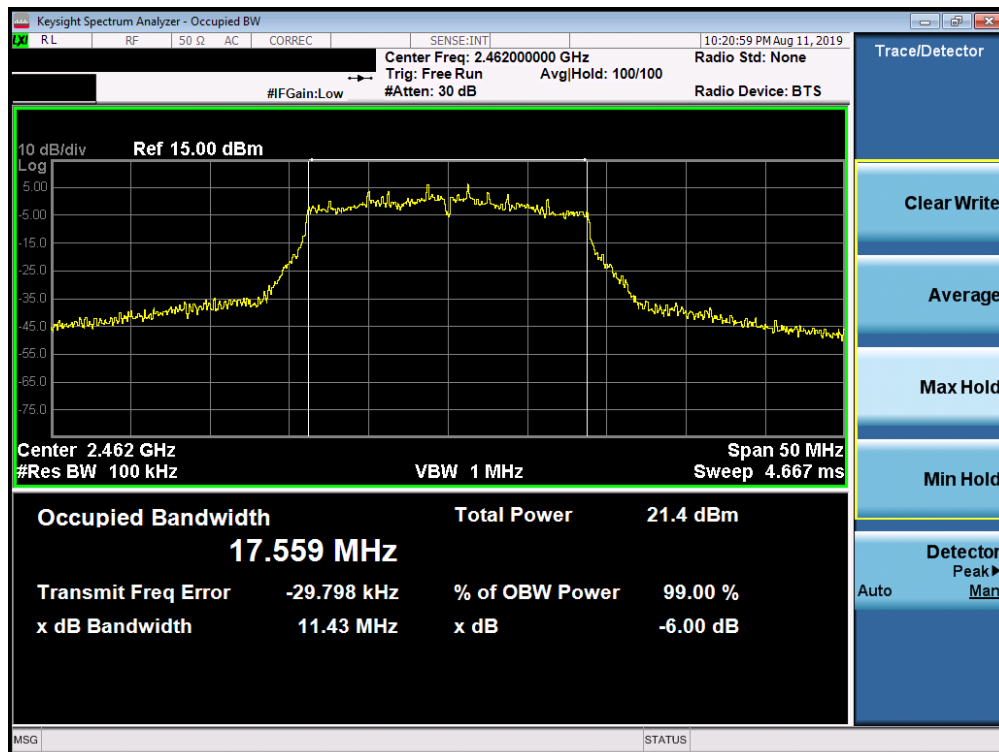
Plot 7-12. 6dB Bandwidth Plot SISO ANT1 (802.11ac (2.4GHz) – Ch. 11)
