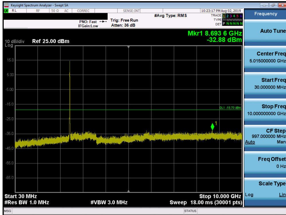
Plot 7-85. Conducted Spurious Plot SISO ANT2 (802.11b – Ch. 6)
