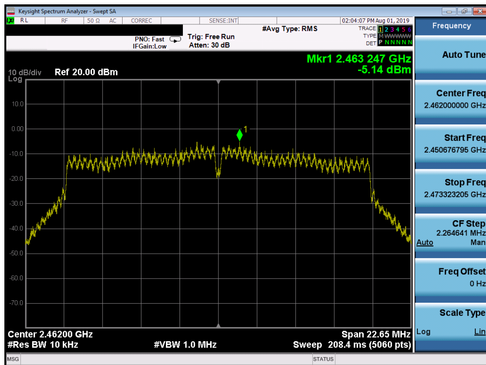
Plot 7-42. Power Spectral Density Plot SISO ANT2 (802.11n (2.4GHz) – Ch. 11)
