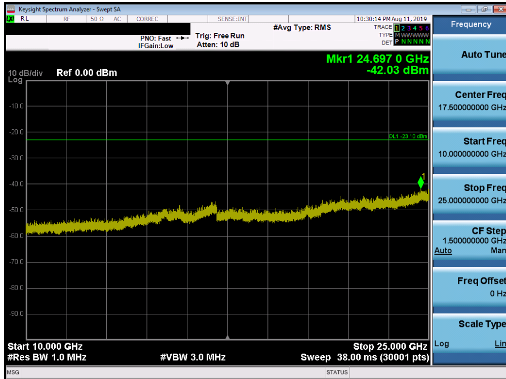
Plot 7-90. Conducted Spurious Plot SISO ANT2 (802.11ac – Ch. 1)
