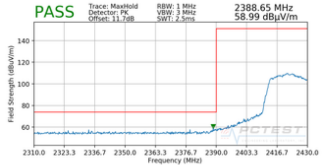
Plot 7-109. Radiated Restricted Lower Band Edge Measurement SISO ANT1 (Peak)
