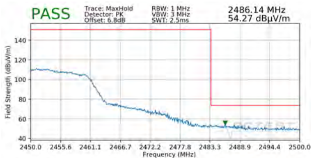
Plot 7-56. Radiated Restricted Upper Band Edge Measurement MIMO (Peak)
