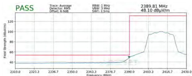
Plot 7-49. Radiated Restricted Lower Band Edge Measurement MIMO (Average)
