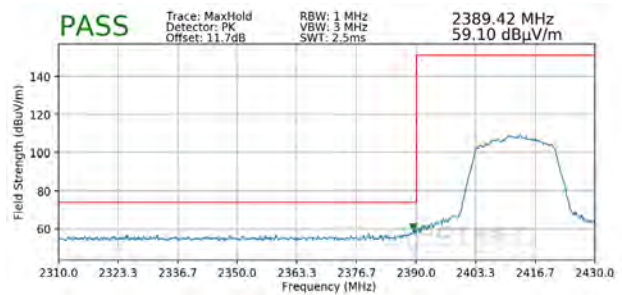
Plot 7-44. Radiated Restricted Band Edge Measurement SISO ANT2 with WCP (Peak)
