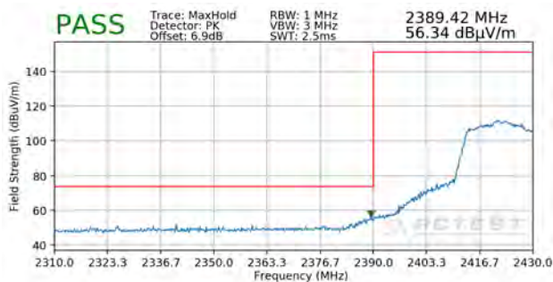
Plot 7-54. Radiated Restricted Lower Band Edge Measurement MIMO (Peak)
