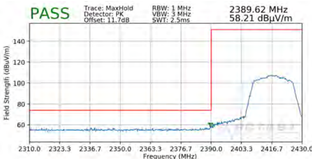
Plot 7-16. Radiated Restricted Lower Band Edge Measurement SISO ANT1 (Peak)
