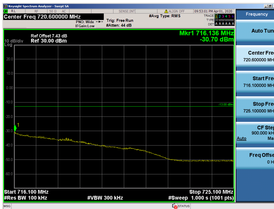
LTE Band 12, 17 / 10MHz / 16QAM - RB Size/Offset (25/25)
