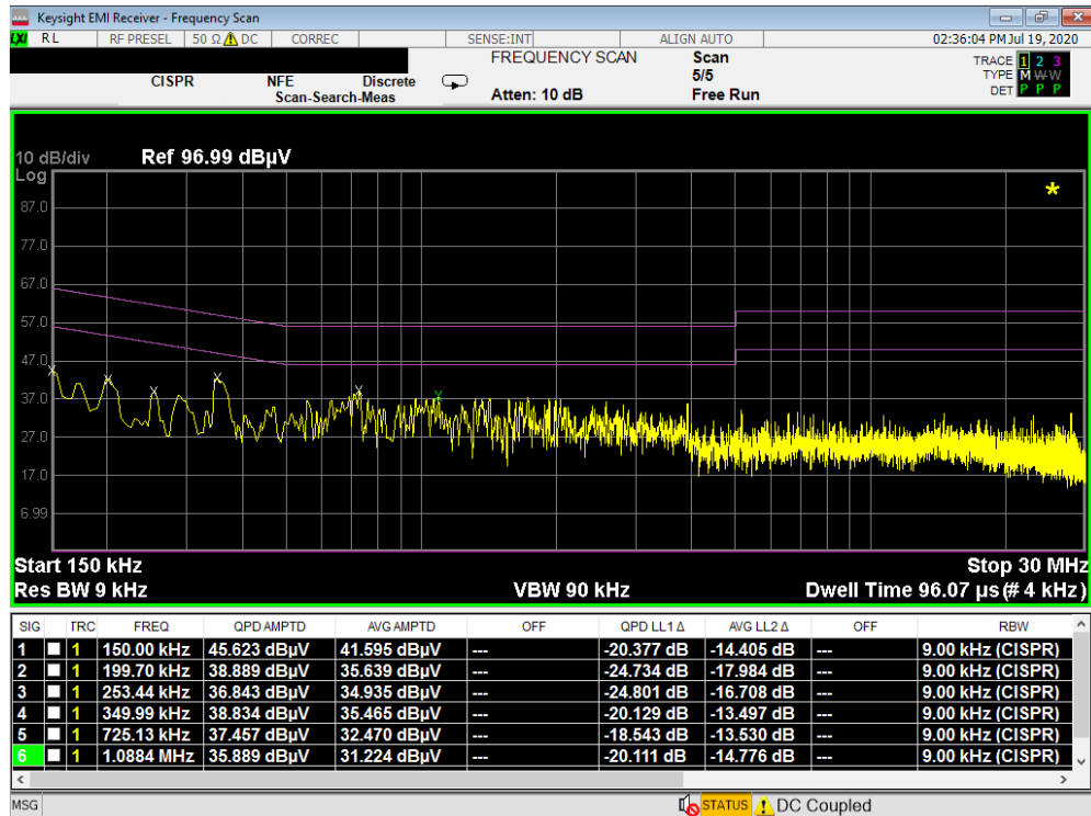
Plot 7-57. Line Conducted Plot with Bluetooth LE (L1) with WCP
