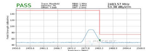
Plot 7-54. Radiated Restricted Upper Band Edge Measurement with WCP (Peak)
