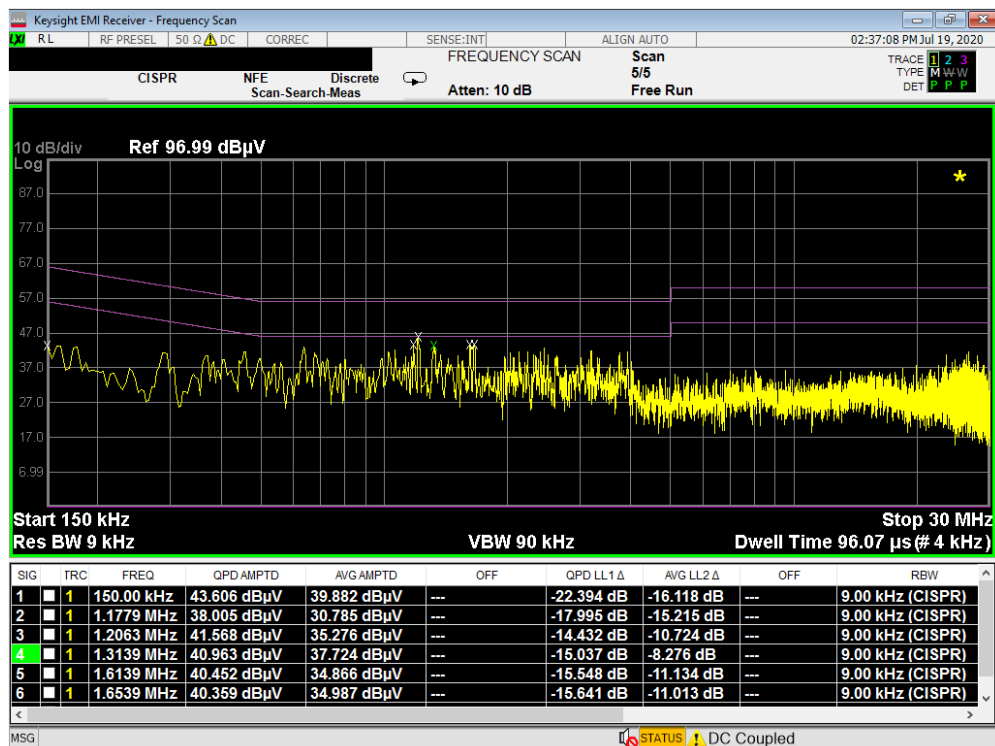
Plot 7-58. Line Conducted Plot with Bluetooth LE (N) with WCP
