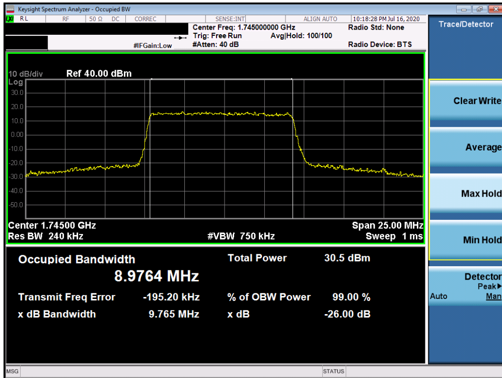
Plot 7-117. Occupied Bandwidth Plot (n66 10MHz 64QAM-CP-OFDM- Full RB Configuration)
