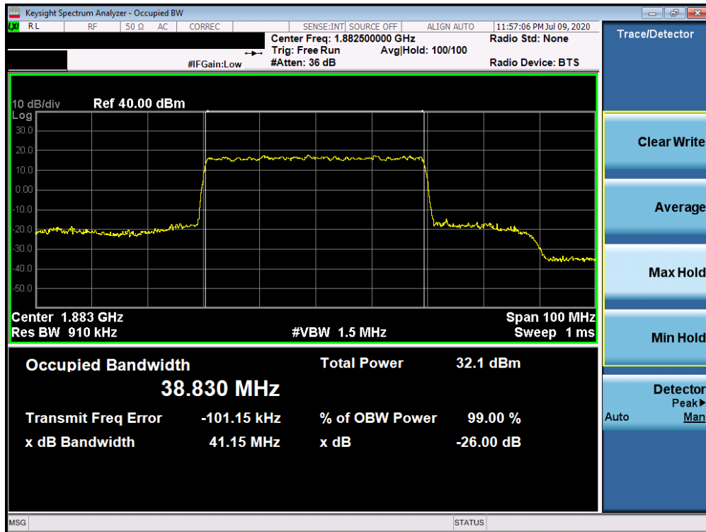
Plot 7-178. Occupied Bandwidth Plot (n25 40MHz 16QAM-CP-OFDM - Full RB Configuration)
