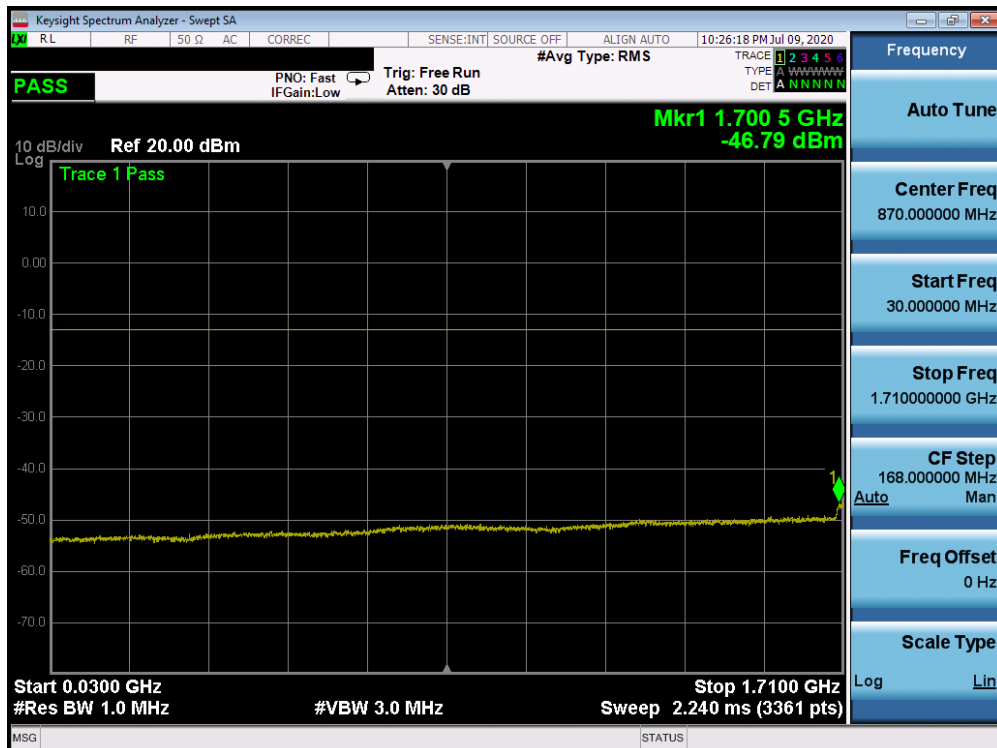
Plot 7-314. Conducted Spurious Plot (n66 - 20MHz DFT-s-OFDM-QPSK - RB Size 1, RB Offset 1 - Mid Channel)
