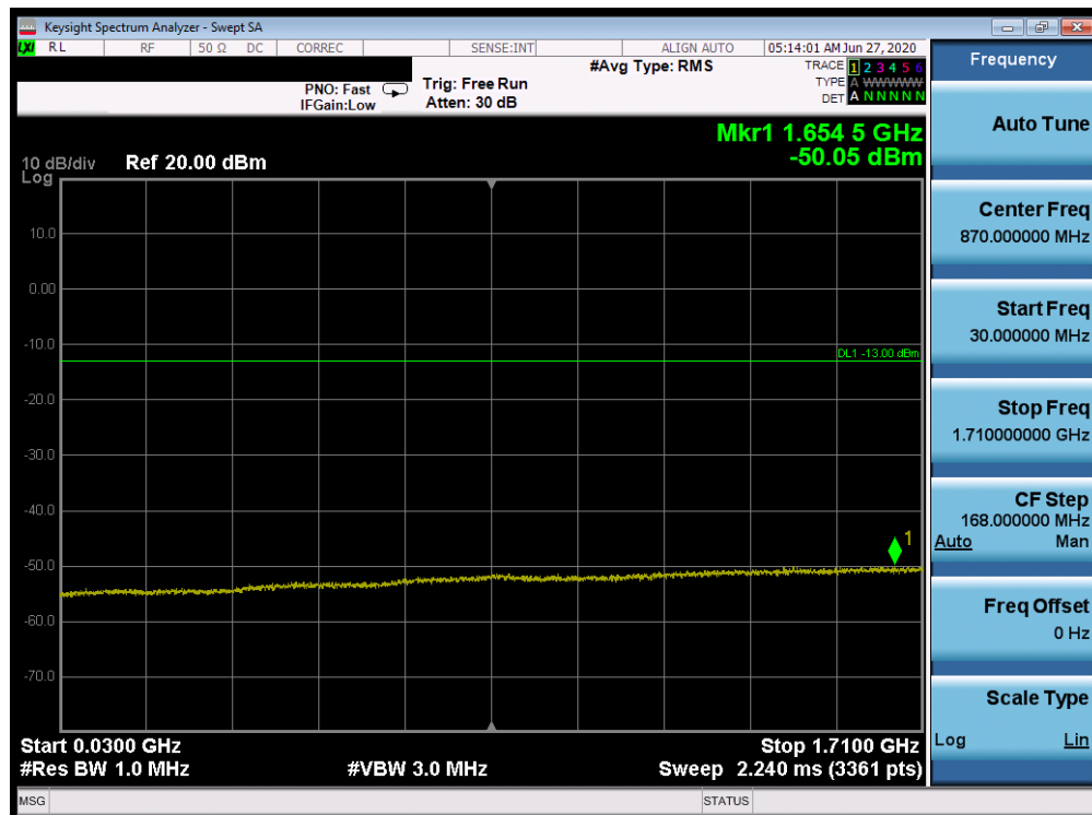
Plot 7-305. Conducted Spurious Plot (Band 66/4 - 20.0MHz QPSK - RB Size 1, RB Offset 0 - Mid Channel)
